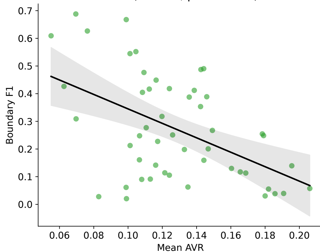
Pooled ( r=-0.42 , p=6.25e-08 )
