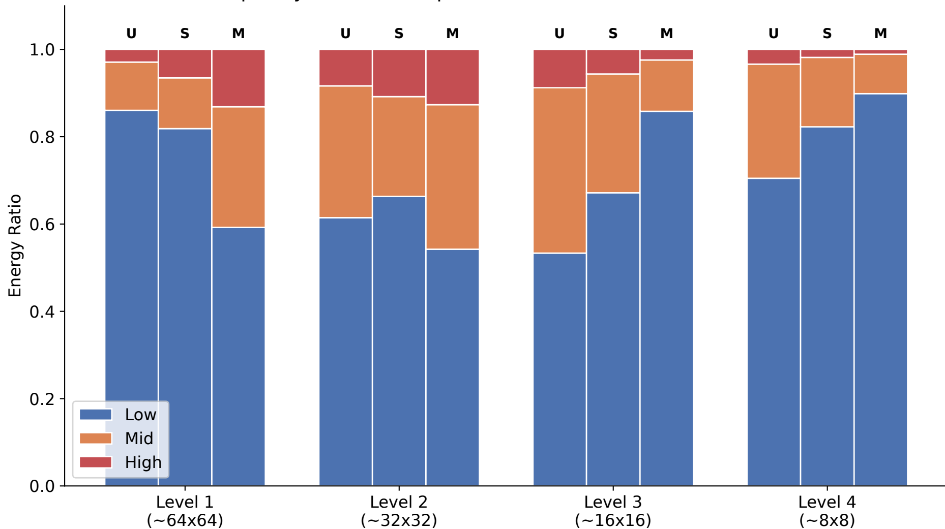
Frequency Band Decomposition (U: UNet, S: Swin, M: Mamba)
