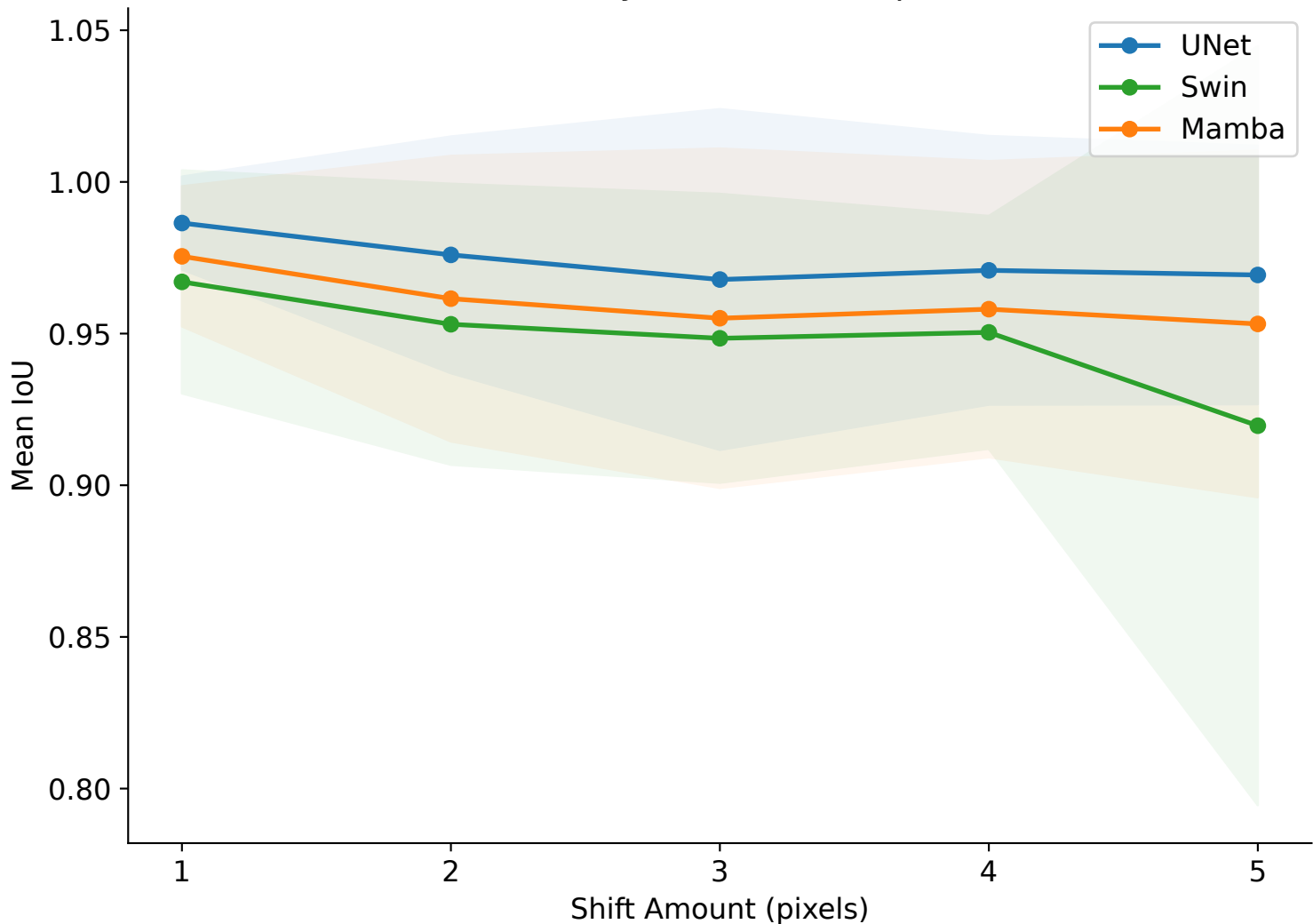
Shift Consistency (Translation Equivariance)
