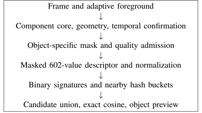
Fig. 1. The visual path from observation formation to retrieval. Hash tables contain exemplar references; full descriptors remain available for verification.
