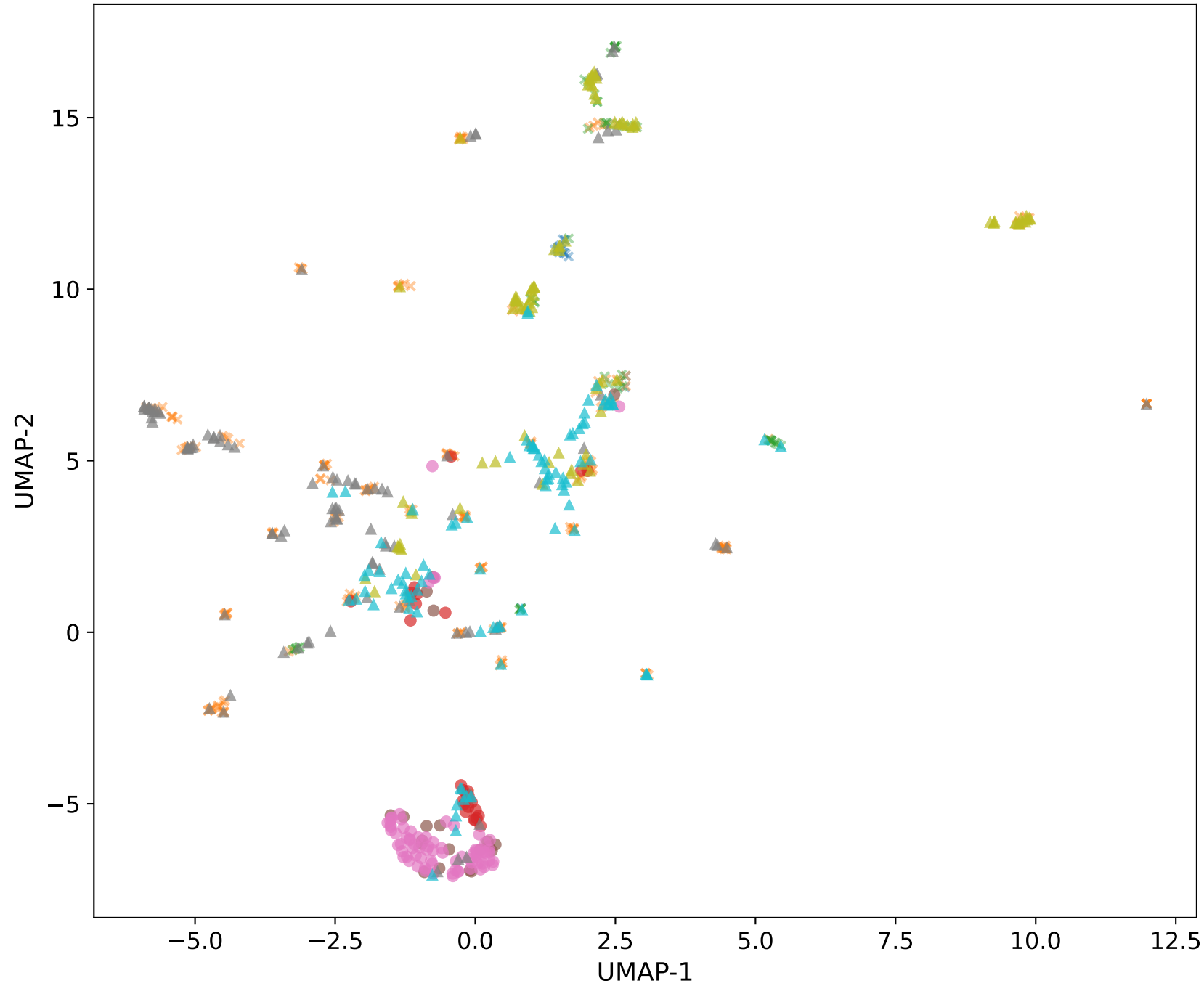
Raw ESM-2 Embeddings (Pretrained)
