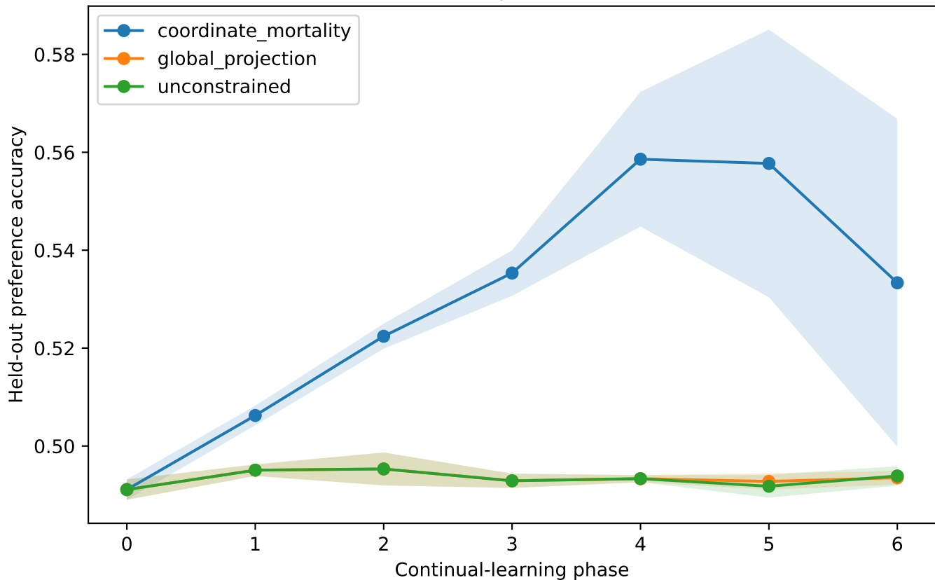
Qwen3-8B | conflict shift
