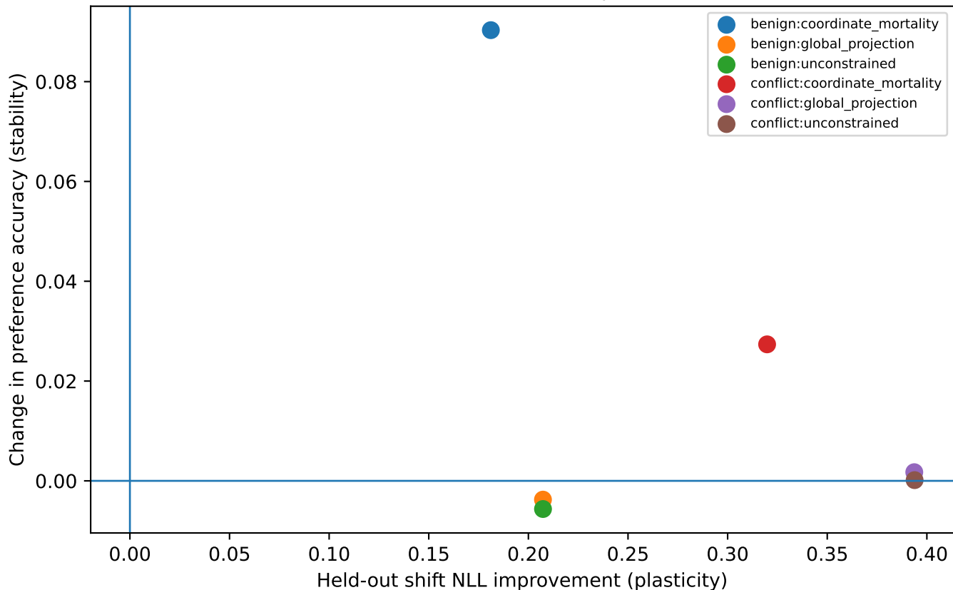
Stability-plasticity frontier | Qwen3-14B
