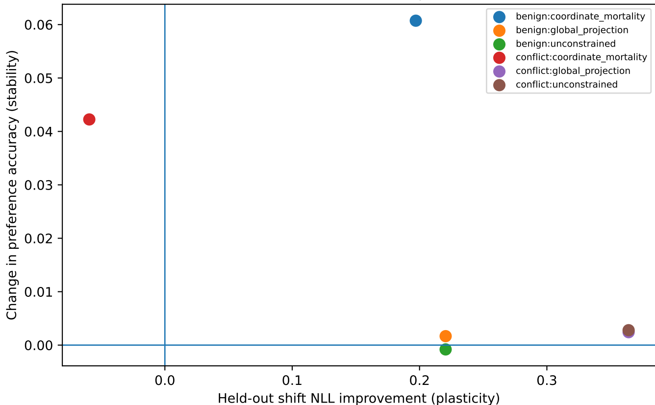
Stability-plasticity frontier | Qwen3-8B
