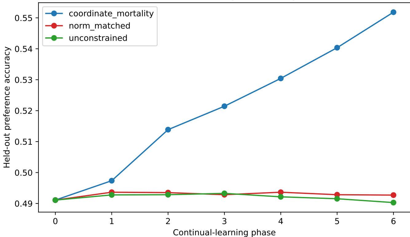
Norm-matched control | Qwen3-8B | benign
