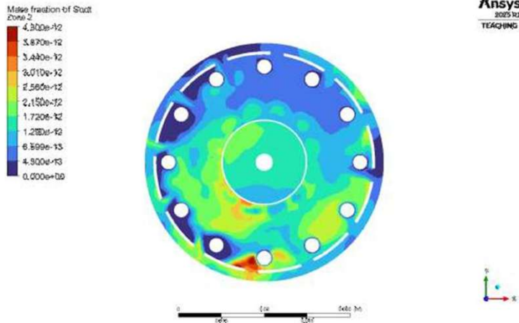
4.1.6.3(c) Zone 2 Soot mass fraction
