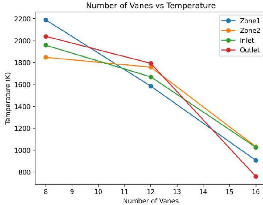
Fig.4.2.3 Number of Vanes vs Temperature (K)
