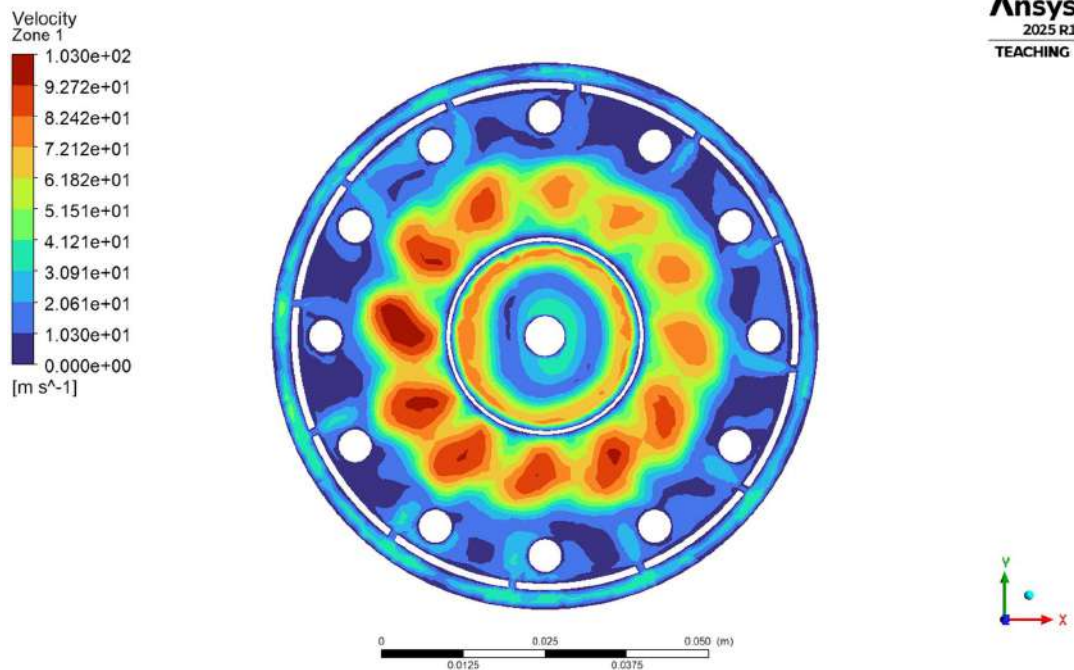
Fig.4.1.2.2(b) Zone 1 velocity Contour
