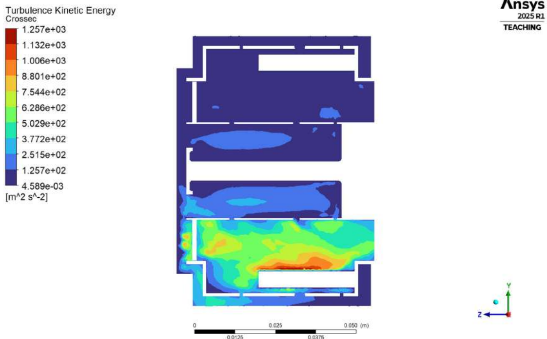
4.1.4.3(f) Cross-Section Turbulence Kinetic Energy
