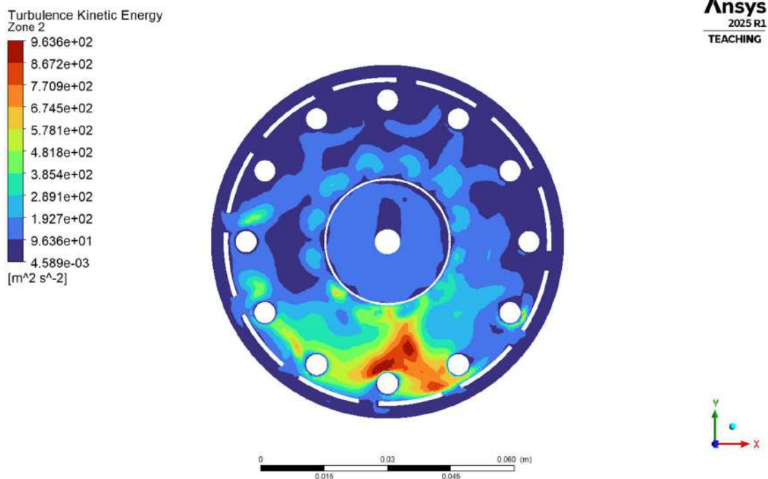
4.1.4.3(c) Zone 2 Turbulence Kinetic Energy
