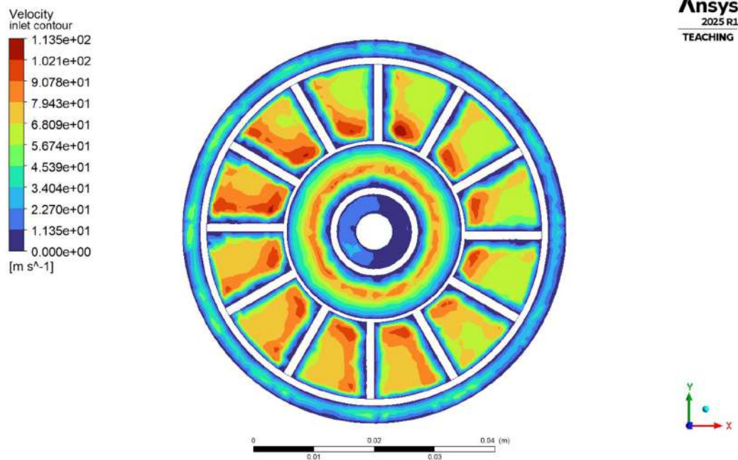
Fig.4.1.2.2(a) Inlet velocity Contour
