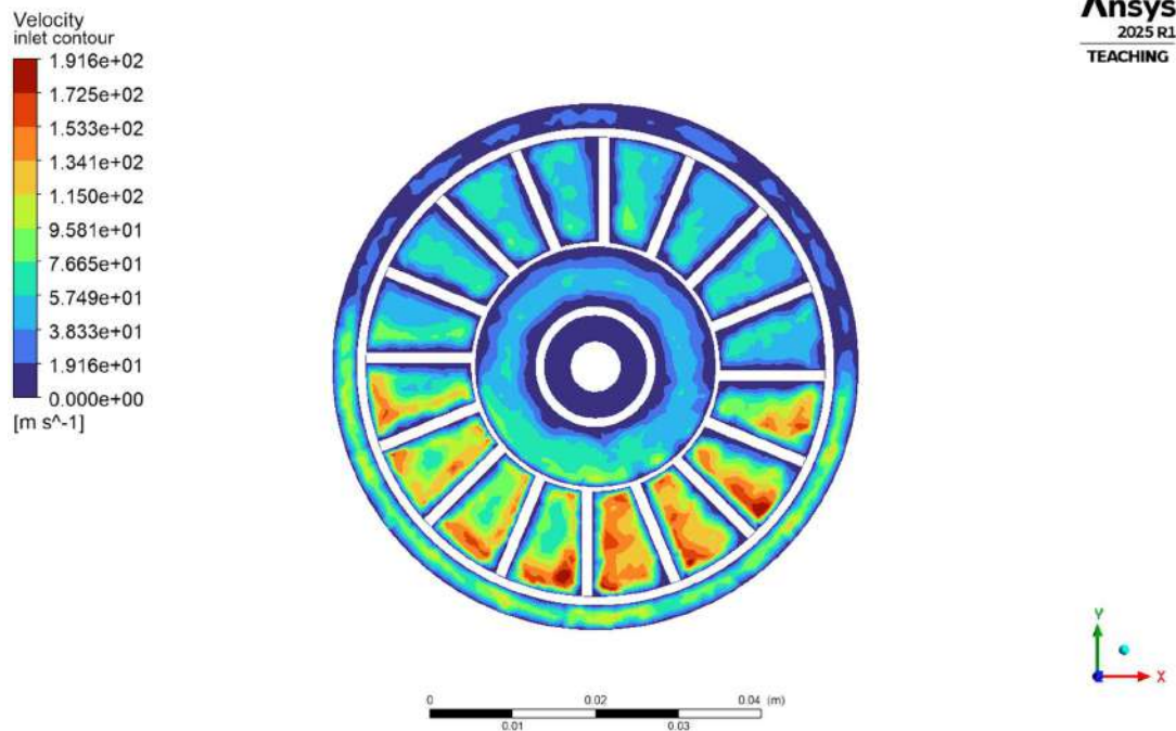
Fig.4.1.2.3(a) Inlet velocity Contour
