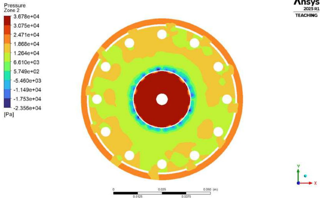
Fig.4.1.1.2(c) Zone 2 Pressure Contour
