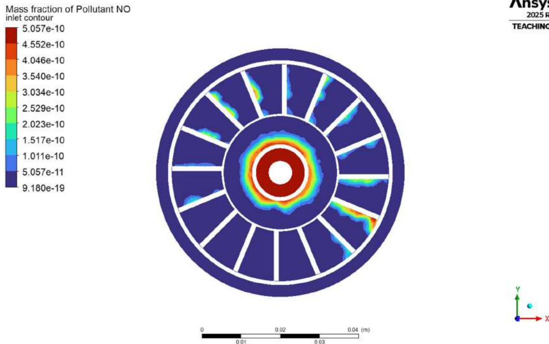
4.1.5.3(a) Inlet NO mass fraction
