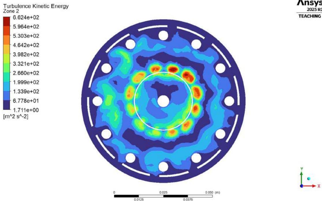
4.1.4.2(c): Zone 2 Turbulence Kinetic Energy
