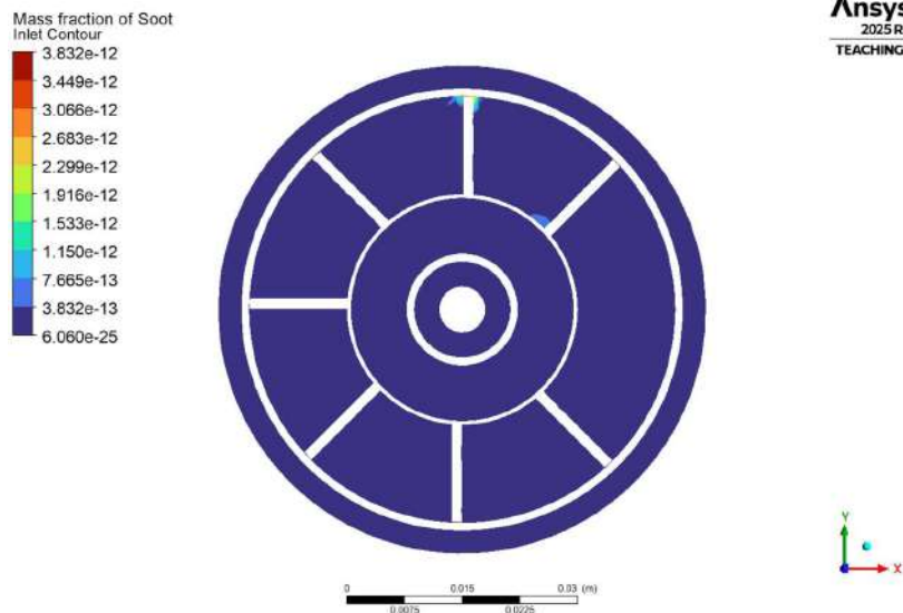
4.1.6.1(a) Inlet Soot mass fraction
