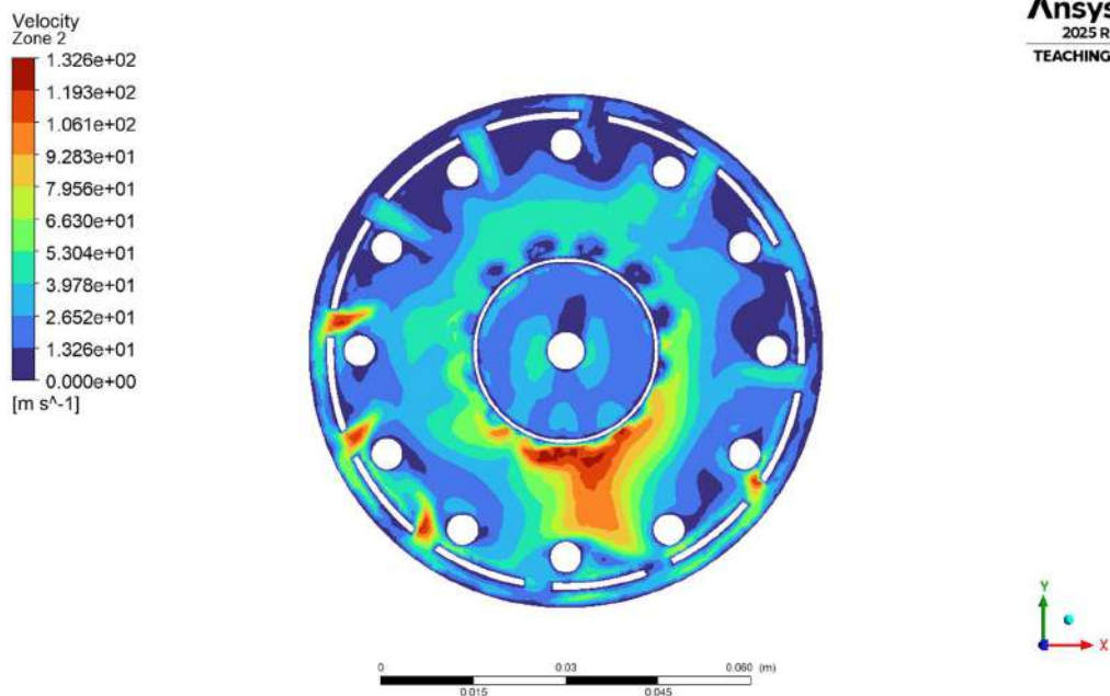
Fig.4.1.2.3(c) Zone 2 velocity Contour
