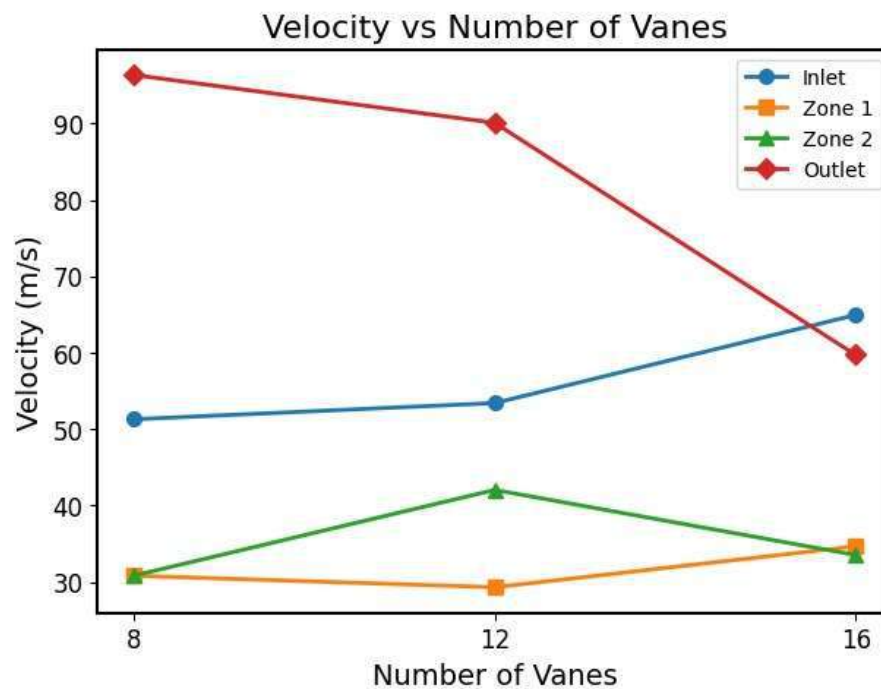
Fig.4.2.1 Number of Vanes vs Velocity (m/s)
