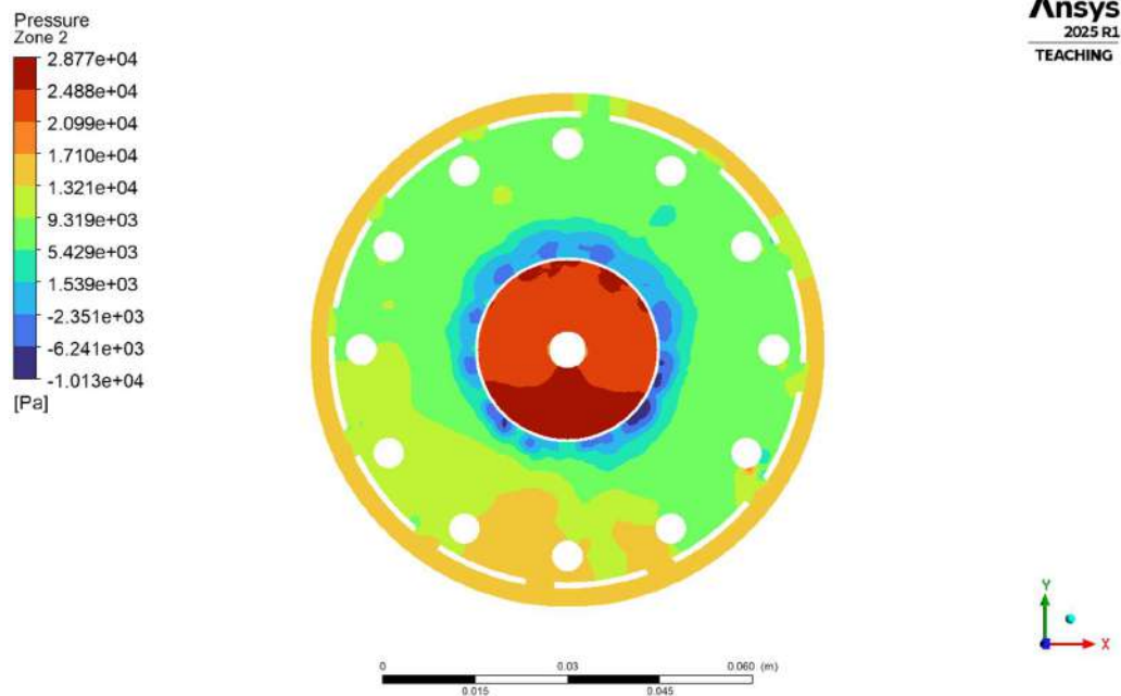
Fig.4.1.1.3(c)Zone 2 Pressure Contour
