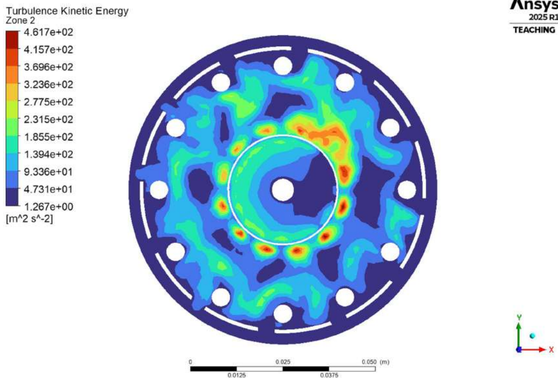
4.1.4.1(c) Zone 2 Turbulent Kinetic Energy
