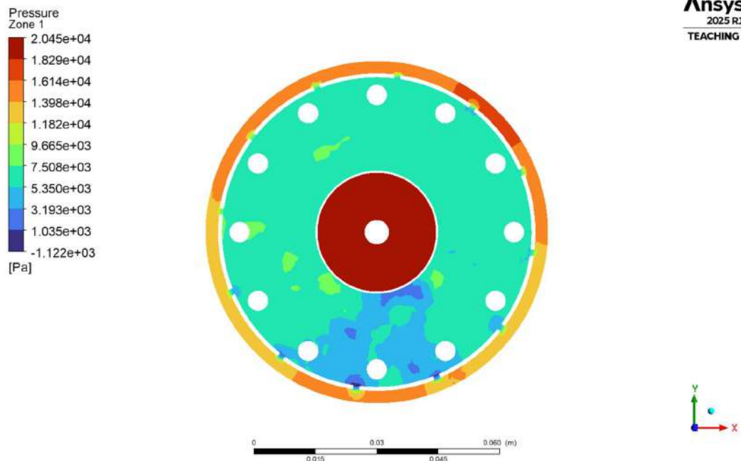
Fig.4.1.1.3(b) zone 1 Pressure Contour
