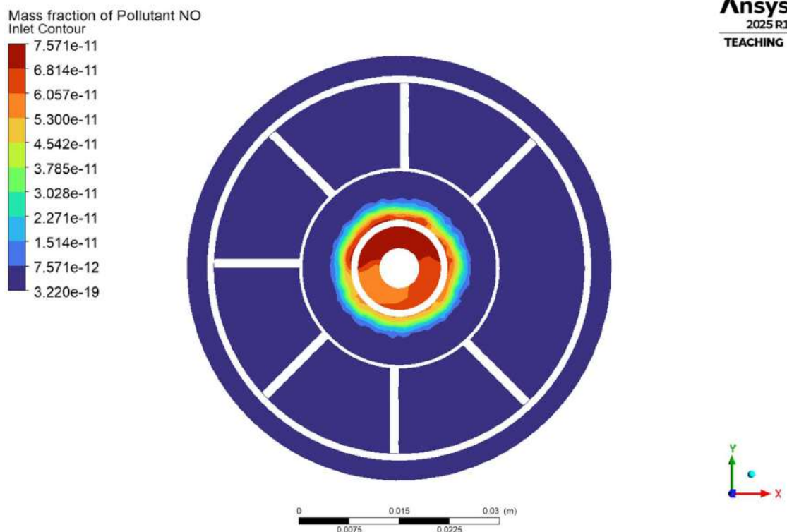
4.1.5.1(a) Mass Fraction of \text{No}_x Inlet Contour
