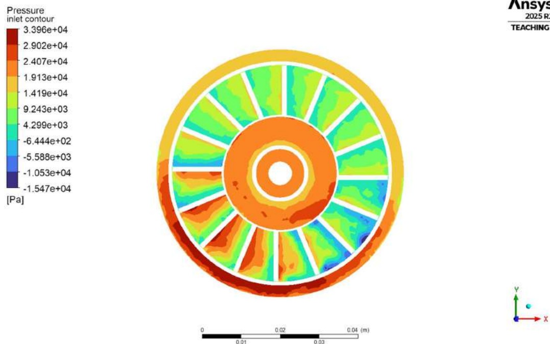
Fig.4.1.1.3(a) Inlet Pressure Contour
