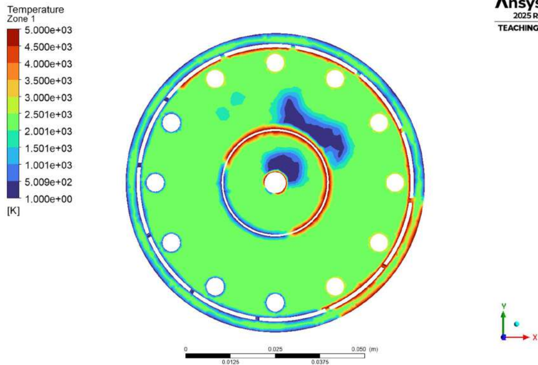
4.1.3.1(b) Zone 1 Temperature Contour
