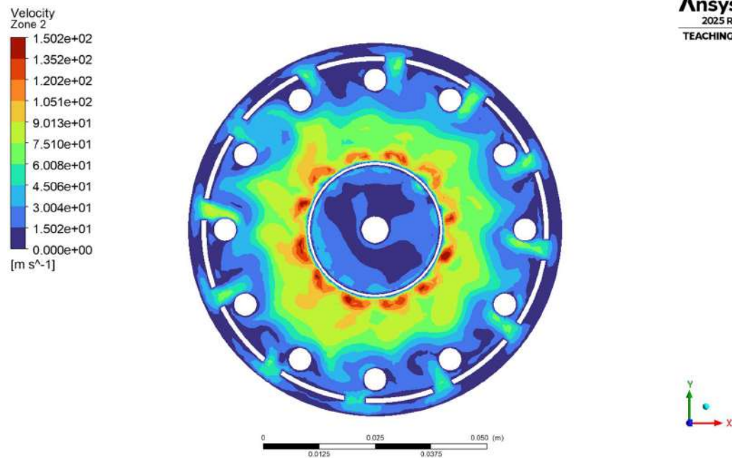
Fig.4.1.2.2(c) Zone 2 velocity Contour
