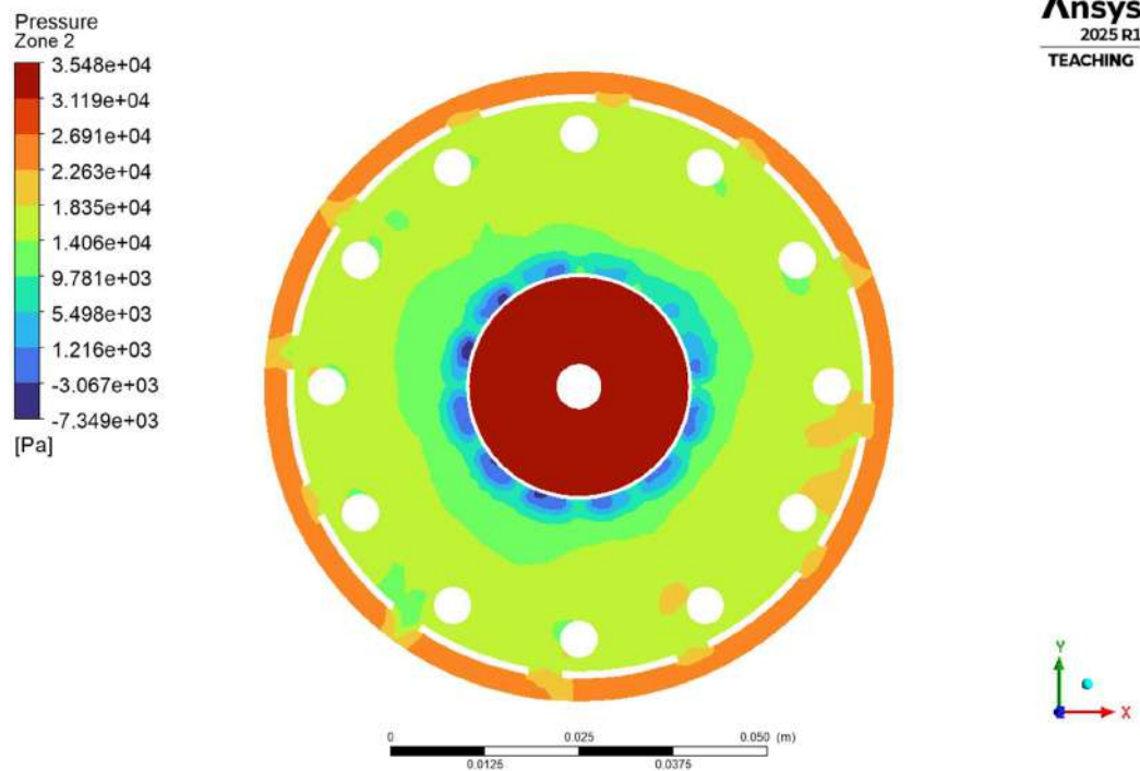
Fig.4.1.1.1(c) Zone 2 Pressure Contour.
