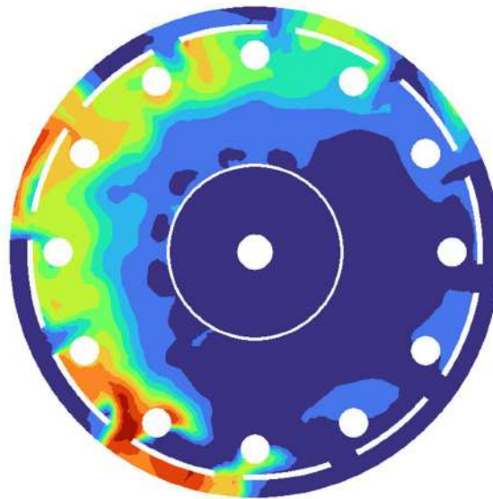
4.1.5.2(c) Zone 2 NO mass fraction
