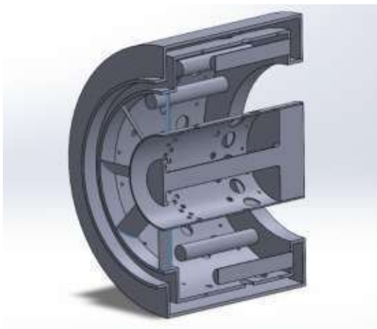
Fig.3.2(a) 8 blade swirler with combustor Cross-sectional view
