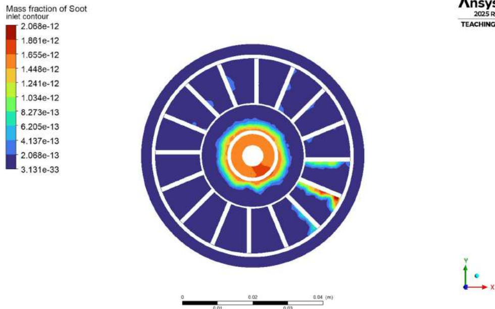
4.1.6.3(a) Inlet Soot mass fraction
