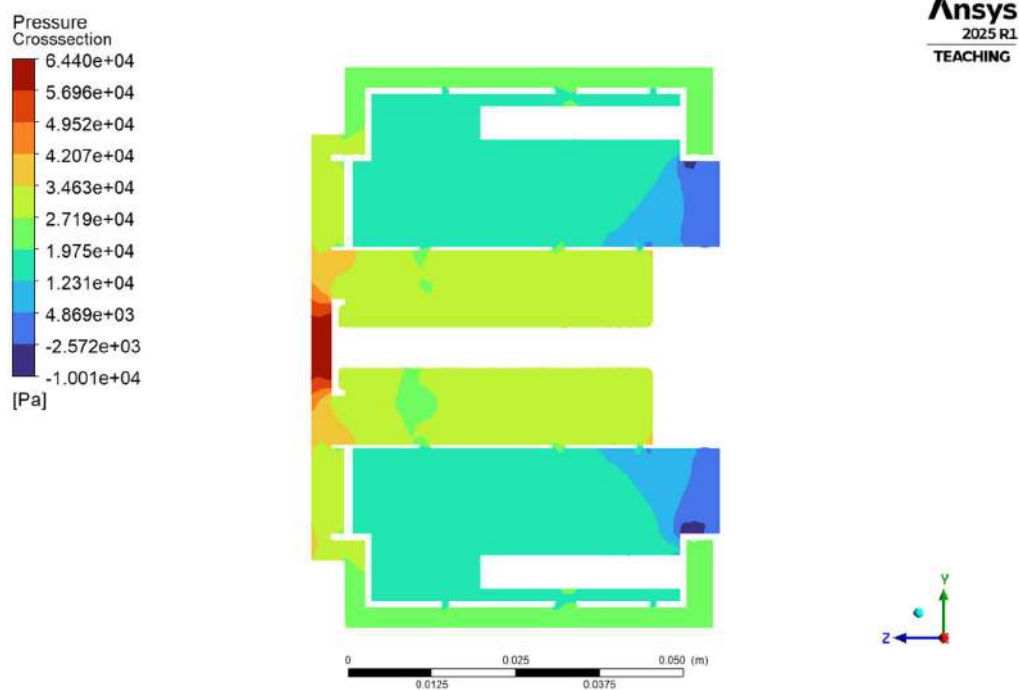
Fig.4.1.1.1(e) Cross-Section Pressure Contour.
