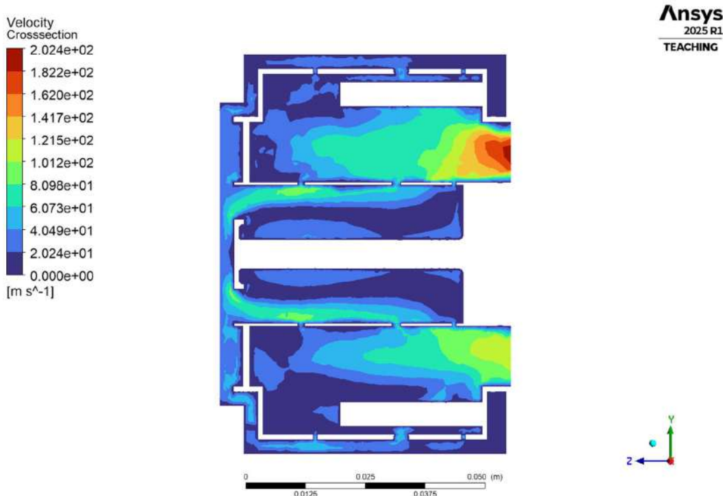
Fig.4.1.2.1(e) Cross-Section velocity Contour
