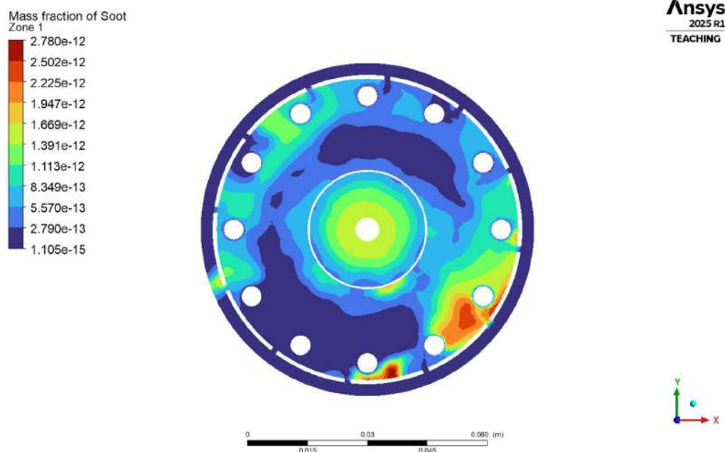
4.1.6.3(b) Zone 1 Soot mass fraction
