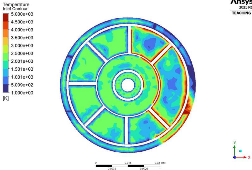
4.1.3.1(a) Inlet Temperature Contour
