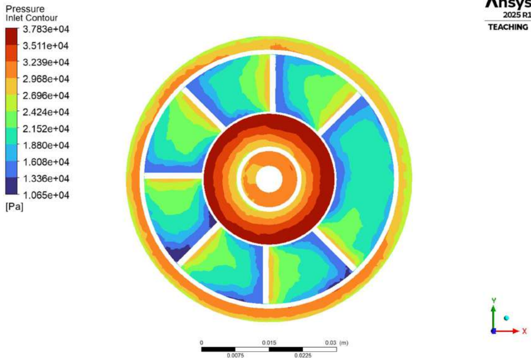
Fig.4.1.1.1(a) Inlet Pressure Contour.
