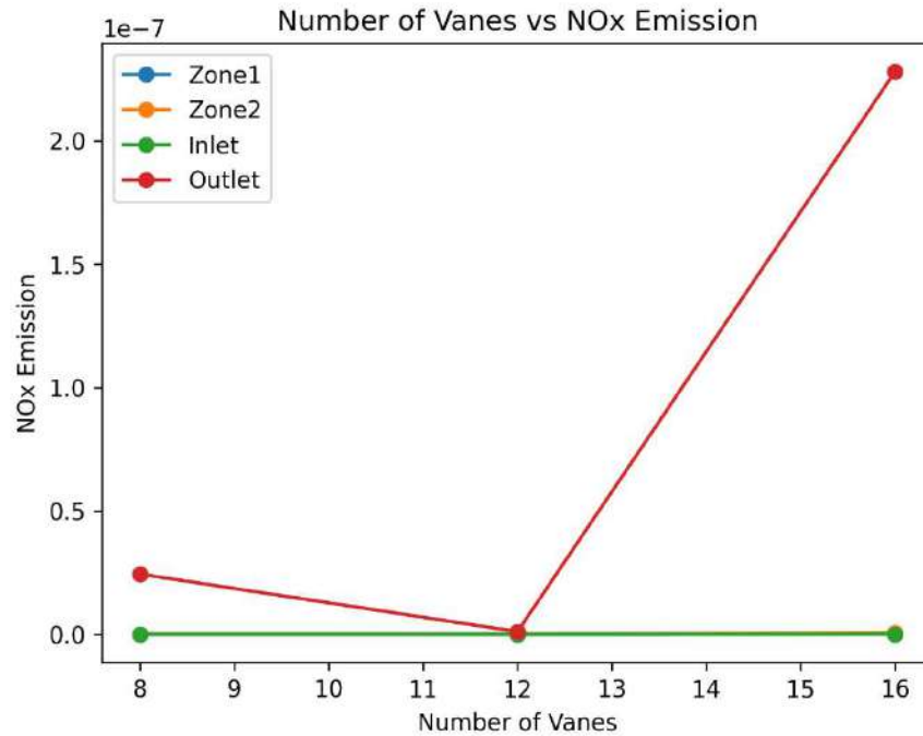
Fig.4.2.5 Number of Vanes vs NO x
