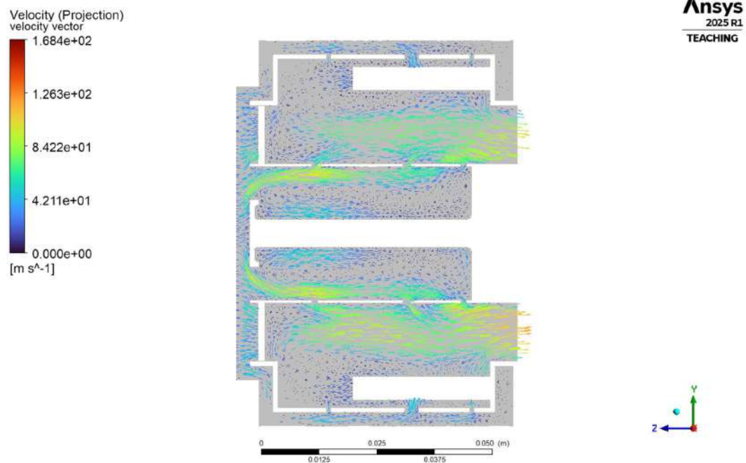
Fig.4.1.2.2(f) Cross-Section velocity vector Contour
