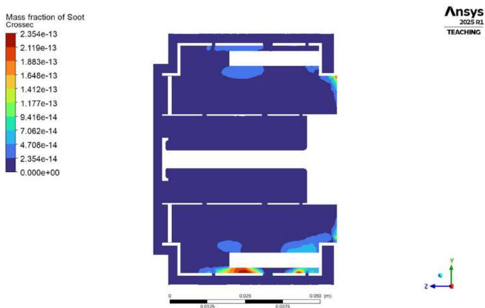
4.1.6.2(e) Cross-section Soot mass fraction
