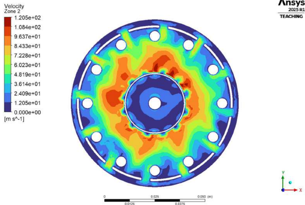
Fig.4.1.2.1(c) Zone 2 velocity Contour
