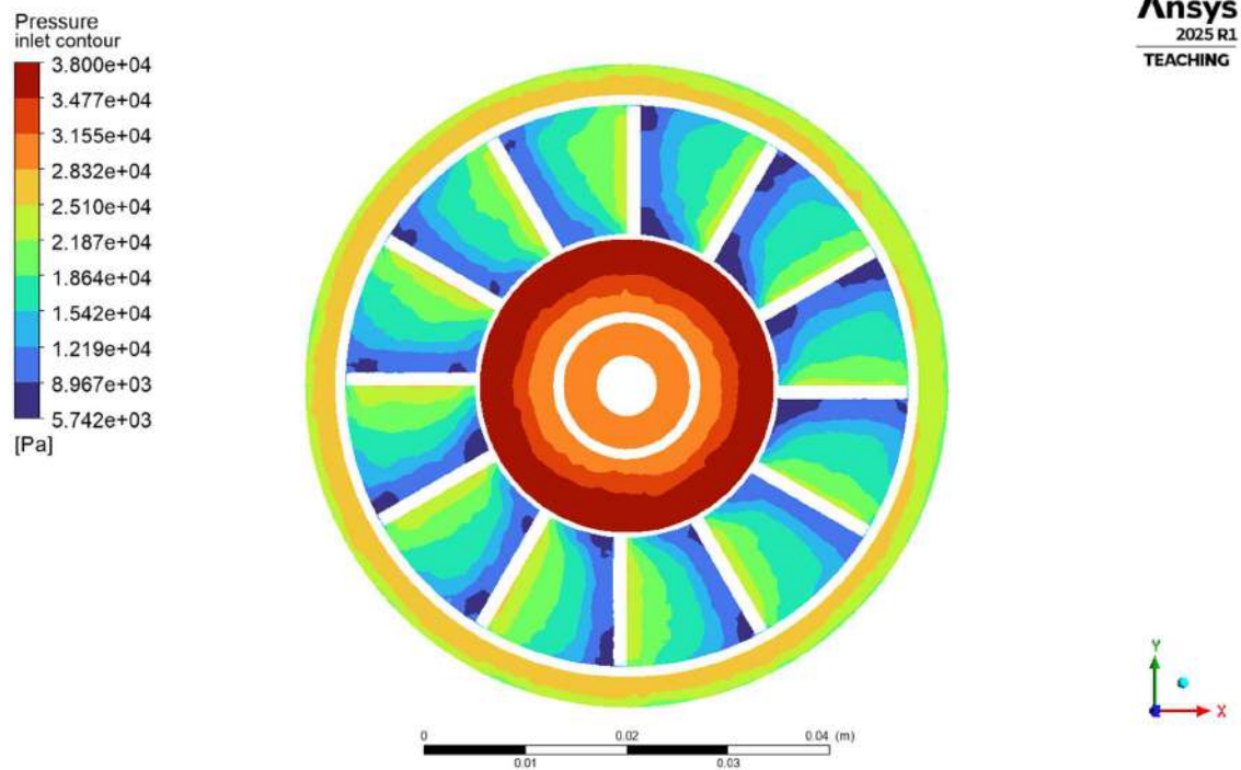
Fig.4.1.1.2(a) Inlet Pressure Contour
