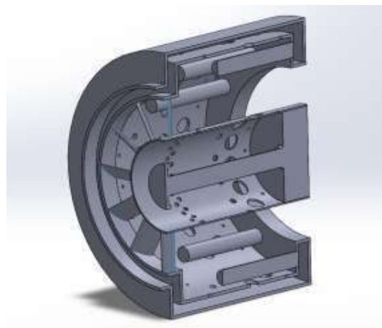
Fig.3.2 (b) 12 blade swirler with combustor Cross-sectional view
