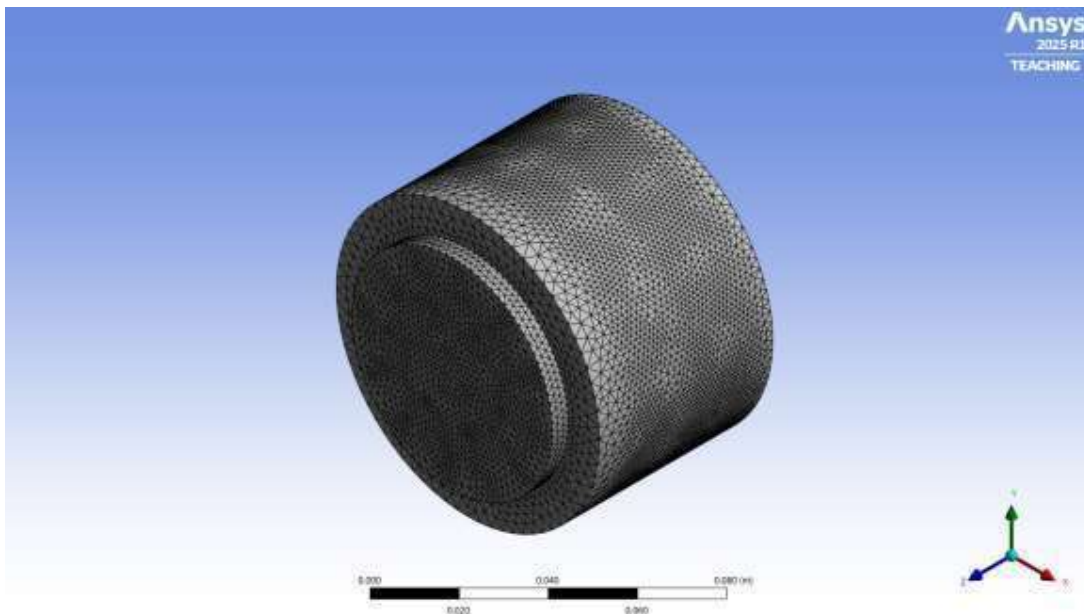
Fig.3.3 Meshing.
