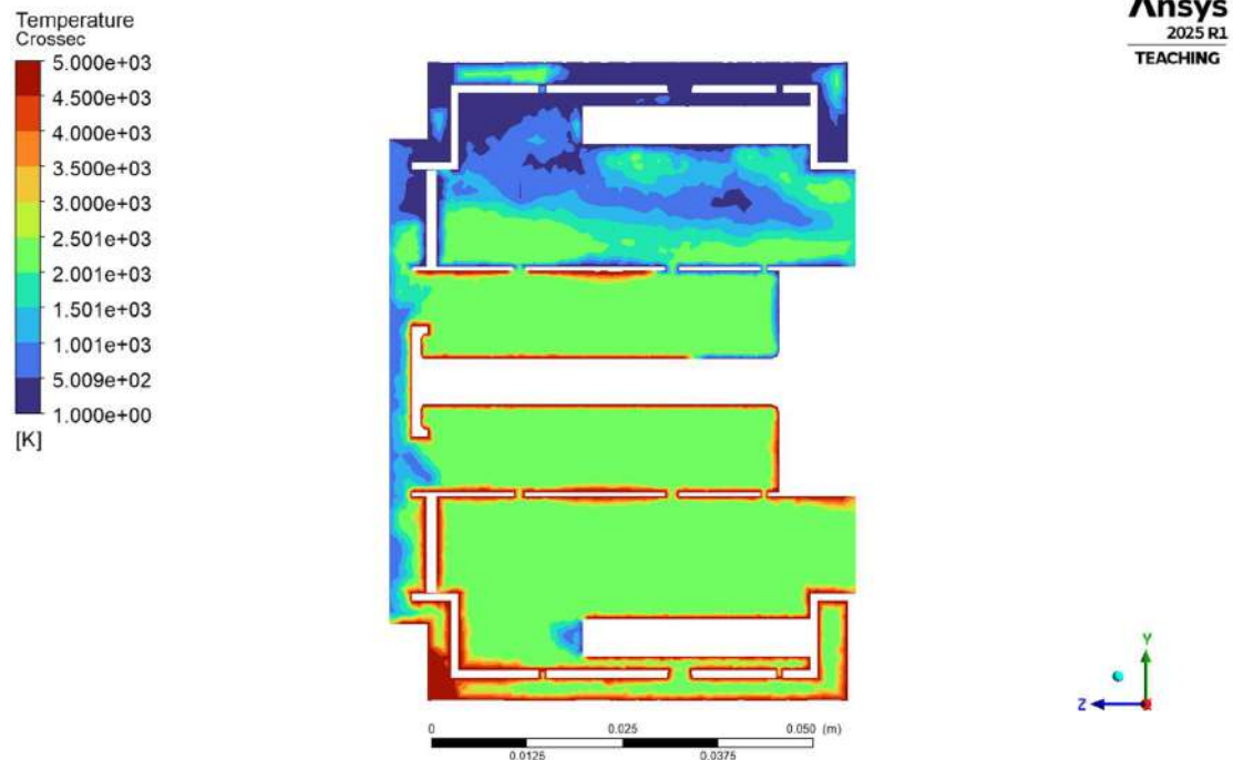
4.1.3.2(e) Cross-Section Temperature Distribution
