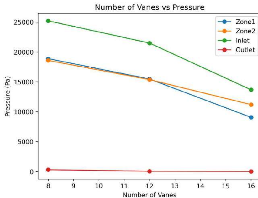
Fig.4.2.2 Number of Vanes vs Pressure (Pa)
