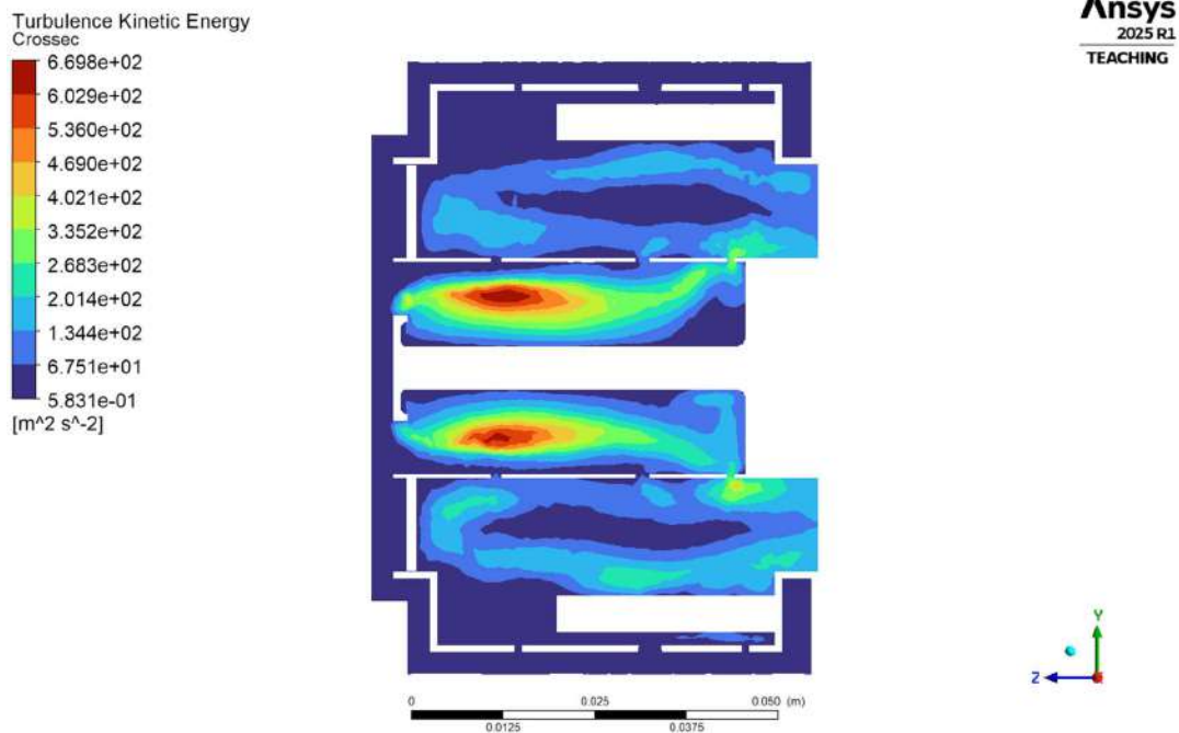
4.1.4.2(f) Cross-Section Turbulence Kinetic Energy
