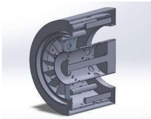
Fig.3.2 (c) 16 blade swirler with combustor Cross-sectional view
