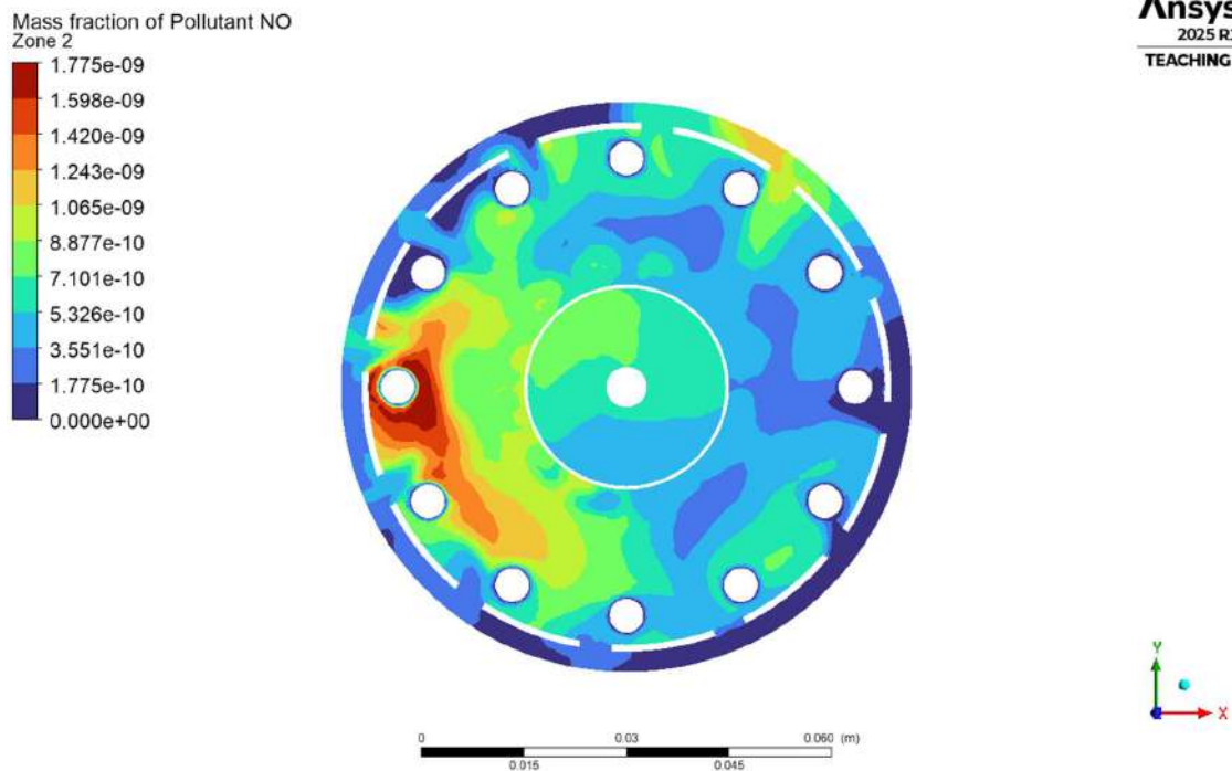
4.1.5.3(c) Zone 2 NO mass fraction
