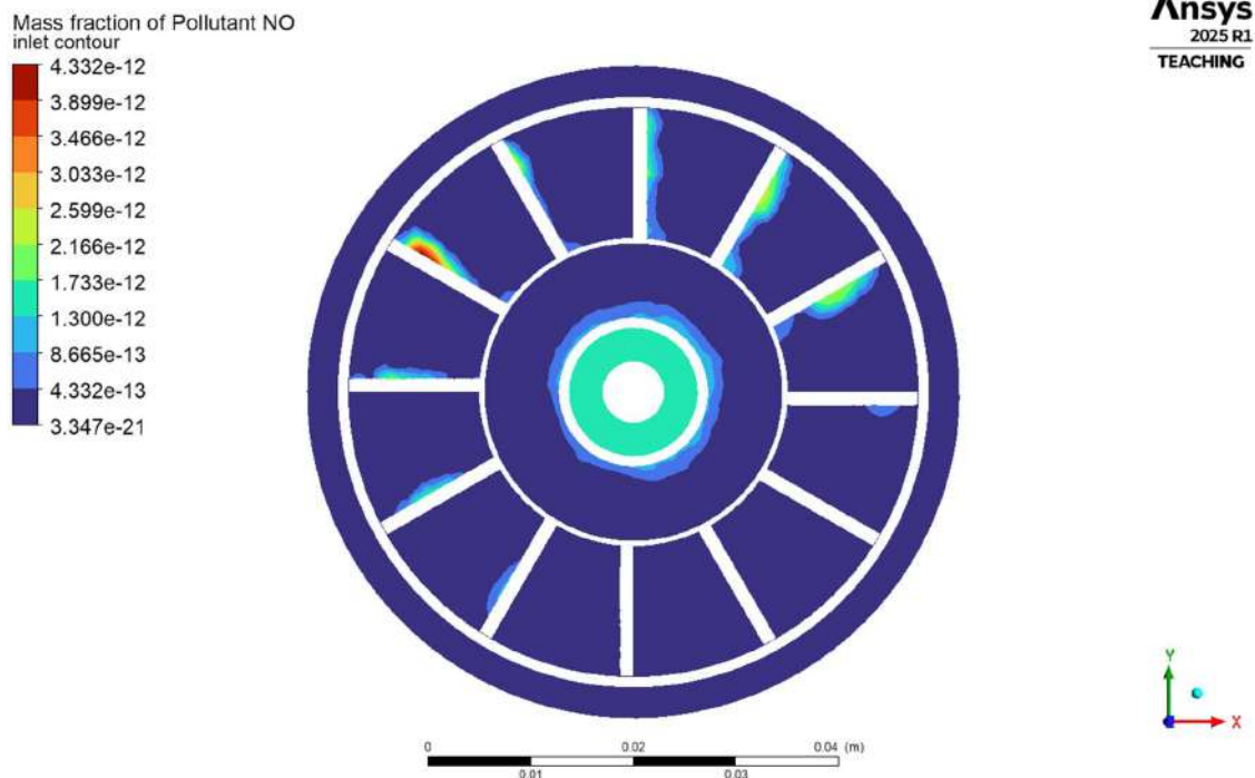
4.1.5.2(a) Inlet NO mass fraction
