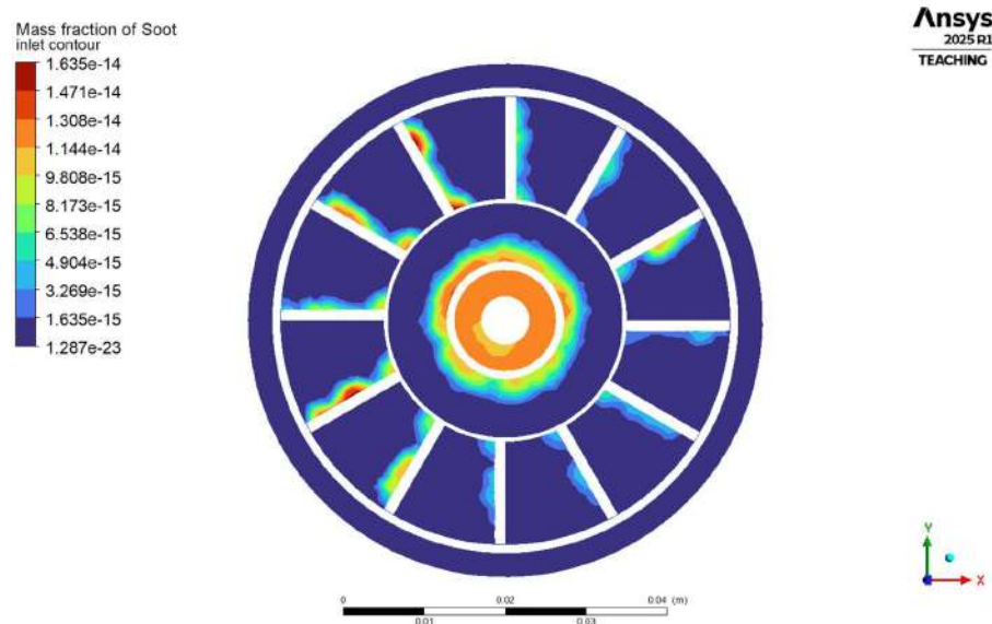
4.1.6.2(a) Inlet Soot mass fraction
