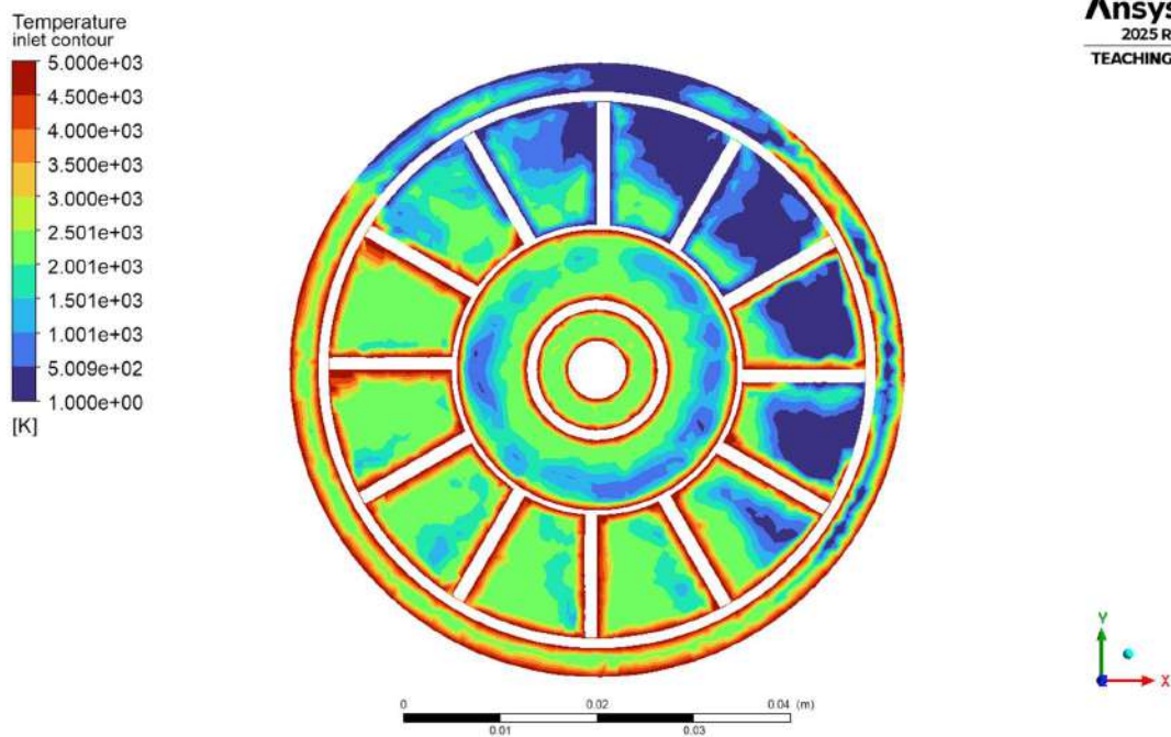
4.1.3.2(a) Inlet Temperature Contour
