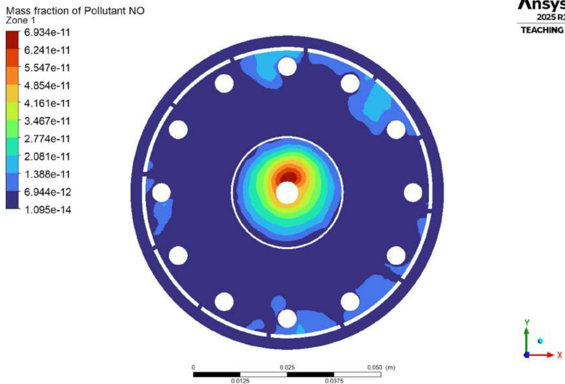
4.1.5.1(b) Mass Fraction of No_x Zone 1 Contour
