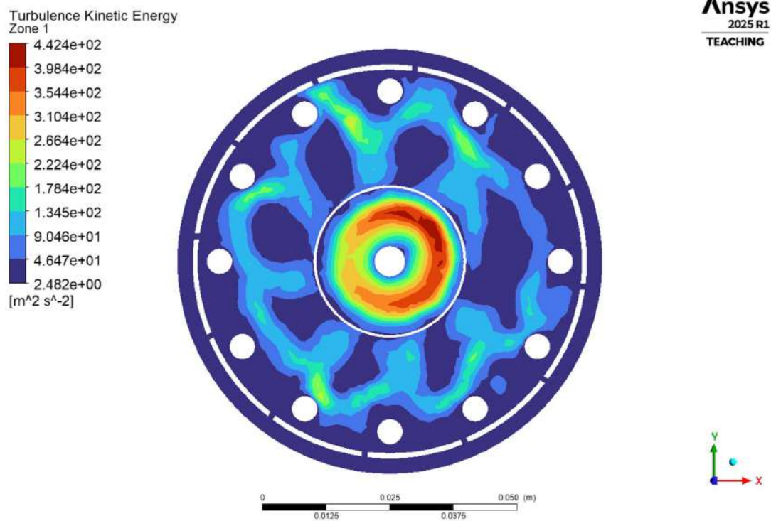
4.1.4.1(b) Turbulence Kinetic Energy in Zone 1
