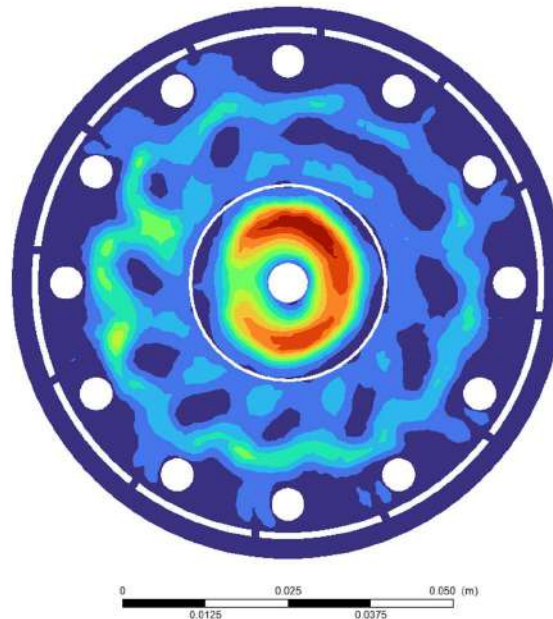
4.1.4.2(b) Zone 1 Turbulence Kinetic Energy
