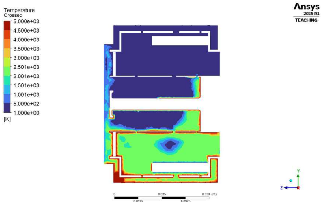
4.1.3.3(e) Cross-Section Temperature Distribution
