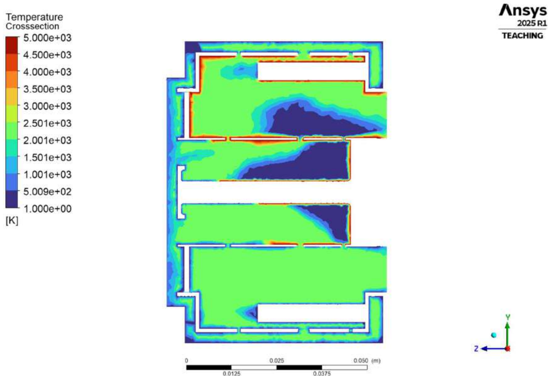
4.1.3.1(d) Cross-Section Temperature Distribution Contour
