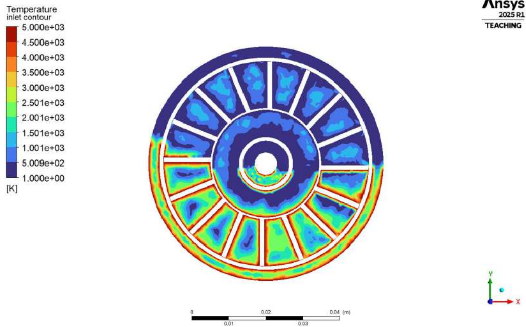
4.1.3.3(a) Inlet Temperature Distribution
