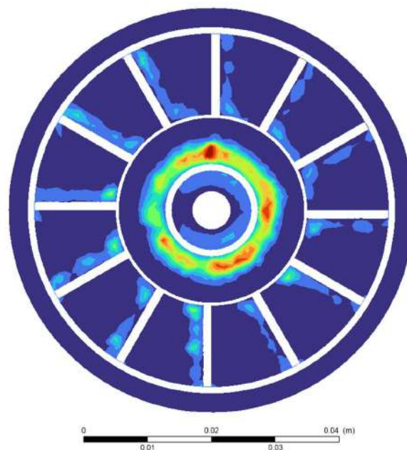
4.1.4.2(a) Inlet Turbulence Kinetic Energy
