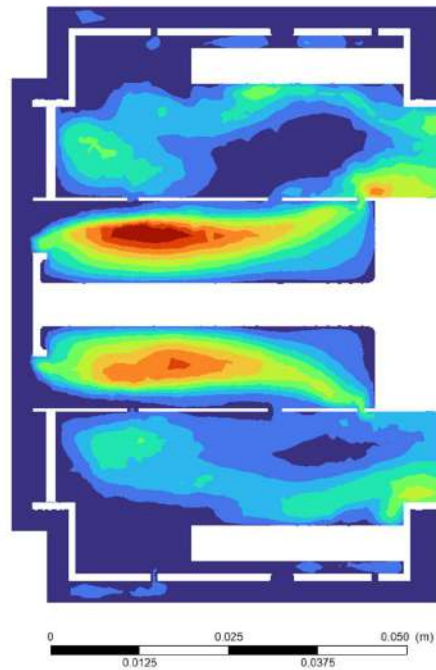
4.1.4.1(e) Cross-Section Turbulence Kinetic Energy
