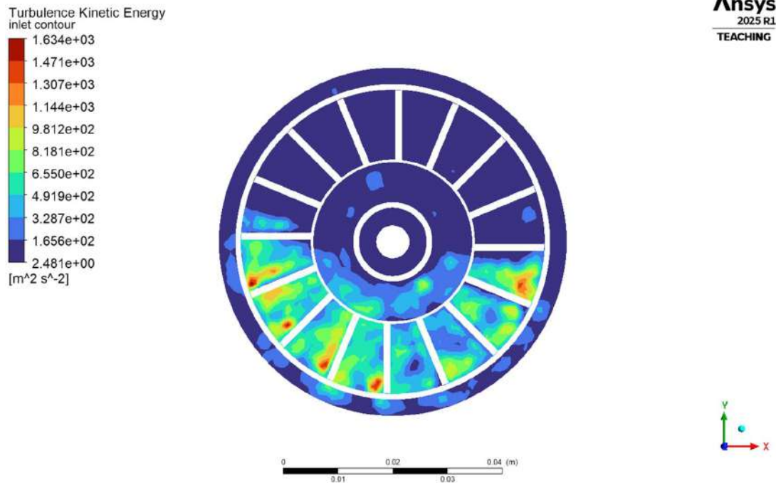
4.1.4.3(a) Inlet Turbulence Kinetic Energy
