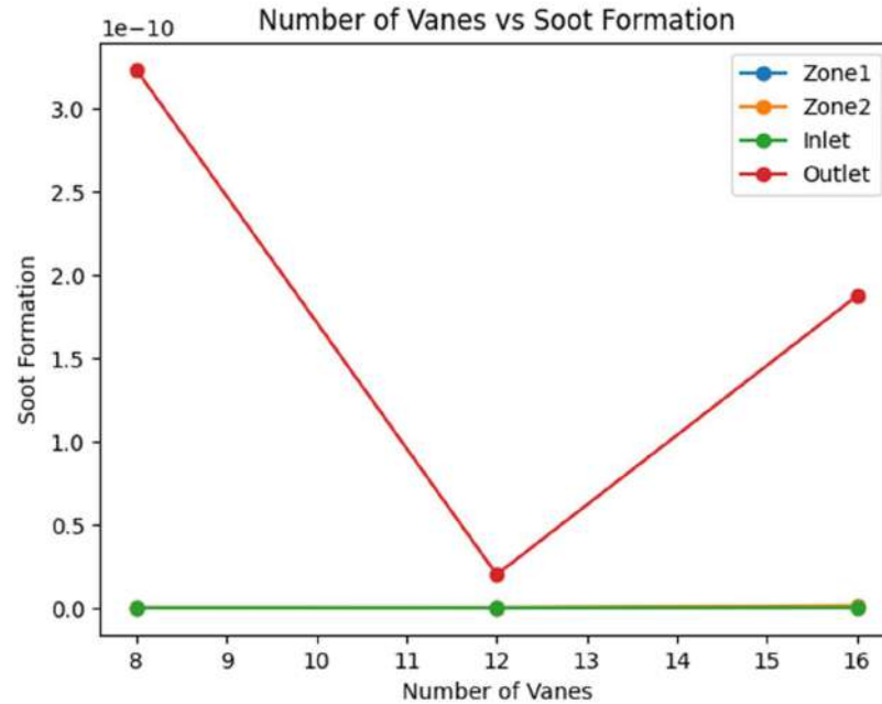
Fig.4.2.6 Number of Vanes vs Soot
