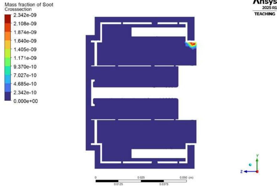
4.1.6.1(f) Cross-section Soot mass fraction
