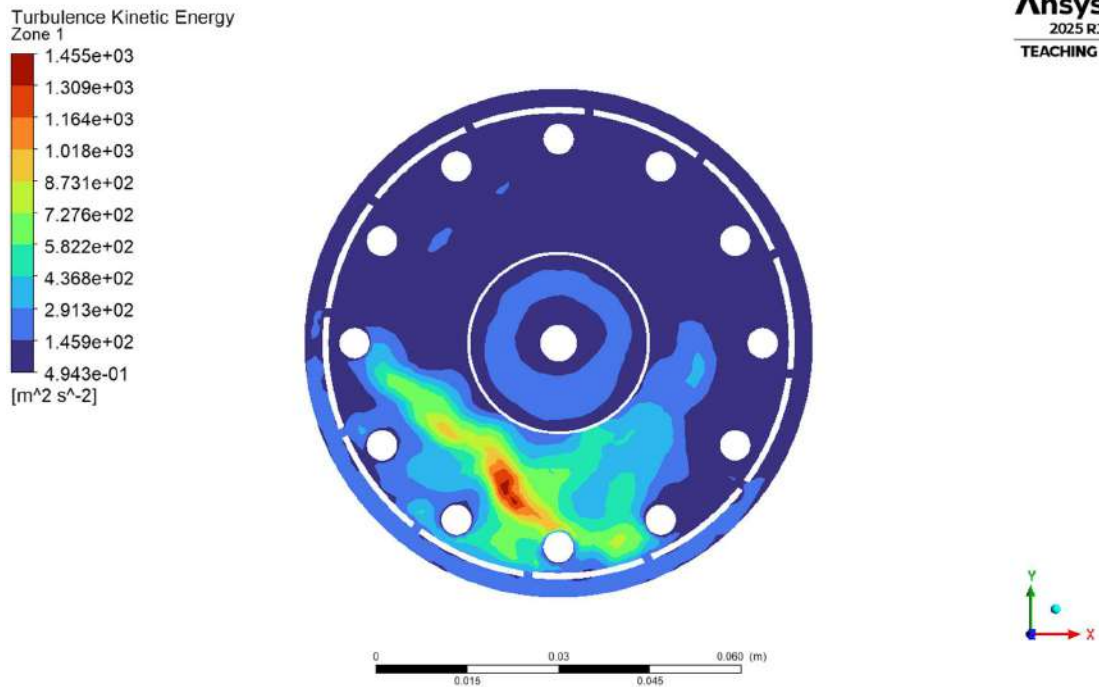
4.1.4.3(b) Zone 1 Turbulence Kinetic Energy
