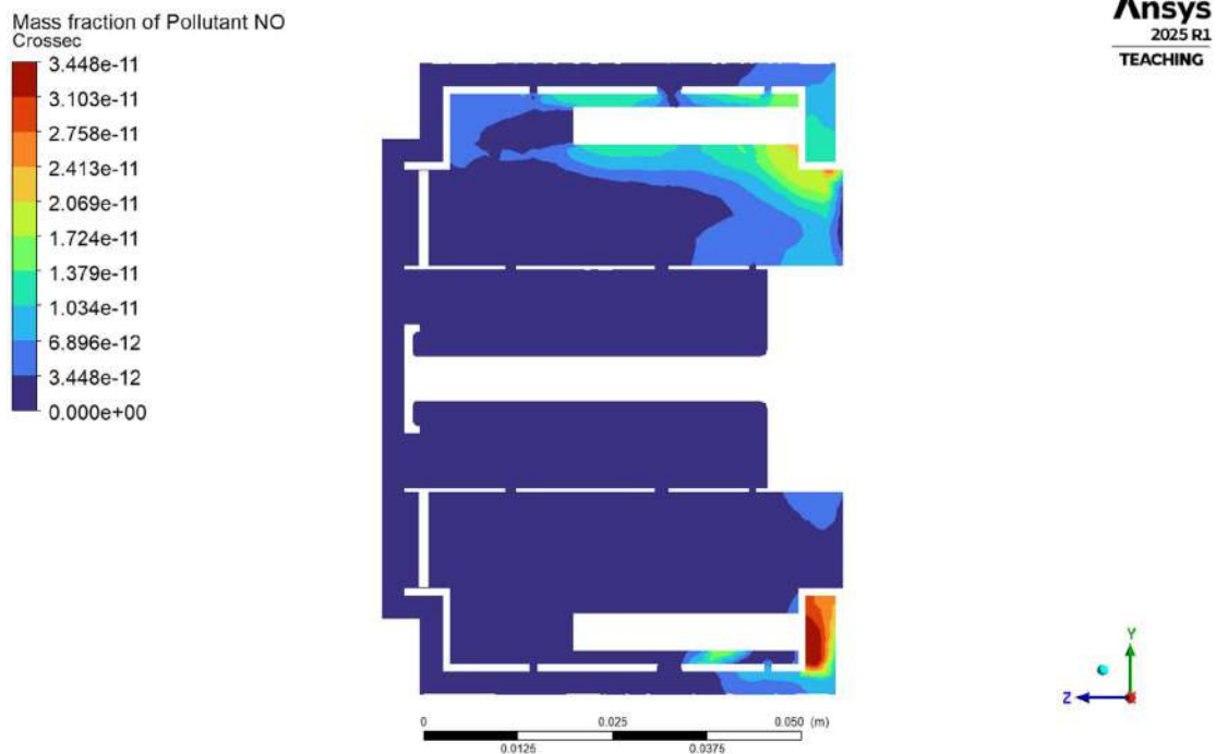
4.1.5.2(e) Cross-section NO mass fraction
