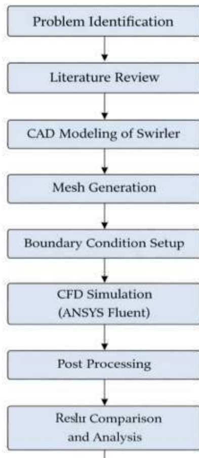
Fig.3.1 Methodology flow chart
