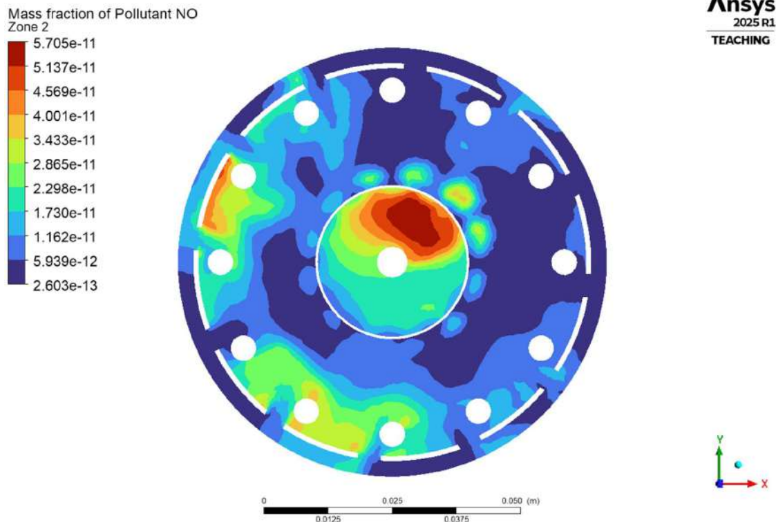
4.1.5.1(c) Mass Fraction of \text{No}_x Zone 2 Contour
