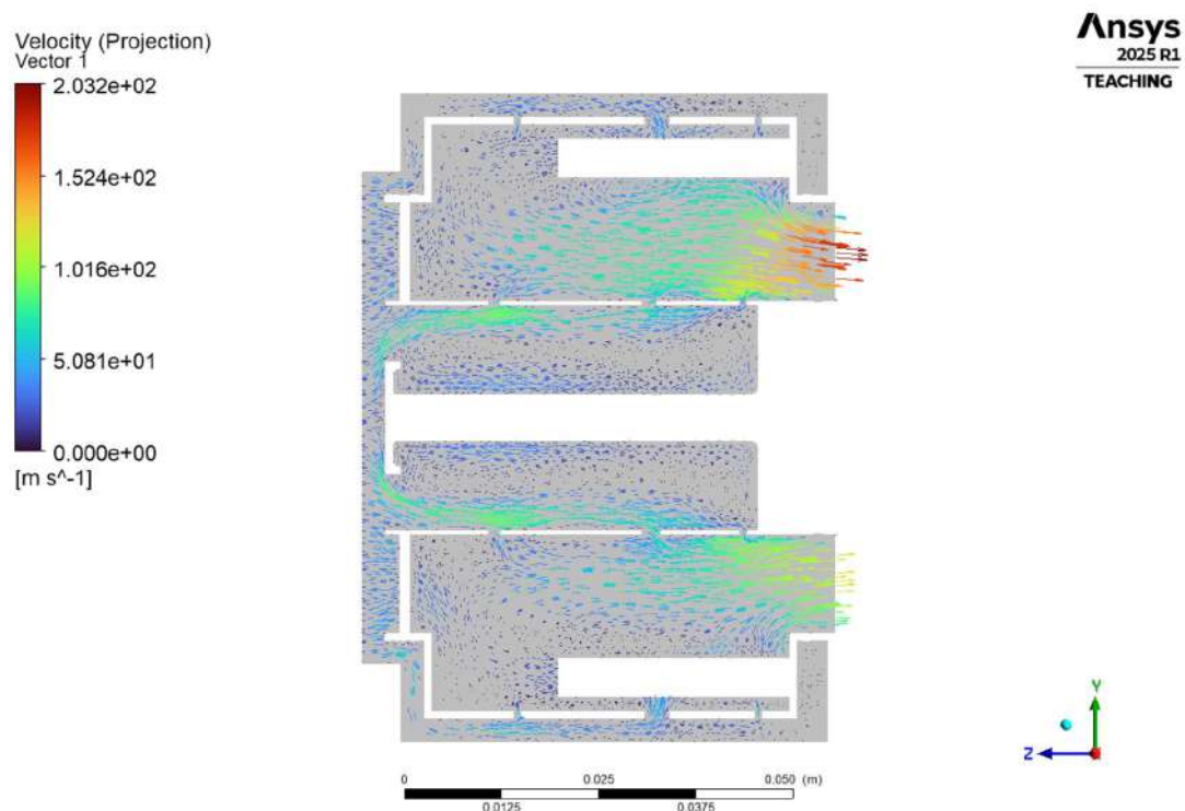
Fig.4.1.2.1(e) Cross-Section velocity vector Contour
