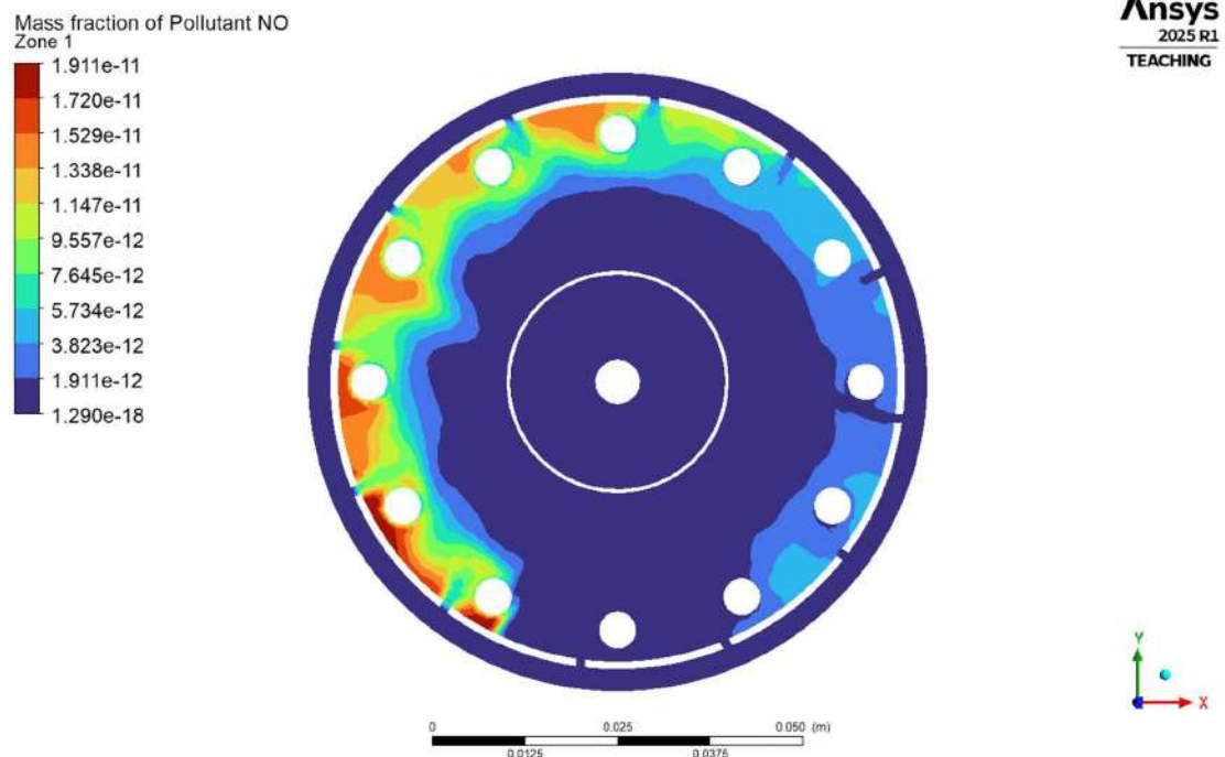
4.1.5.2(b) Zone 1 NO mass fraction
