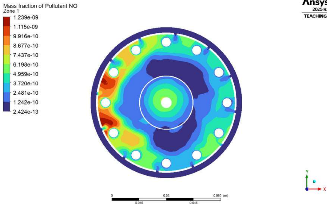
4.1.5.3(b) Zone 1 NO mass fraction
