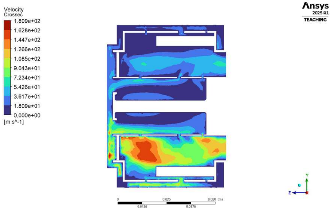
Fig.4.1.2.1(e) Cross-Section velocity Contour
