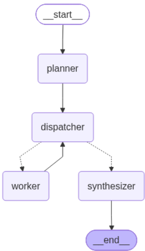
The compiled LangGraph, emitted from the running application by docs/render-graph.py .
