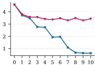
Distinct-4
