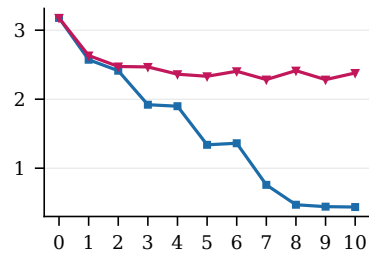
Distinct-3
