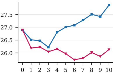
Distinct-1
