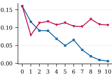
Distinct-1
