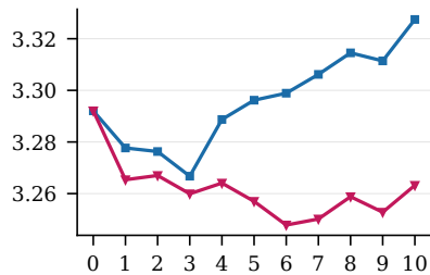
Distinct-2
