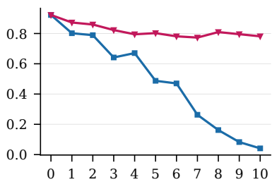
Distinct-4
