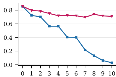
Distinct-3
