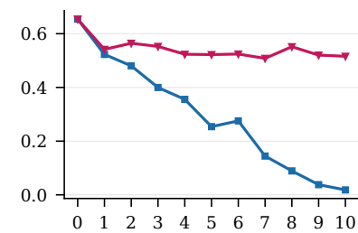
Distinct-2
