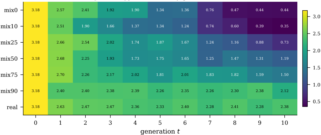
Output entropy (nats/token) | generations 0-10
