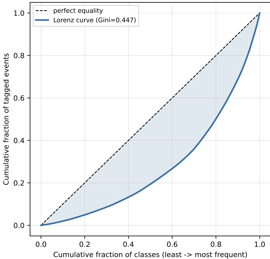
Lorenz curve
