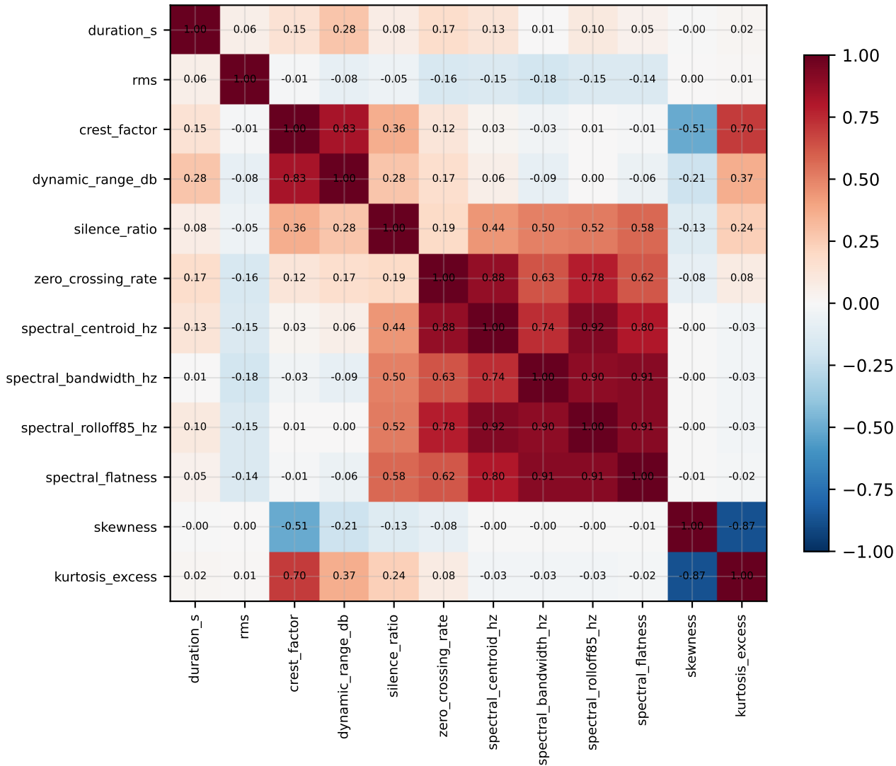
Feature correlations
