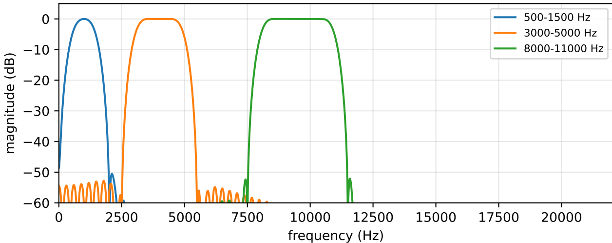
SincConv filters (frequency domain)
