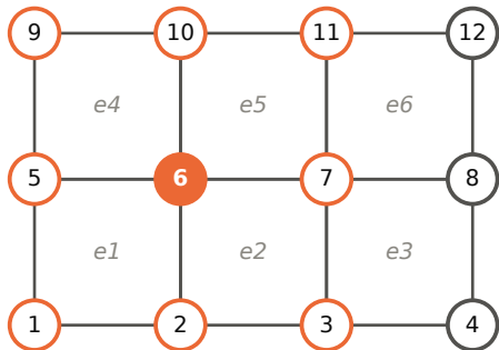
Malla 3 x 2 Q4: 12 nodos, 24 GDL
