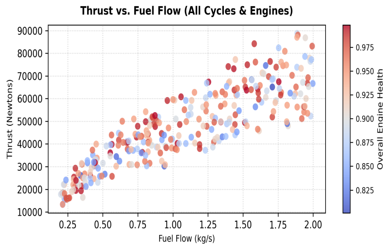
Figure 5: Output Engine Net Thrust (N) vs Fuel Flow (kg/s) Validation Fit
