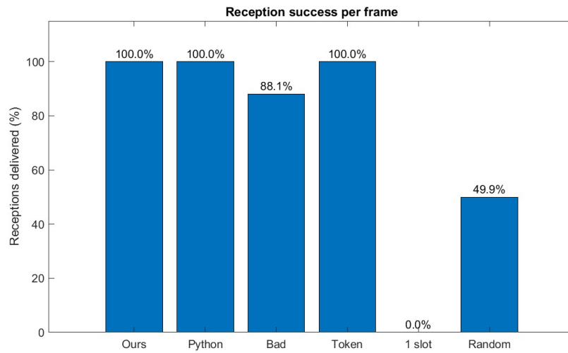
Figure 3. Share of possible receptions delivered in each scenario.
