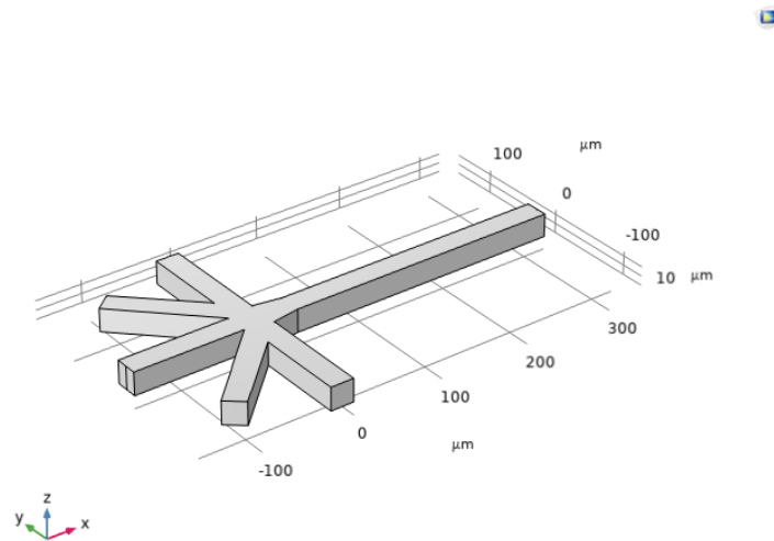
Figure 2: Schematic representation of the star-shaped microchannel geometry with five inlet branches converging into a single outlet.
