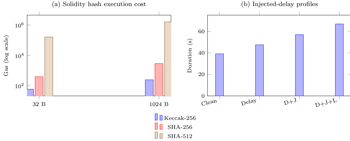
Figure 4: Consolidated cost and stress results. Panel (a) uses a logarithmic axis because the Solidity SHA-512 implementation is orders of magnitude more expensive; panel (b) reports observed workflow duration under cumulative delay (D), jitter (J), and loss/retry (L) injection. These experiments have distinct workloads and should not be interpreted as a single end-to-end deployment benchmark.
