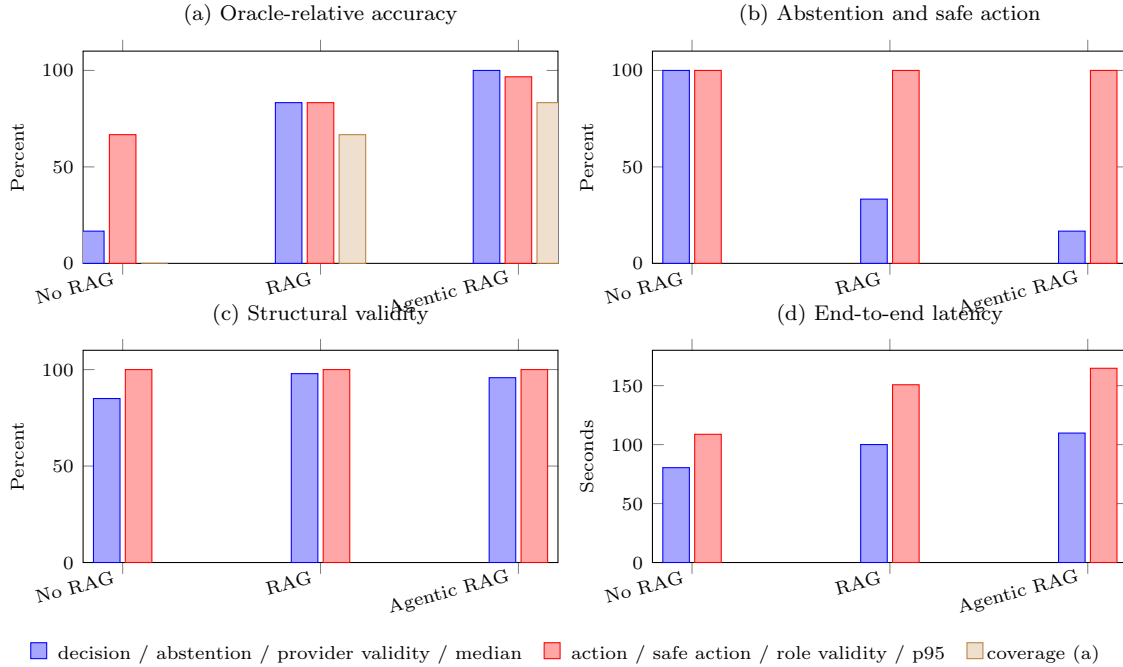
Figure 3: Consolidated frozen-oracle results (60 runs per mode). In (b), the series are abstention and safe-action rate; in (c), provider-schema and role-schema validity; in (d), median and p95 latency. Accuracy is relative to the synthetic oracle, and latency targets Non-RT rather than Near-RT control.
