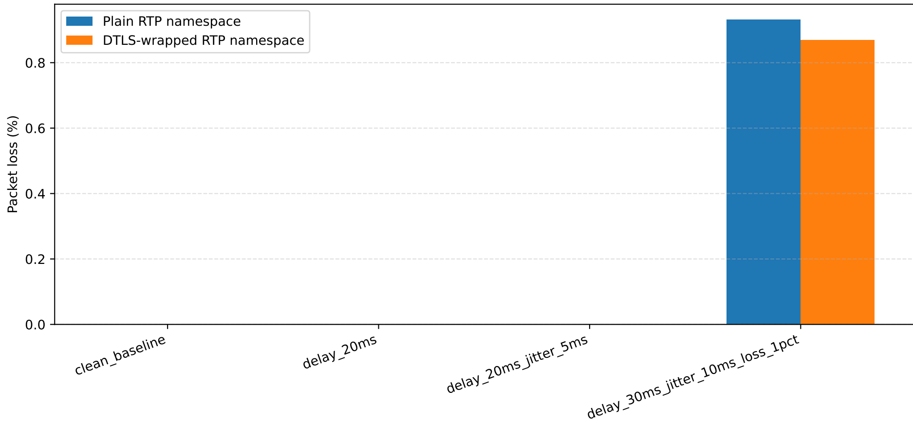
Packet loss (%) under namespace impairment
