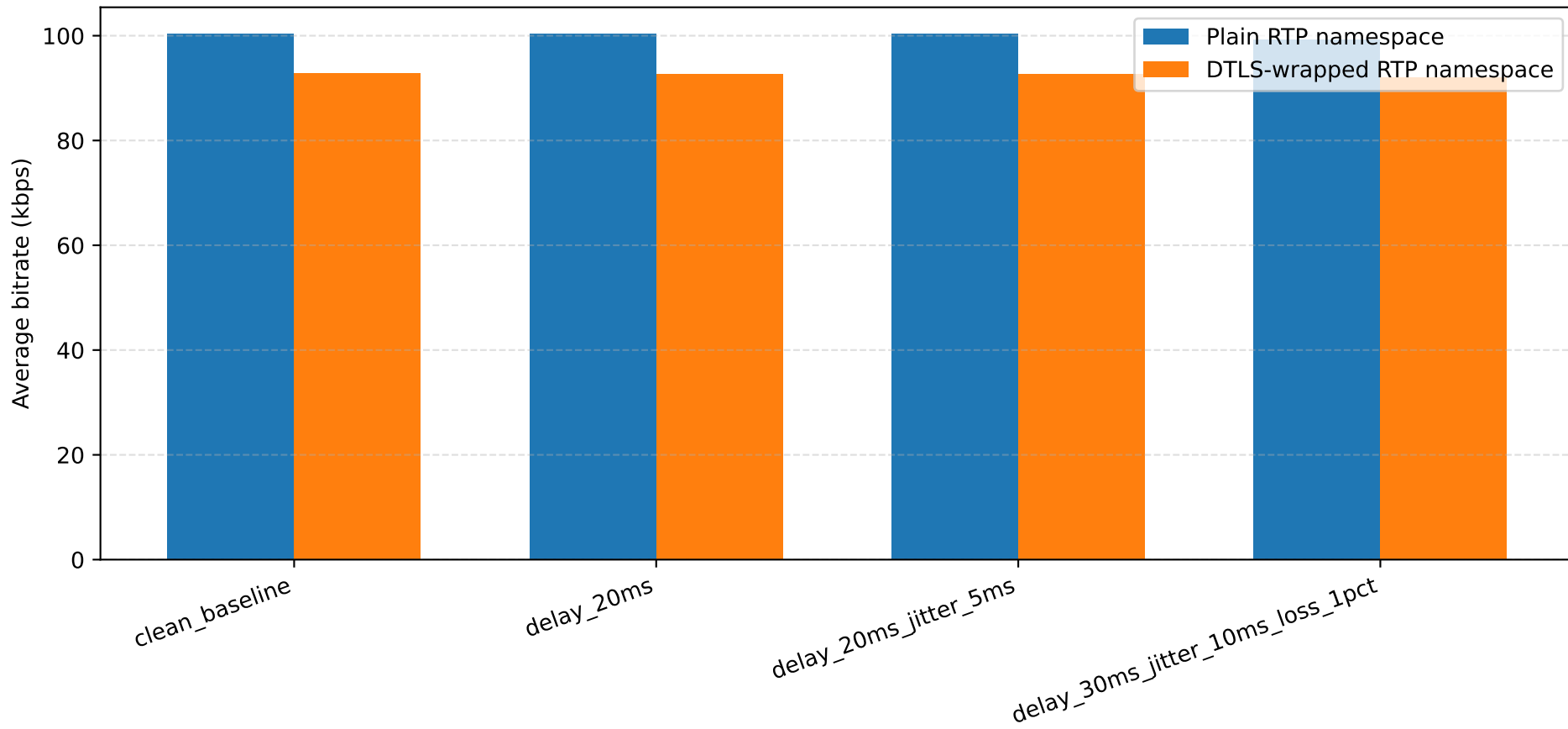
Average bitrate (kbps) under namespace impairment
