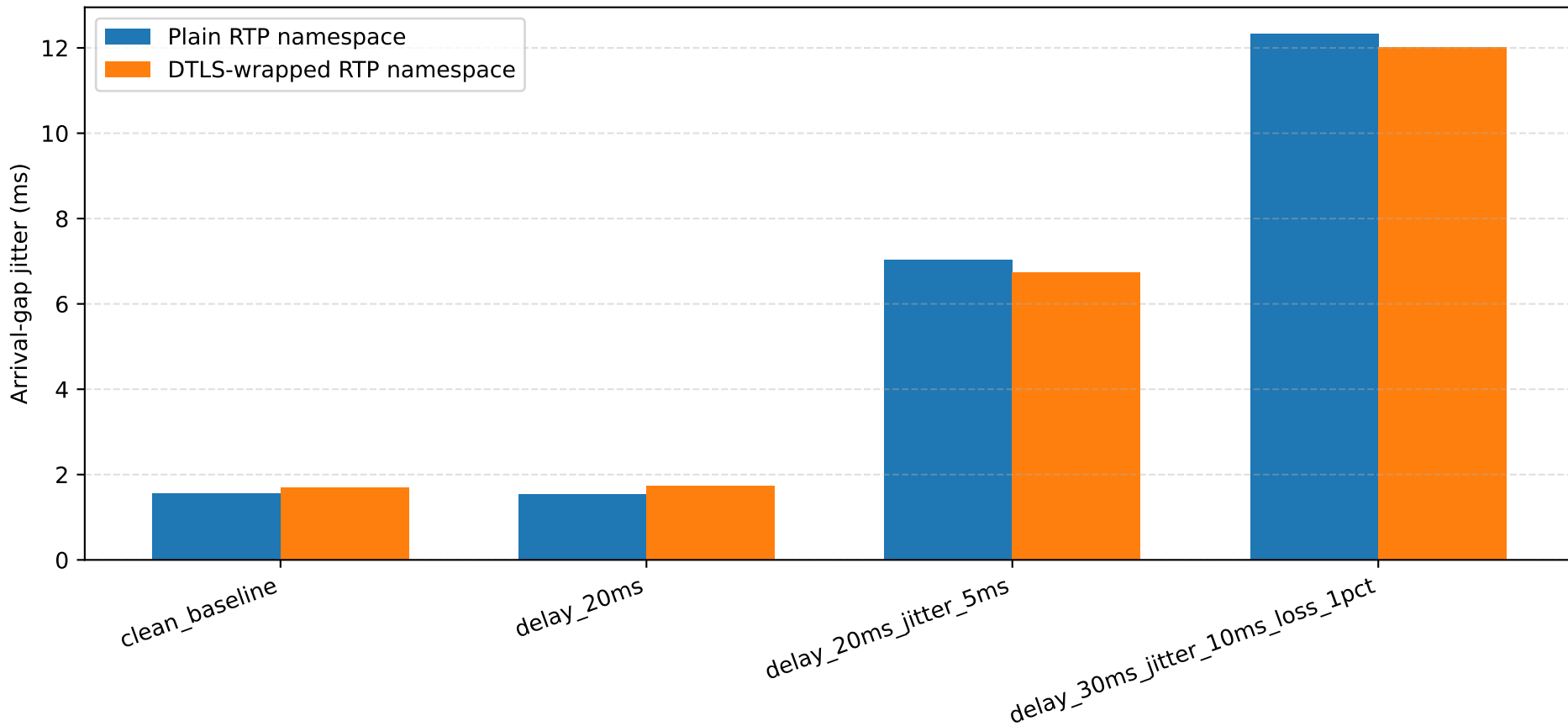
Arrival-gap jitter (ms) under namespace impairment
