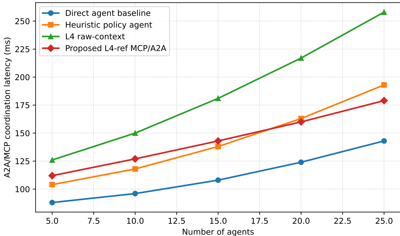
Figure 5.3: Agent Scaling of Level 4 Coordination
