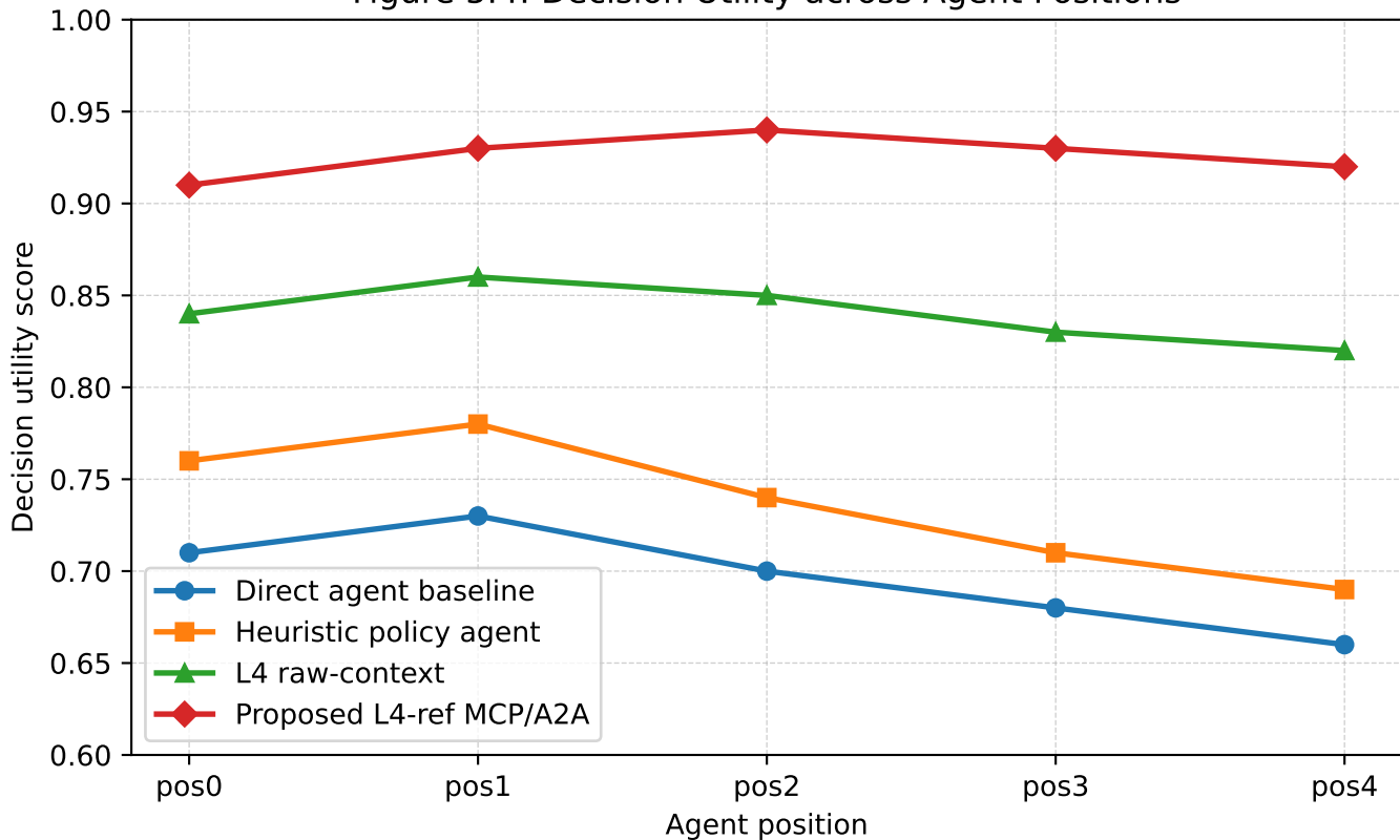
Figure 5.4: Decision Utility across Agent Positions
