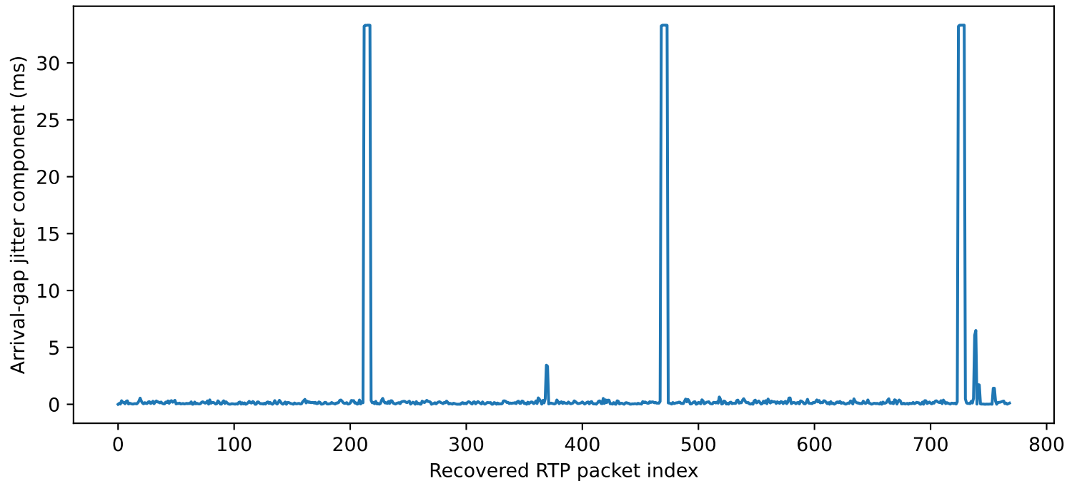
Figure 5.13: DTLS-Wrapped RTP Arrival-Gap Jitter
