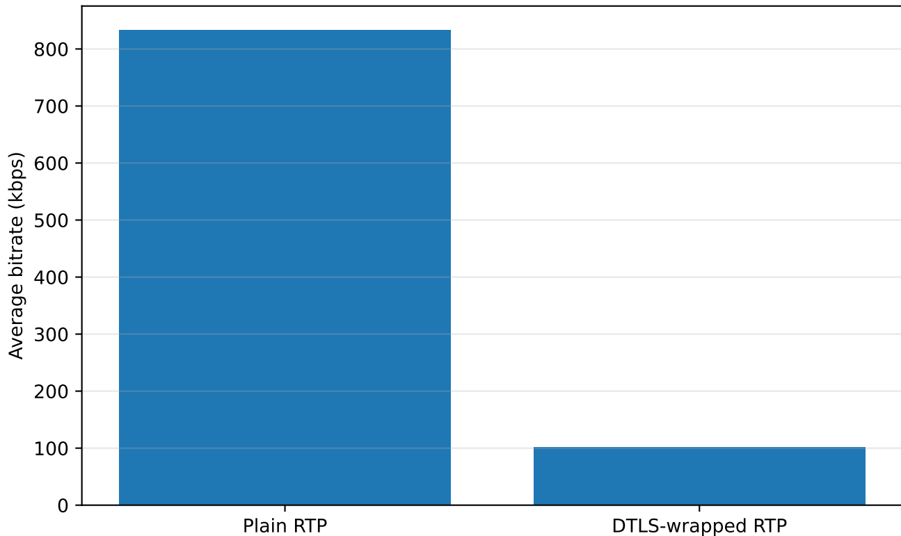
Figure 5.15: Plain RTP vs DTLS-wrapped RTP bitrate
