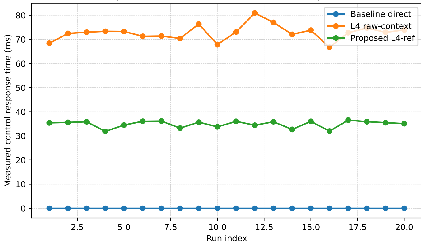
Figure 5.5: Semi-Live MCP/A2A Control Response
