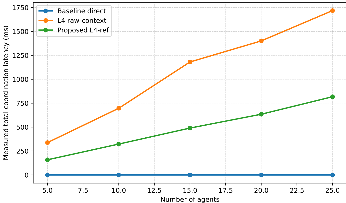
Figure 5.7: Multi-Agent Scaling Latency
