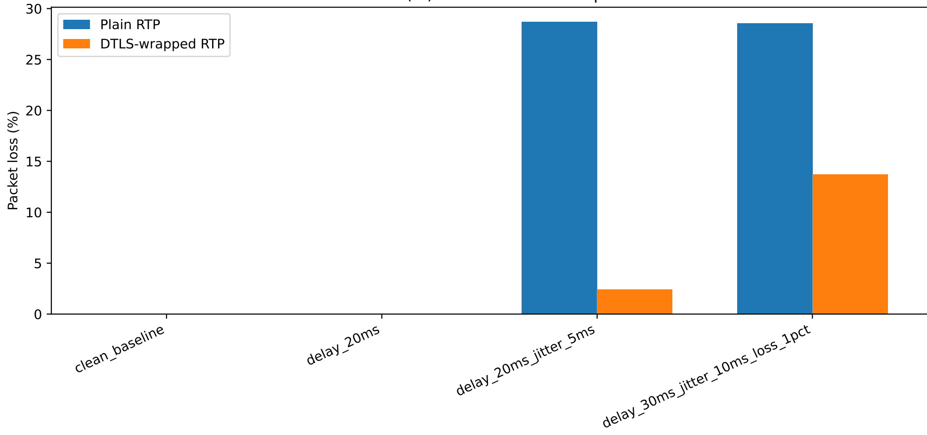
Packet loss (%) under controlled impairment
