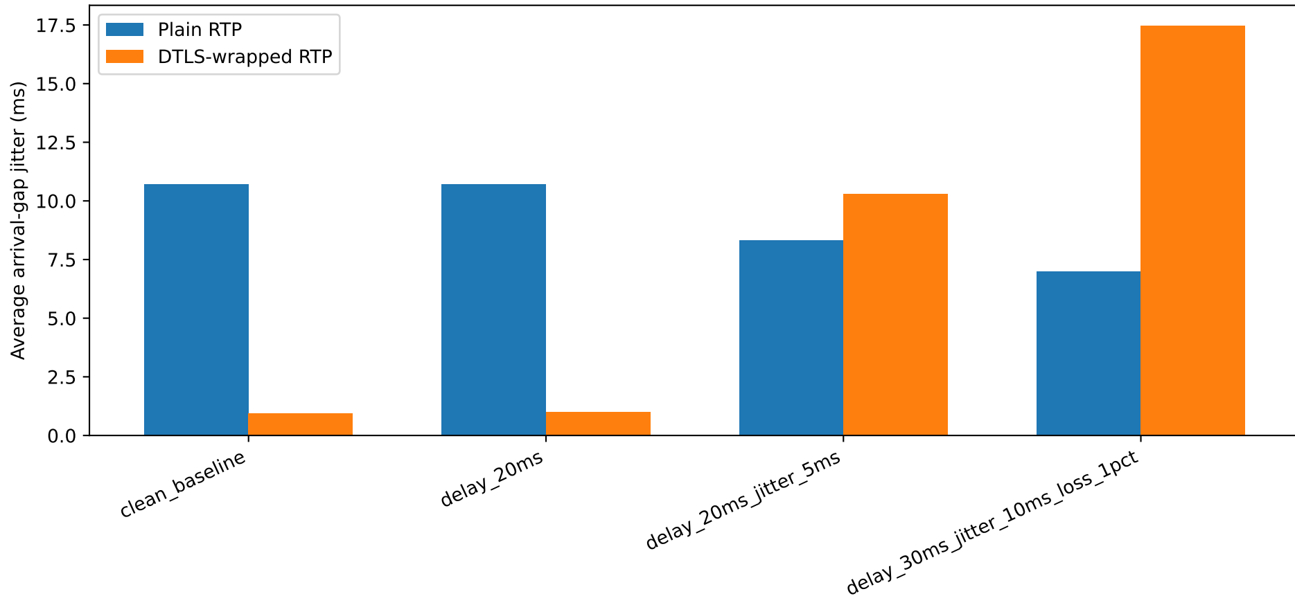
Average arrival-gap jitter (ms) under controlled impairment
