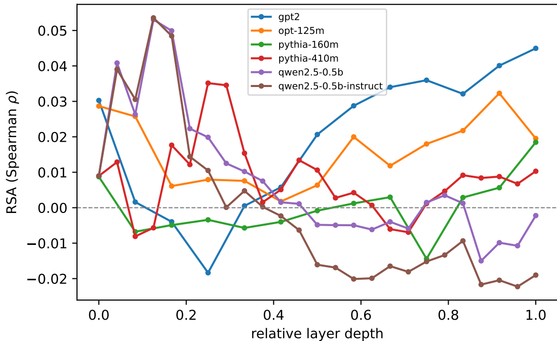
Representational geometry alignment
