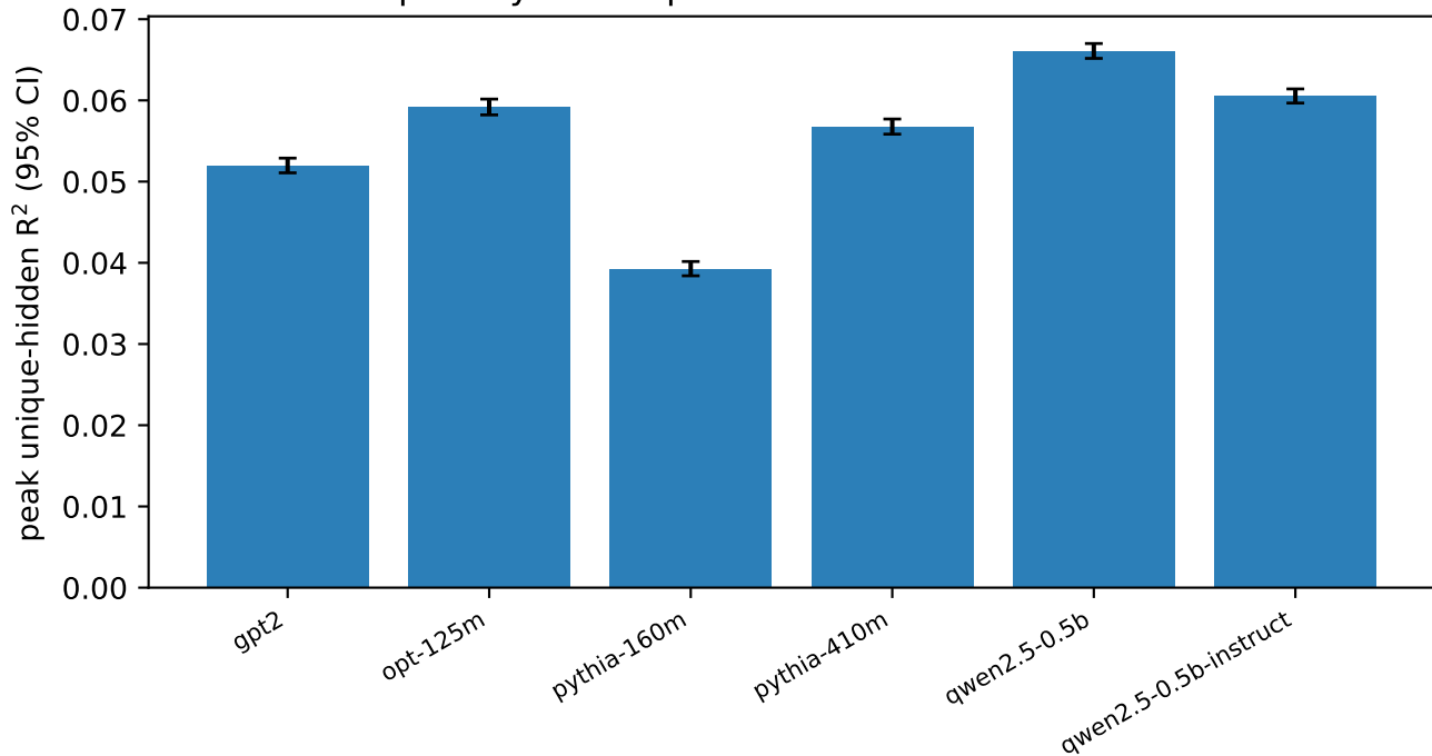
Unique-beyond-surprisal contribution across models
