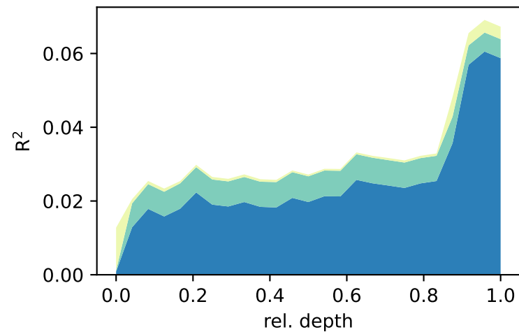
qwen2.5-0.5b-instruct
