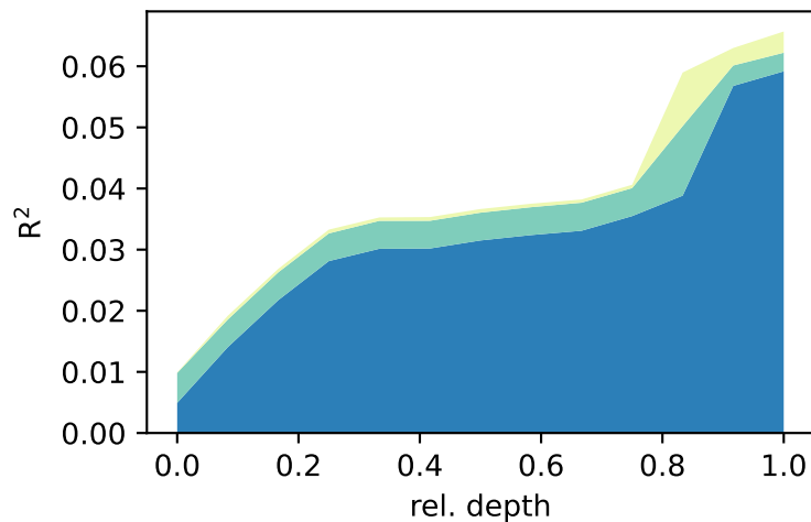
qwen2.5-0.5b
