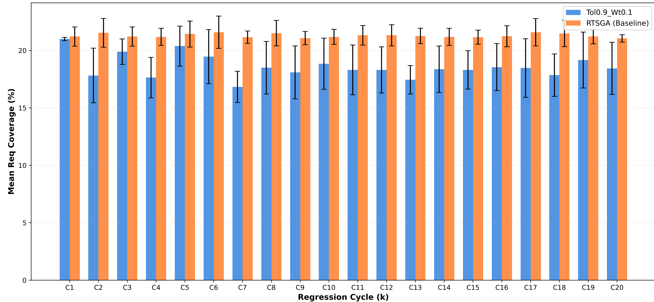
Req Coverage: Tol0.9_Wt0.1 vs RTSGA
