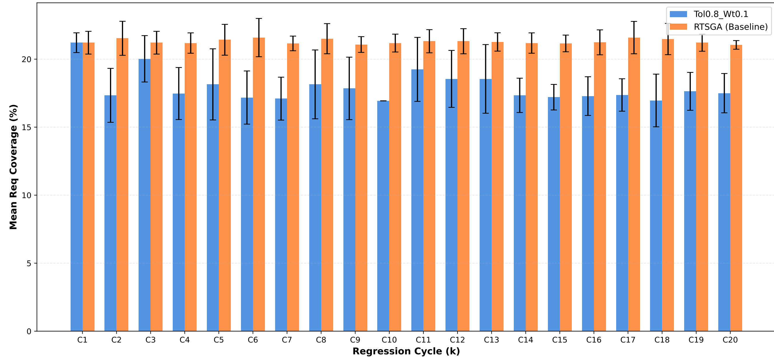
Req Coverage: Tol0.8_Wt0.1 vs RTSGA
