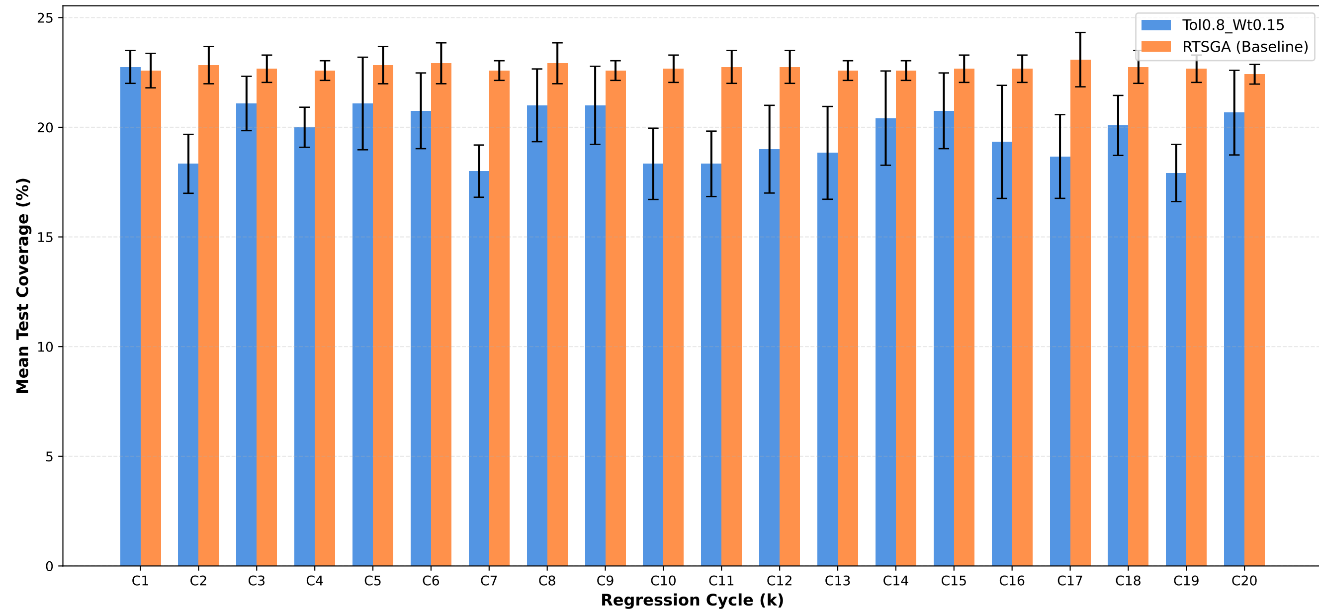
Test Coverage: Tol0.8_Wt0.15 vs RTSGA
