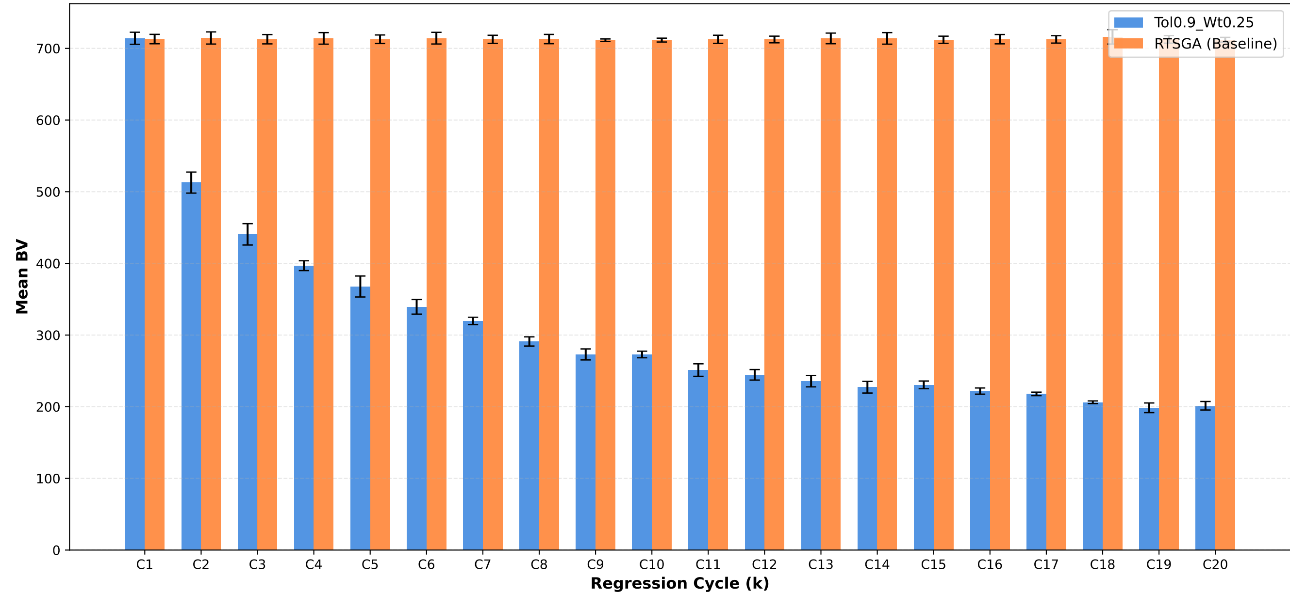
Business Value: Tol0.9_Wt0.25 vs RTSGA
