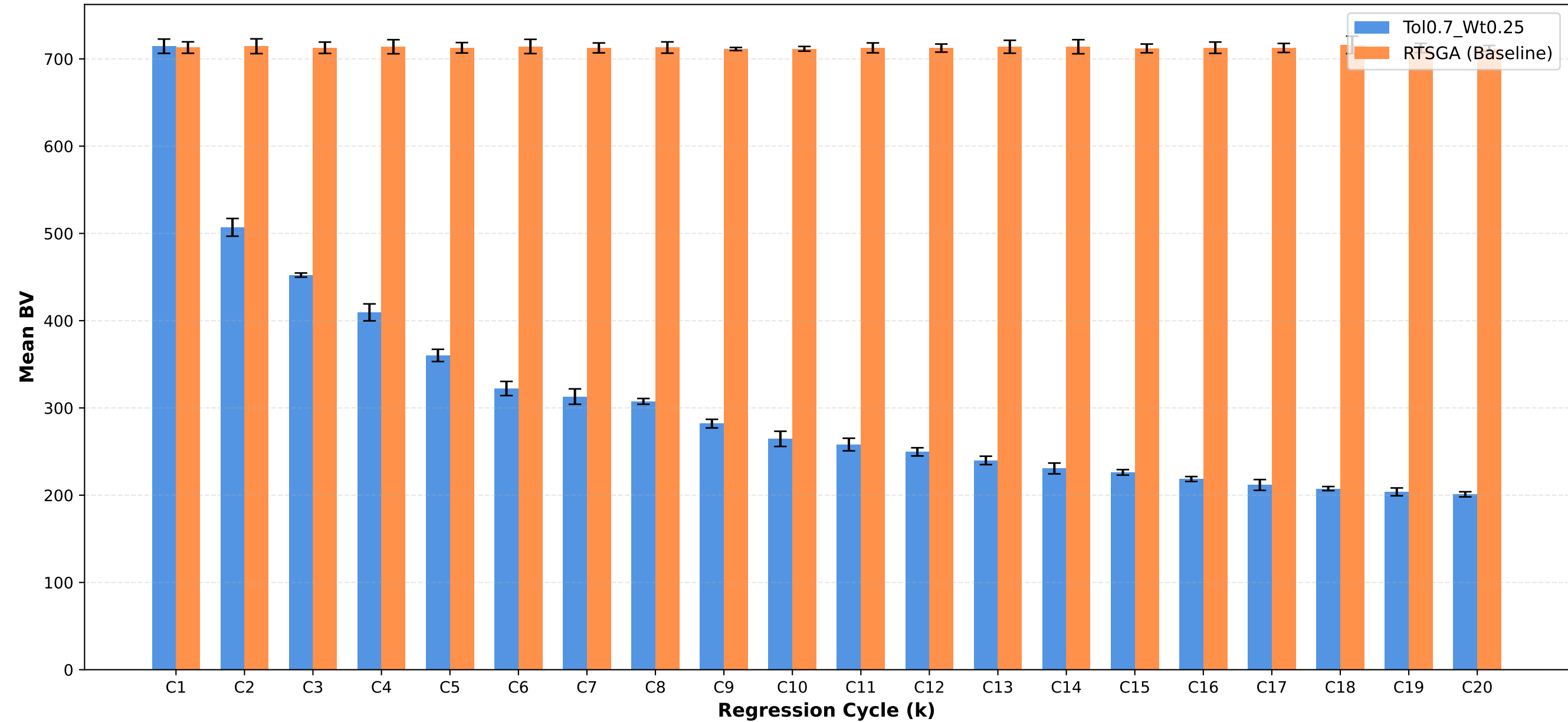
Business Value: Tol0.7_Wt0.25 vs RTSGA
