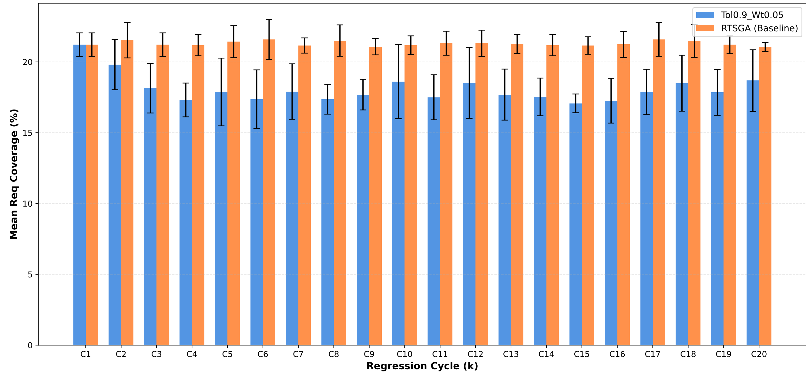
Req Coverage: Tol0.9_Wt0.05 vs RTSGA
