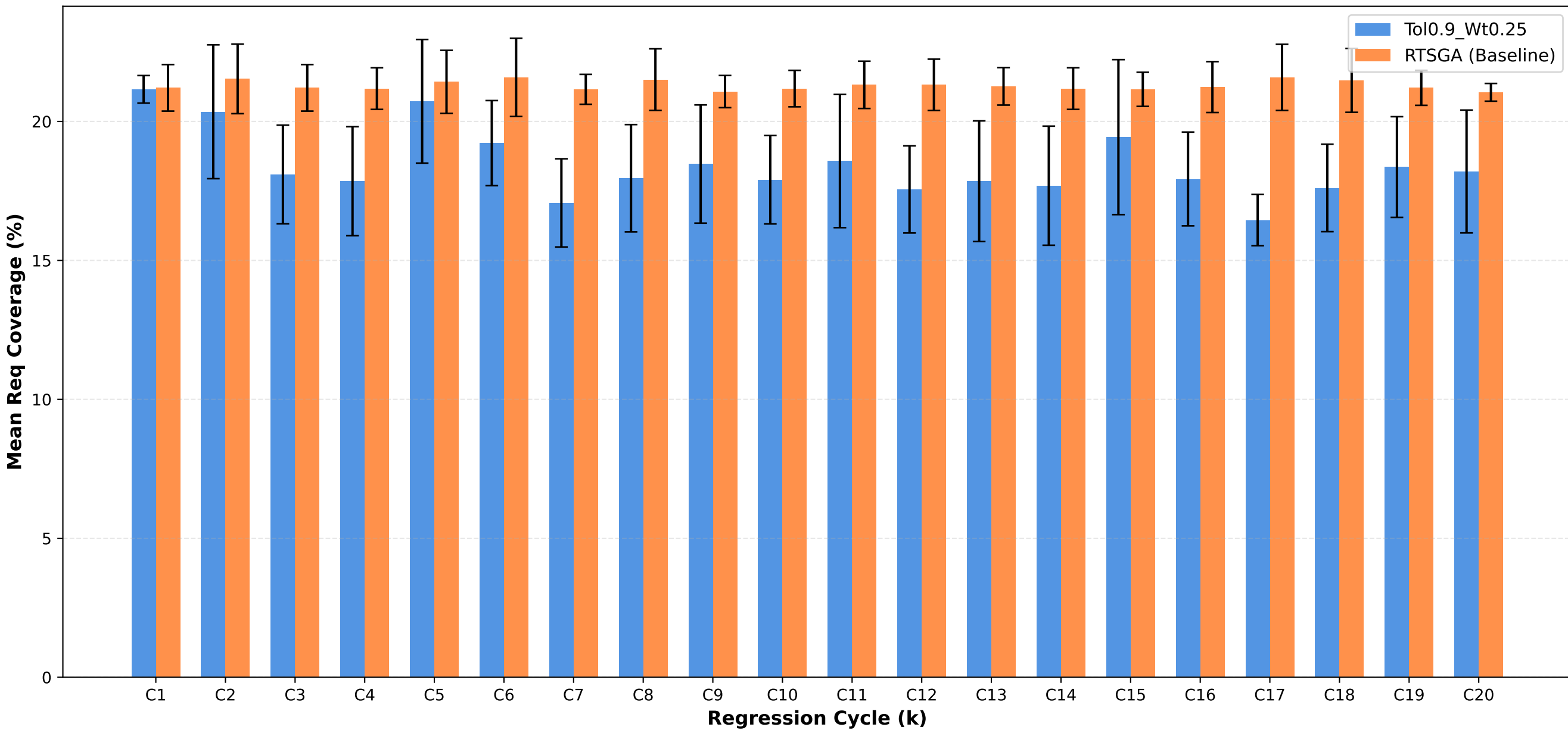
Req Coverage: Tol0.9_Wt0.25 vs RTSGA
