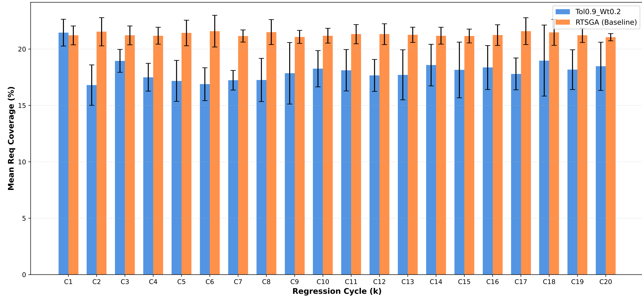
Req Coverage: Tol0.9_Wt0.2 vs RTSGA
