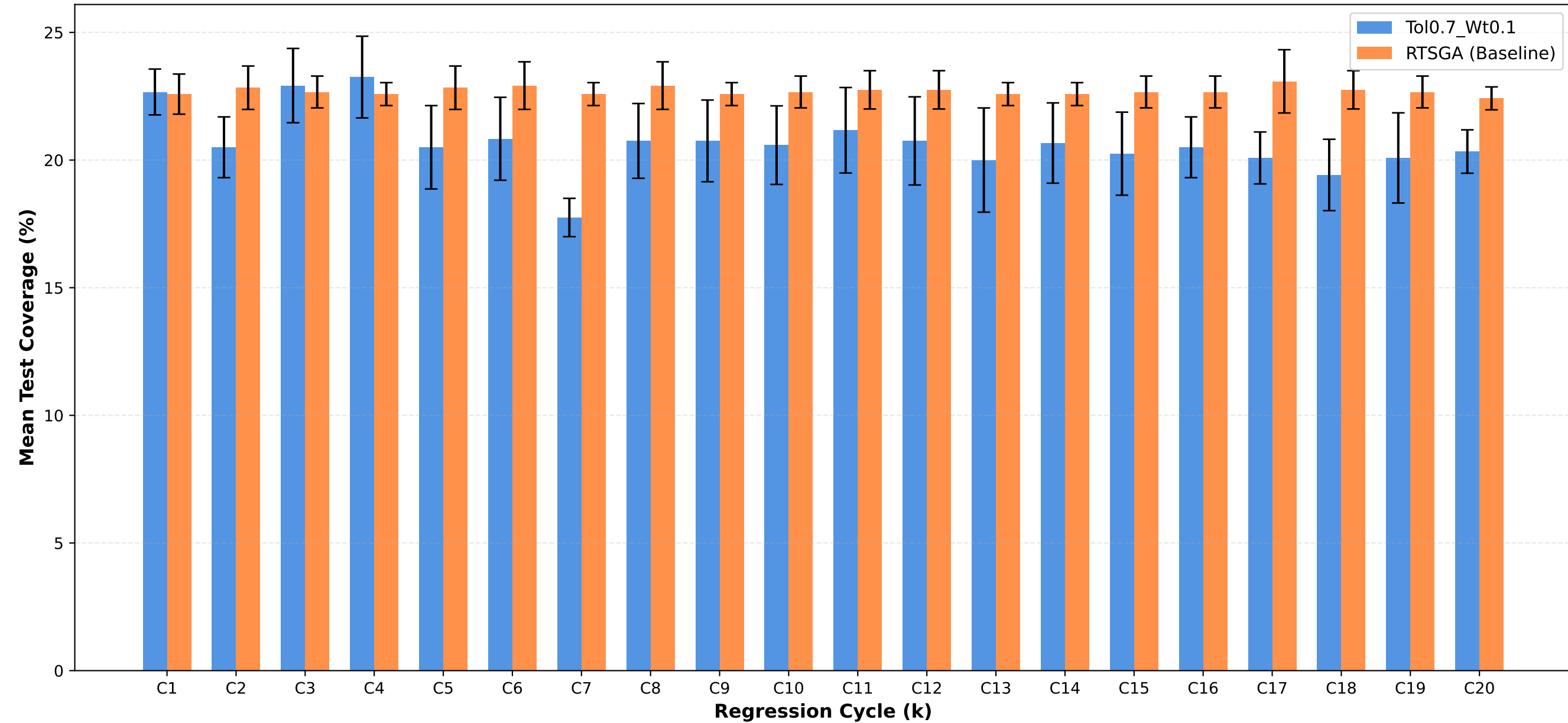
Test Coverage: Tol0.7_Wt0.1 vs RTSGA
