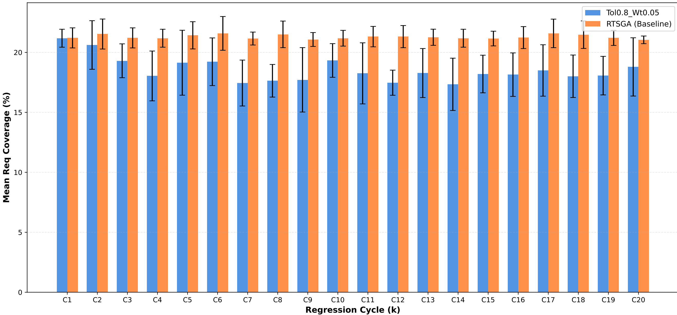
Req Coverage: Tol0.8_Wt0.05 vs RTSGA
