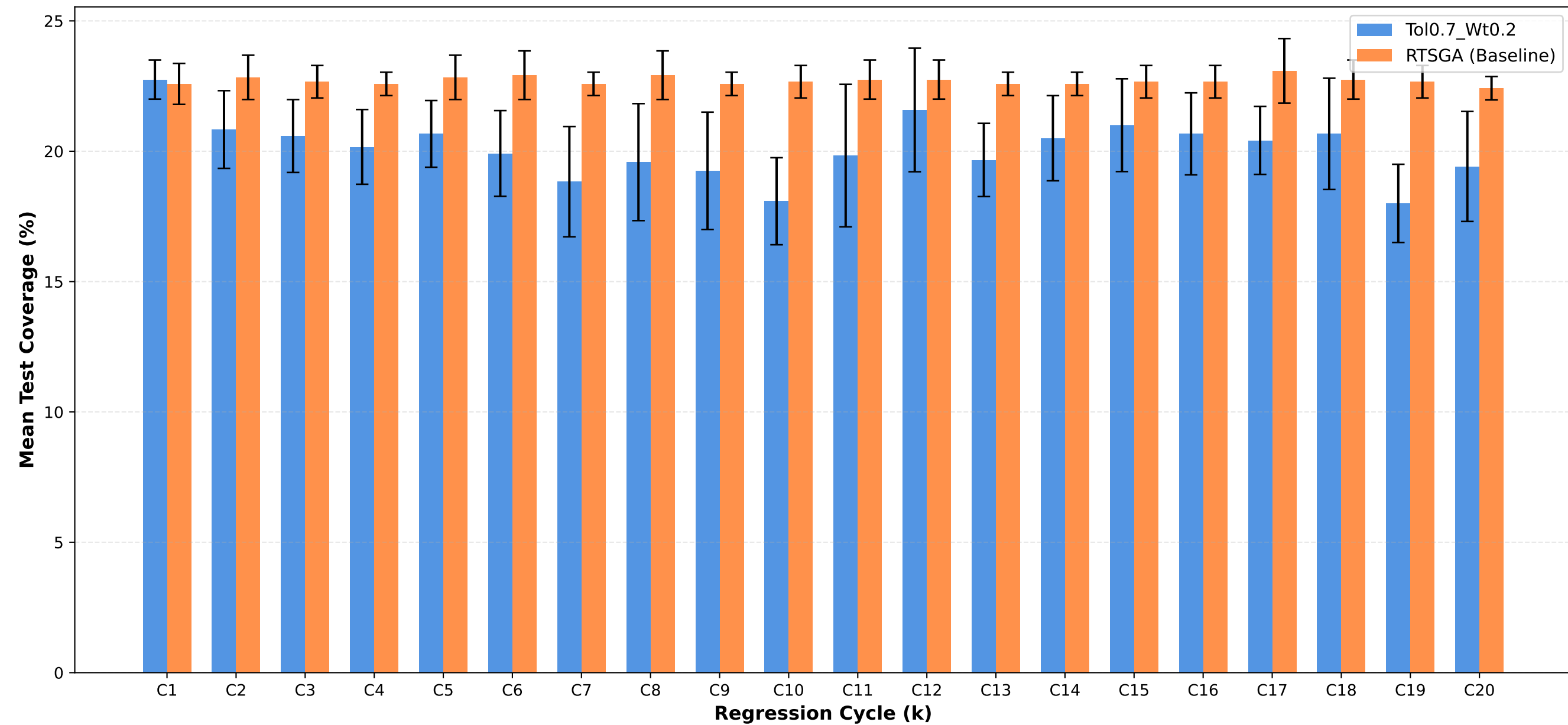
Test Coverage: Tol0.7_Wt0.2 vs RTSGA
