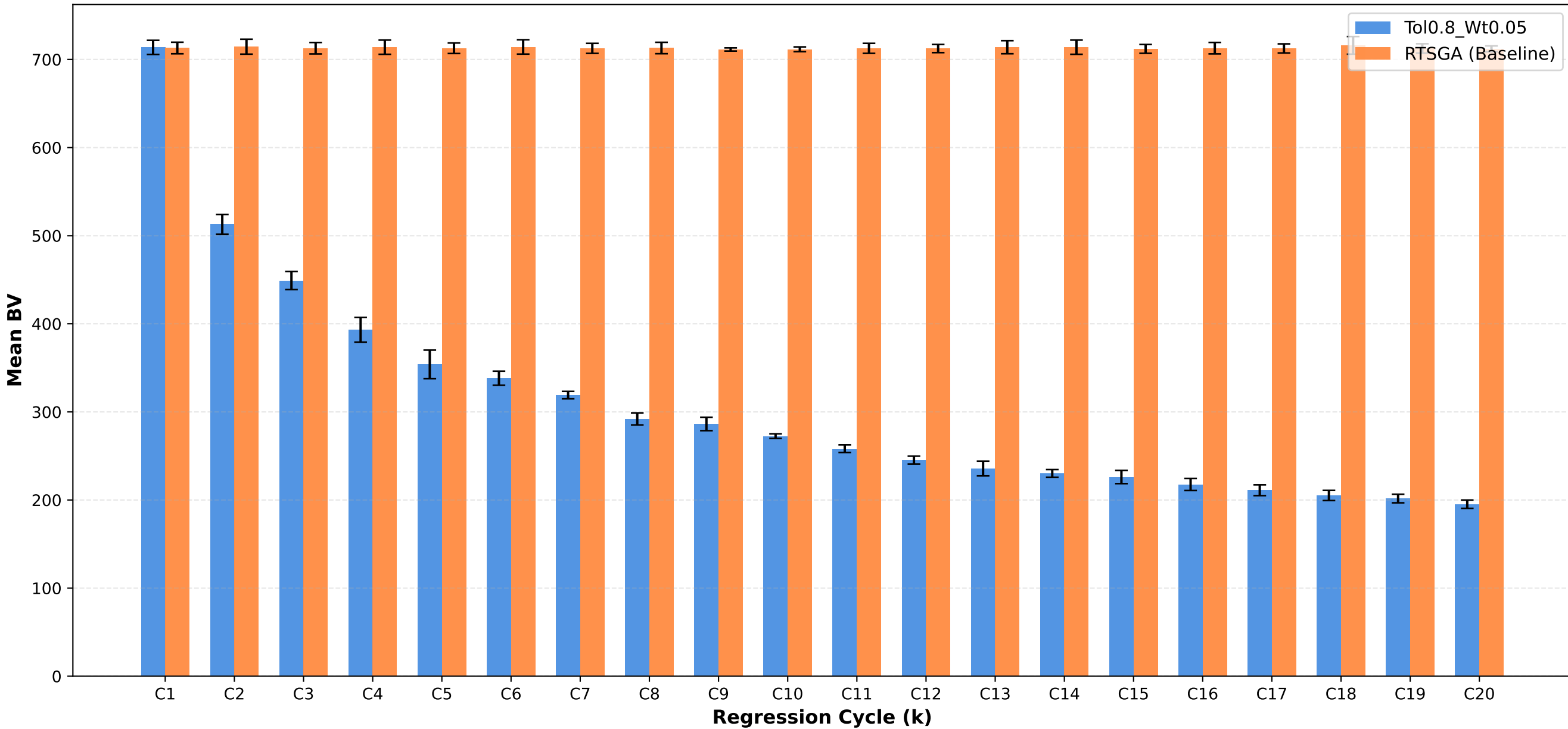
Business Value: Tol0.8_Wt0.05 vs RTSGA
