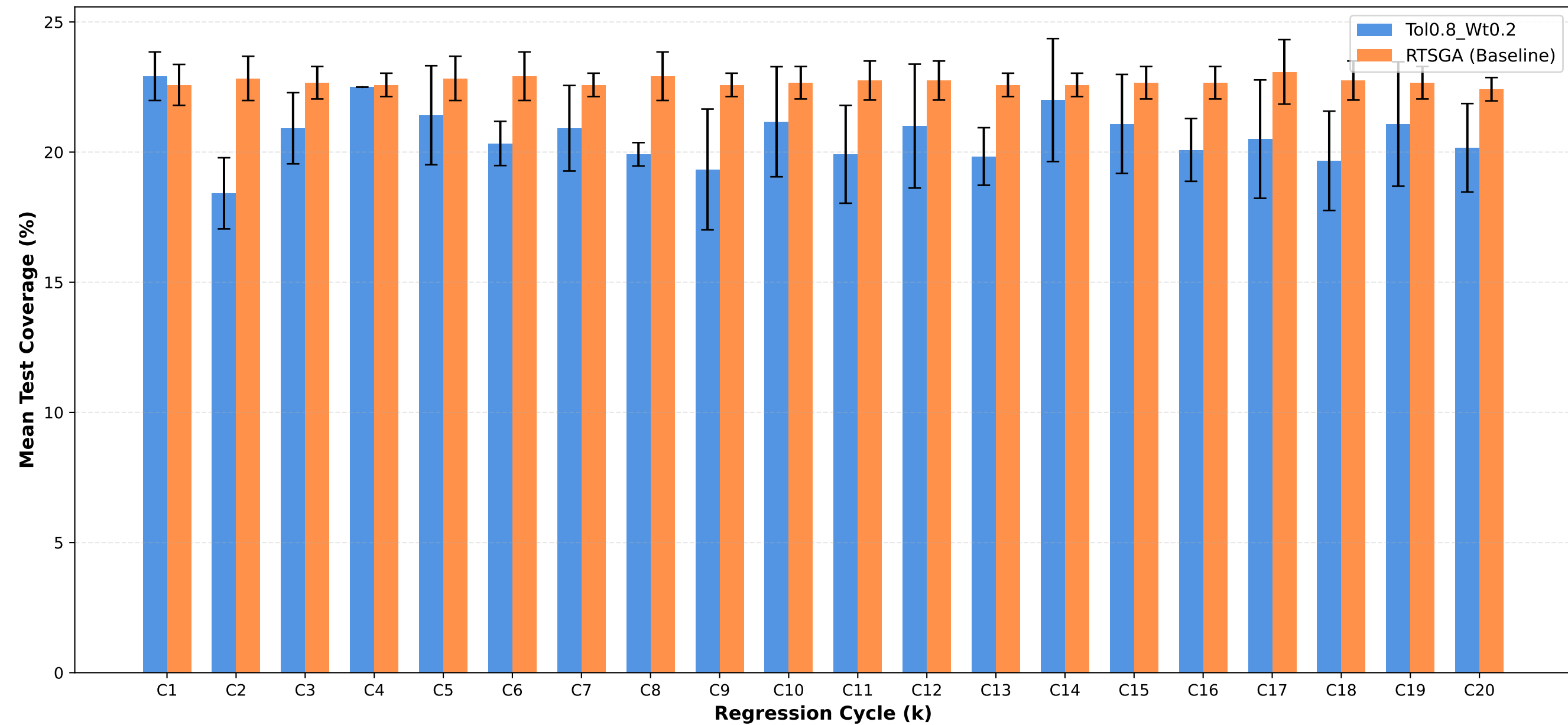
Test Coverage: Tol0.8_Wt0.2 vs RTSGA
