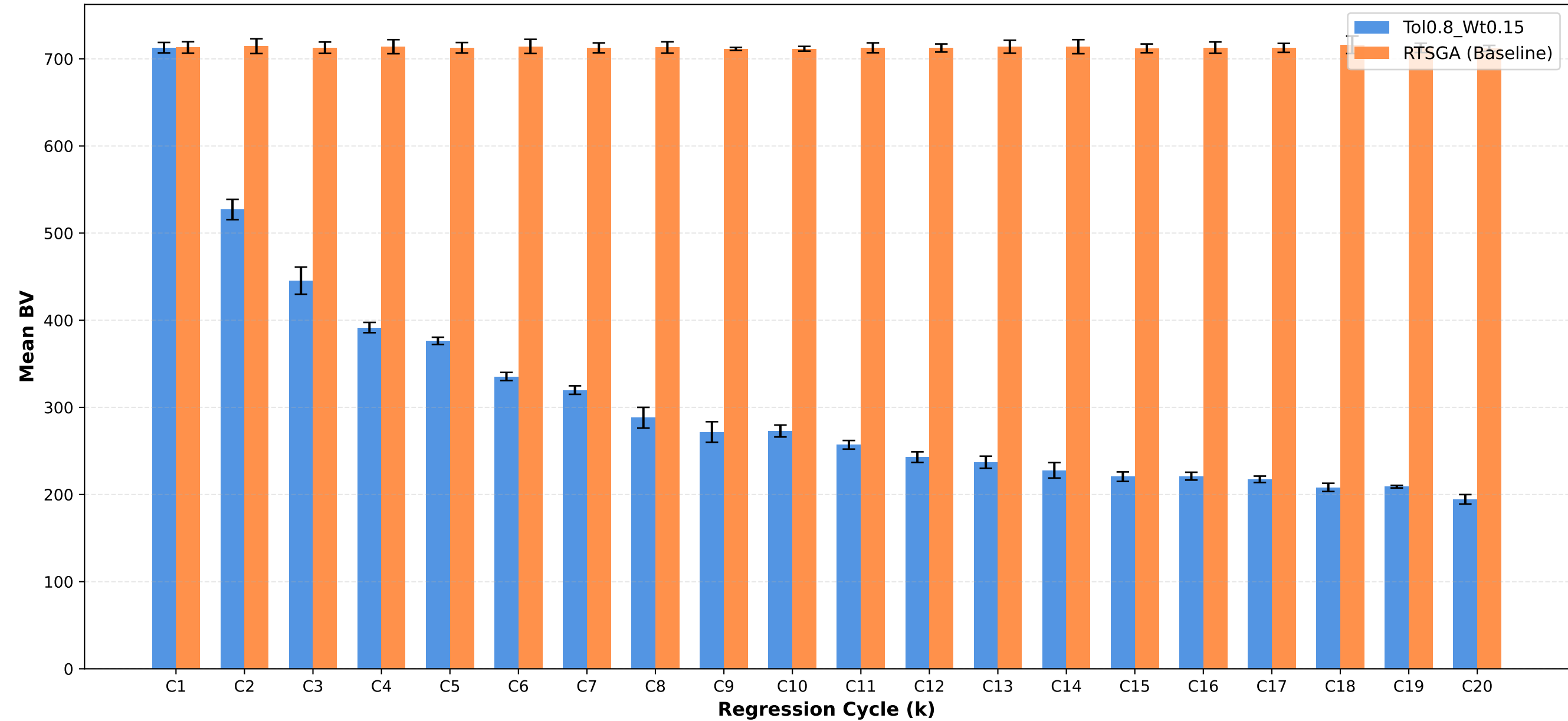
Business Value: Tol0.8_Wt0.15 vs RTSGA
