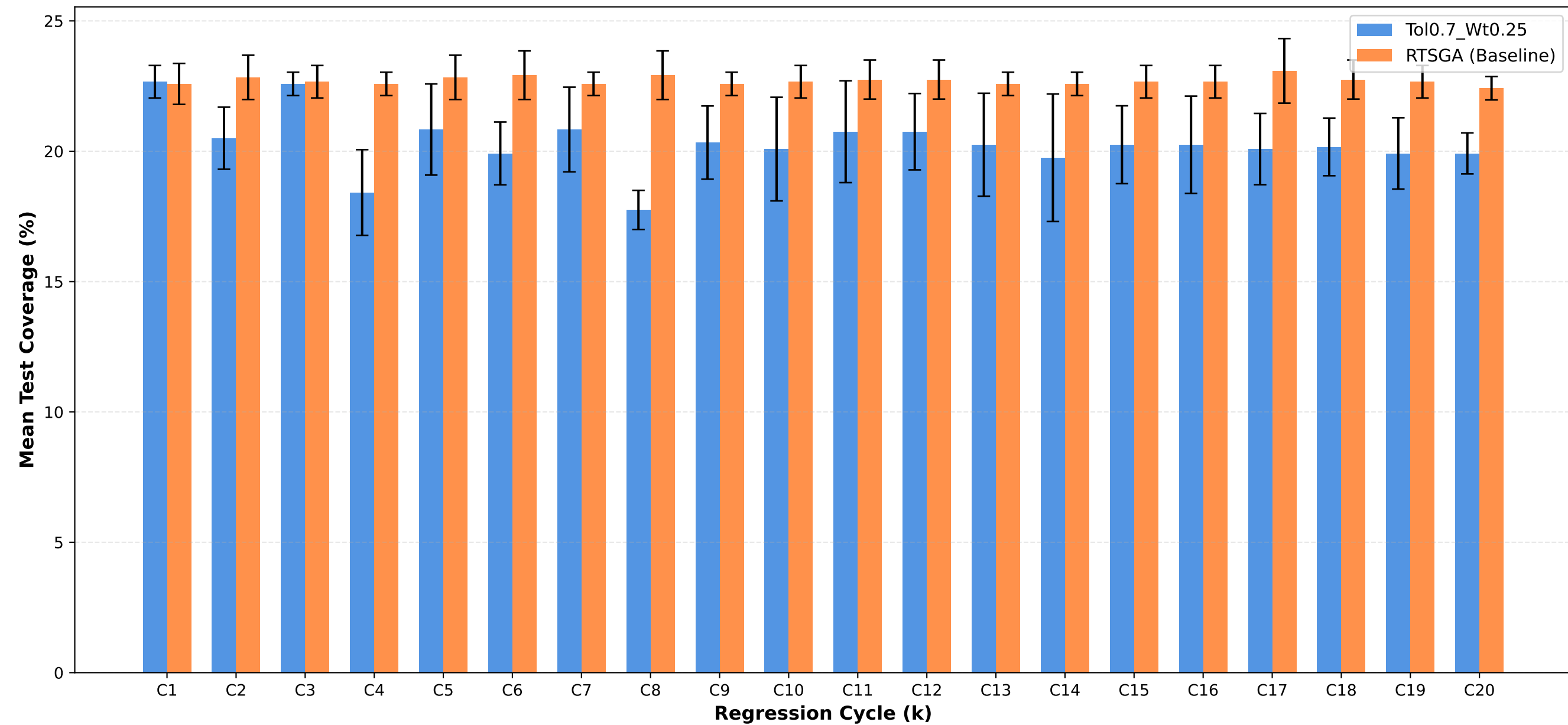
Test Coverage: Tol0.7_Wt0.25 vs RTSGA
