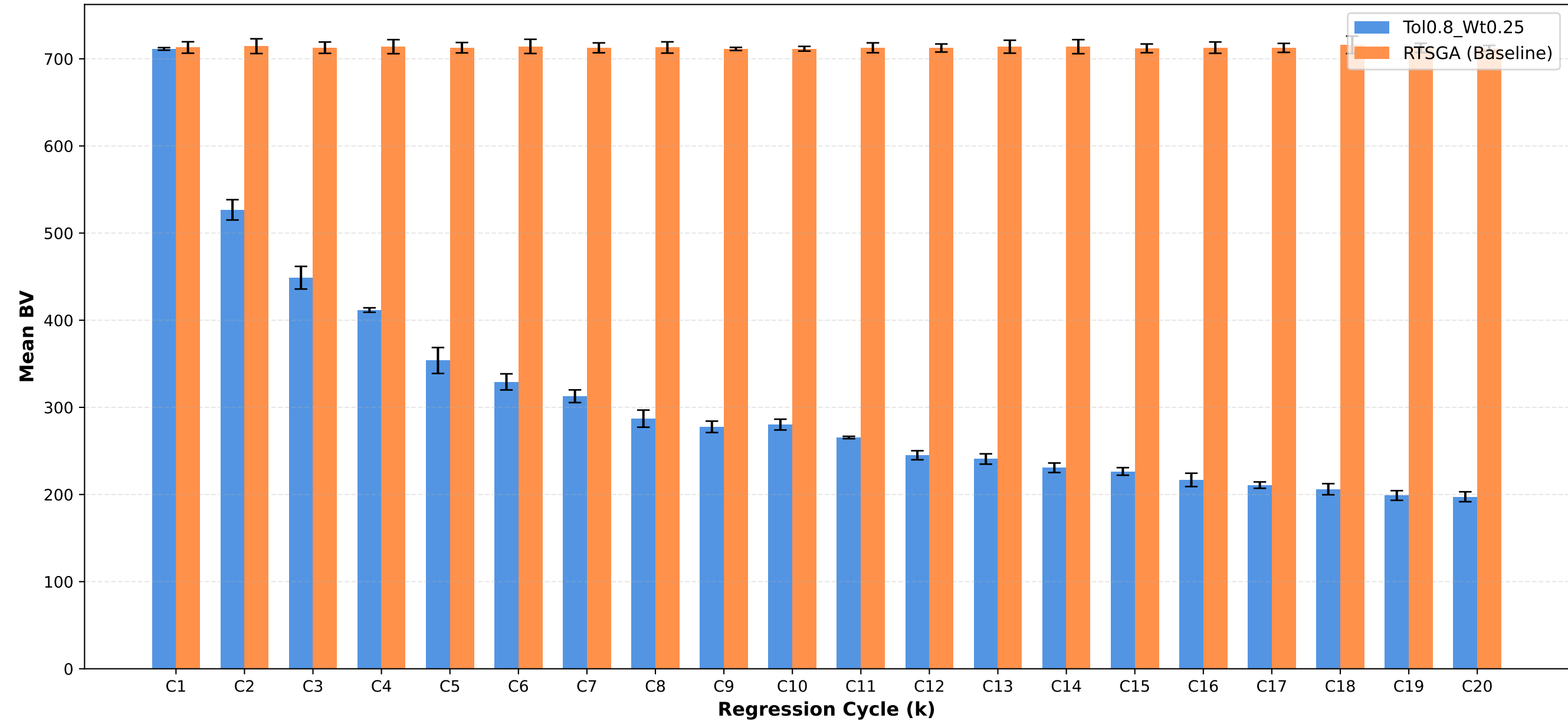
Business Value: Tol0.8_Wt0.25 vs RTSGA
