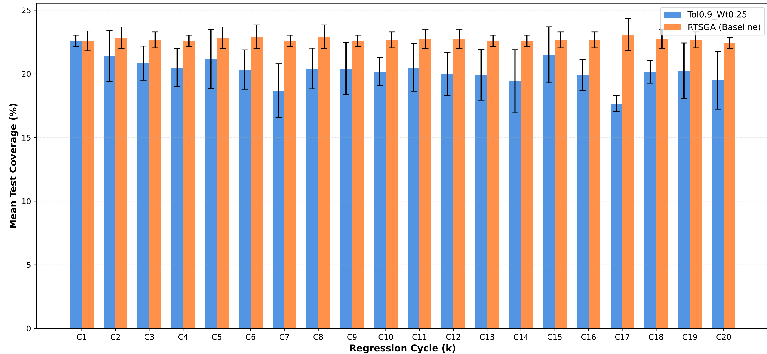
Test Coverage: Tol0.9_Wt0.25 vs RTSGA
