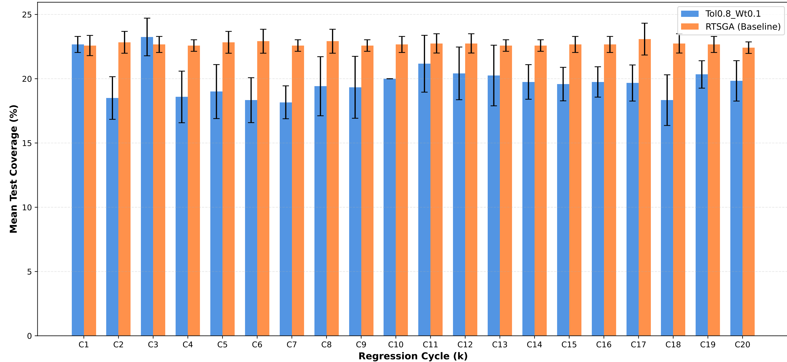
Test Coverage: Tol0.8_Wt0.1 vs RTSGA
