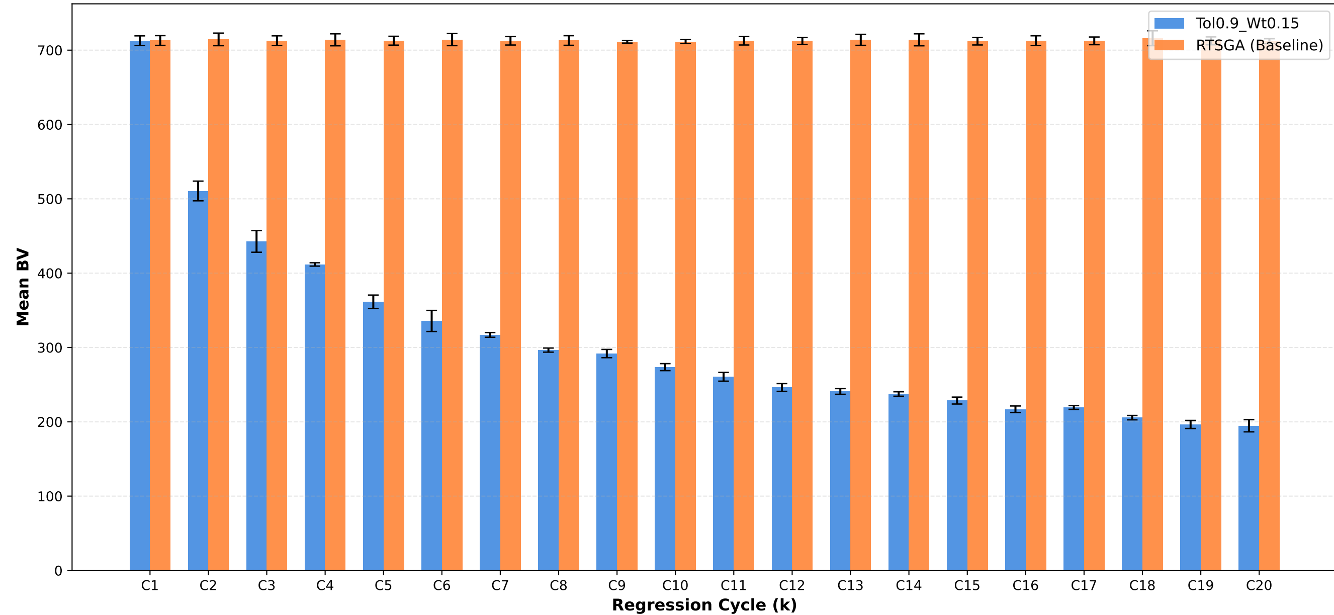
Business Value: Tol0.9_Wt0.15 vs RTSGA
