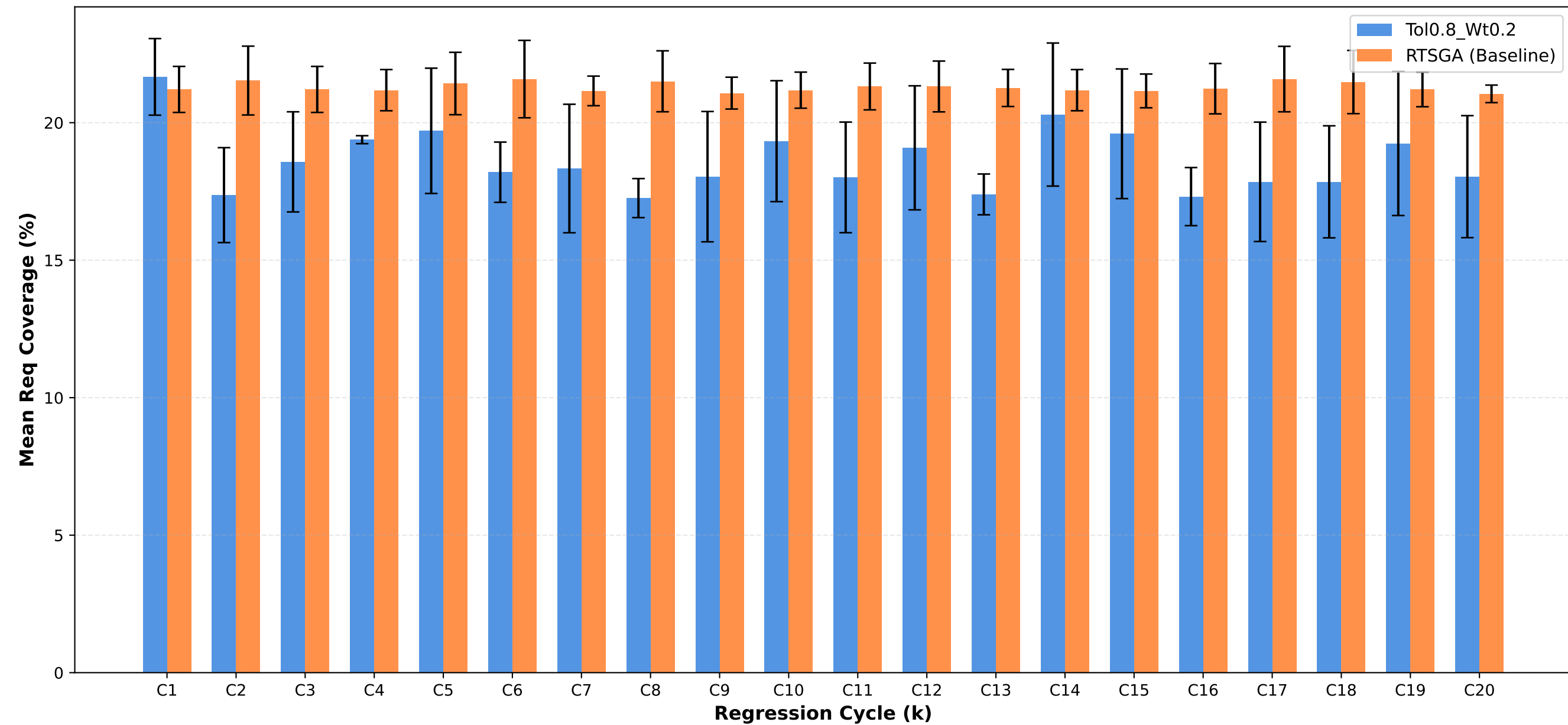
Req Coverage: Tol0.8_Wt0.2 vs RTSGA
