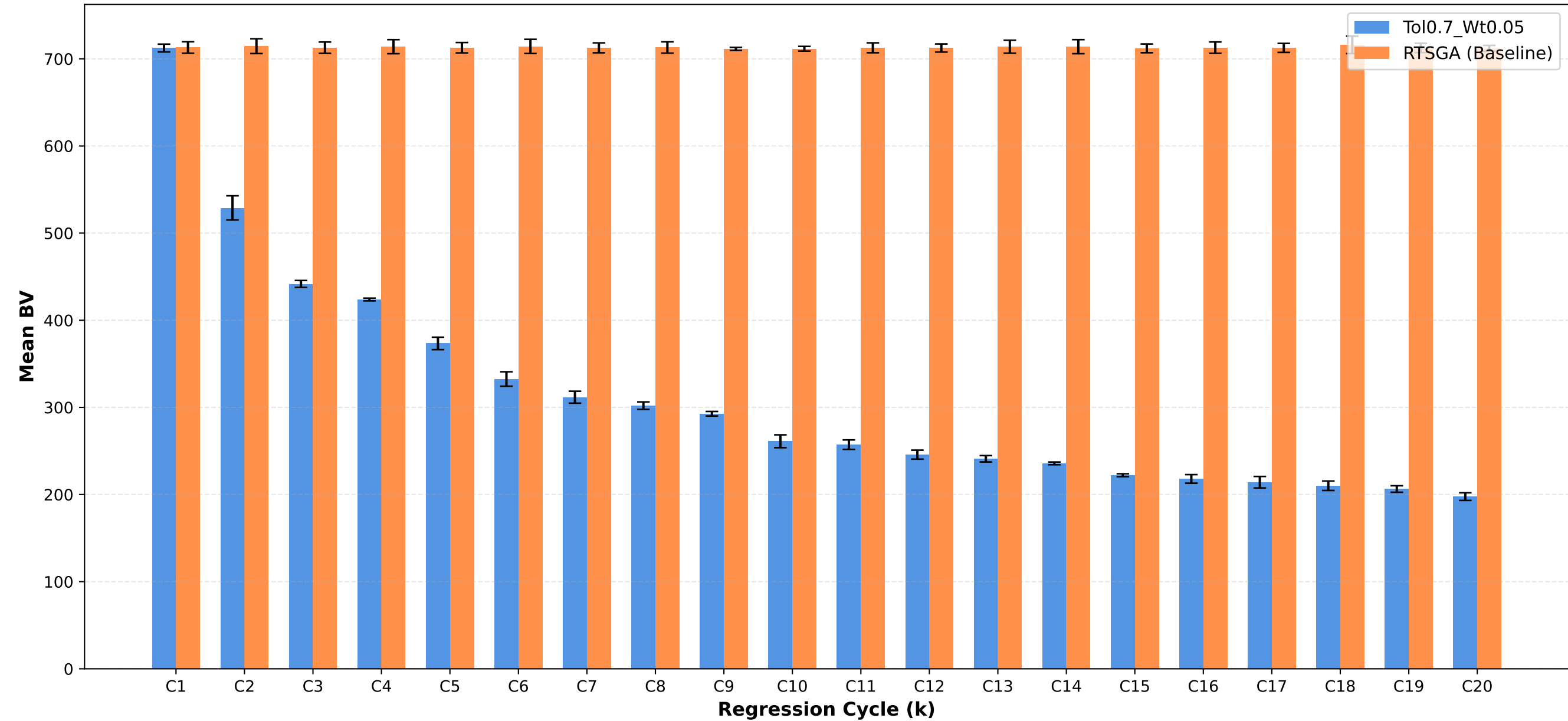
Business Value: Tol0.7_Wt0.05 vs RTSGA
