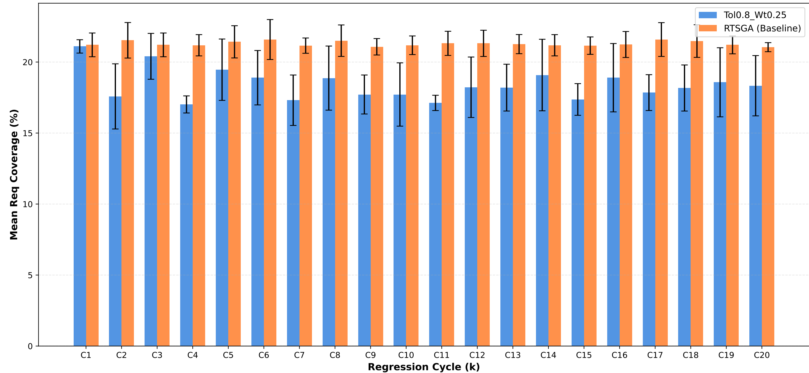
Req Coverage: Tol0.8_Wt0.25 vs RTSGA
