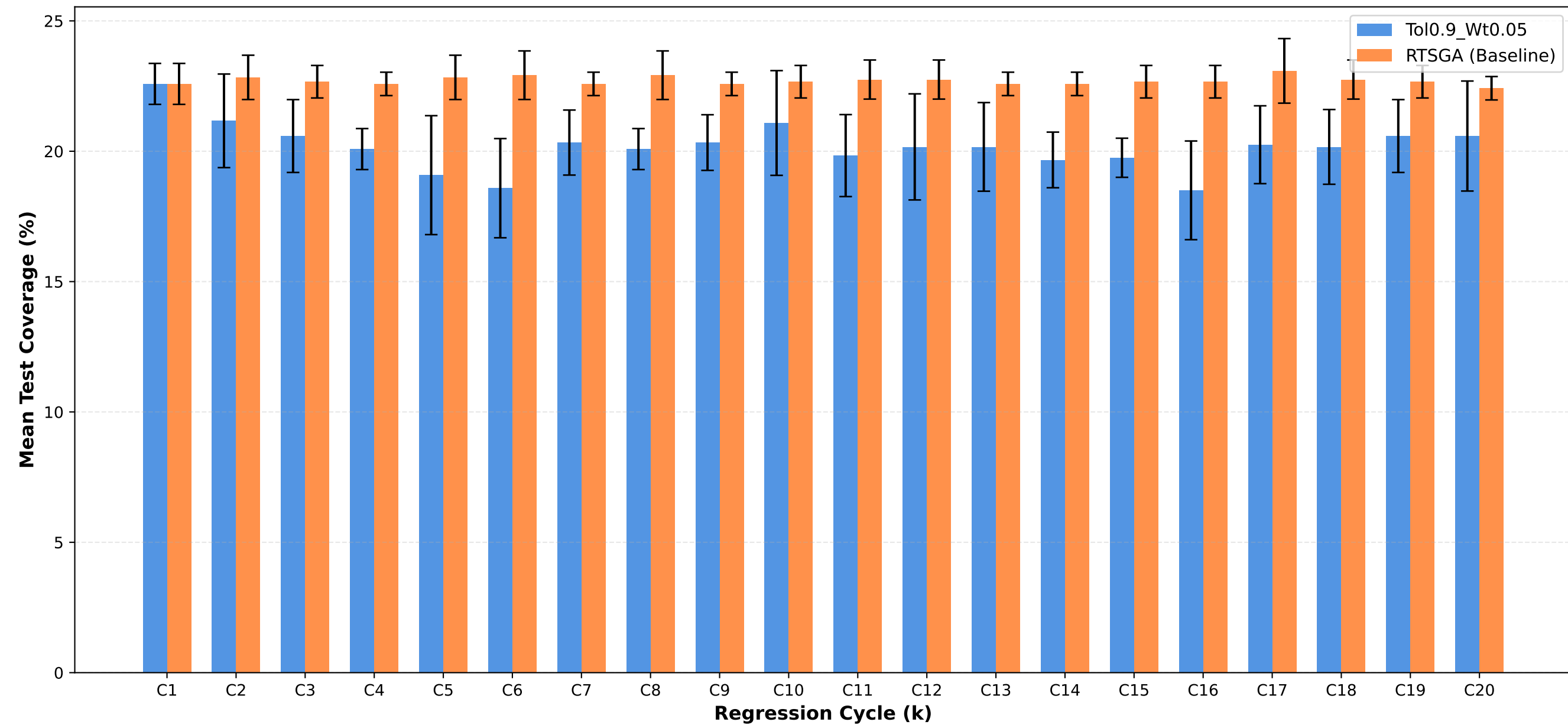
Test Coverage: Tol0.9_Wt0.05 vs RTSGA
