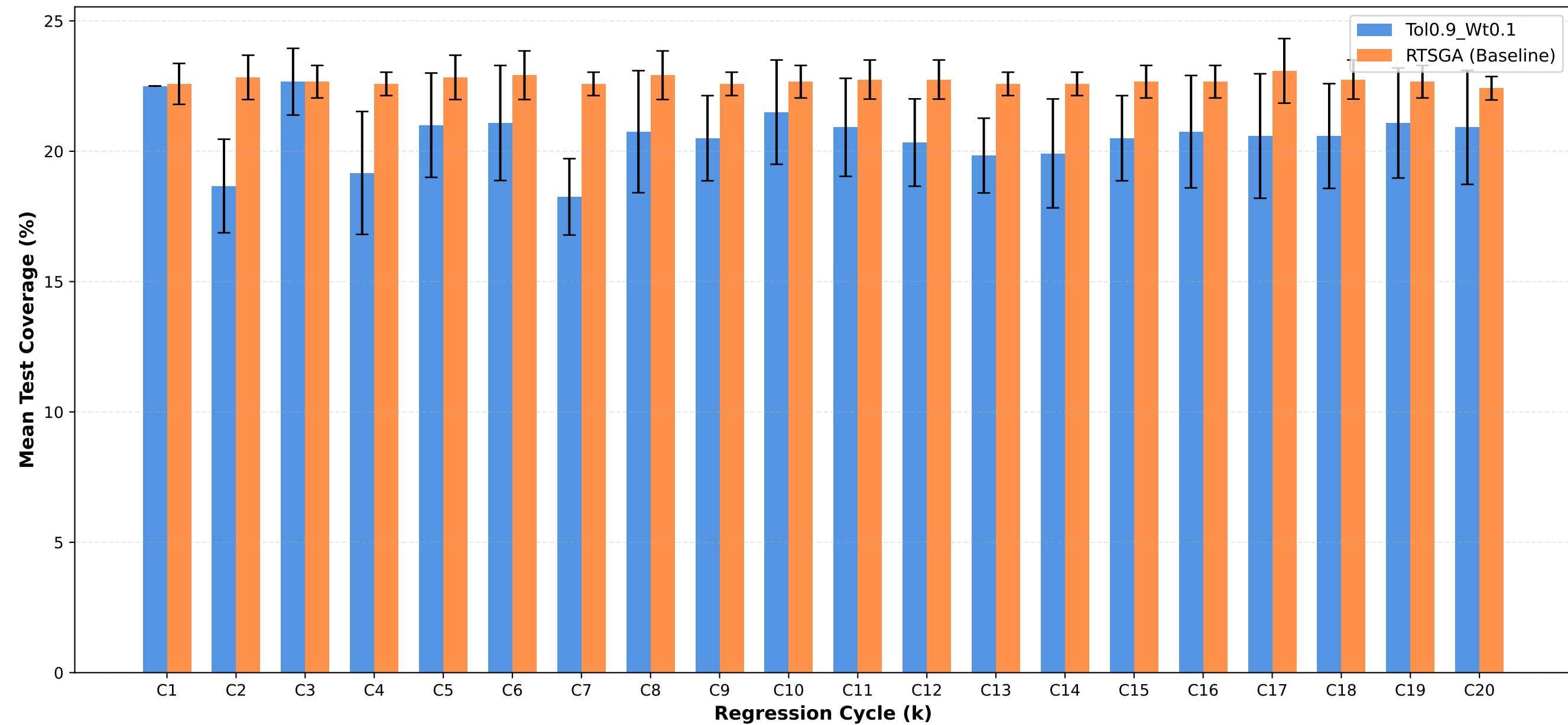
Test Coverage: Tol0.9_Wt0.1 vs RTSGA
