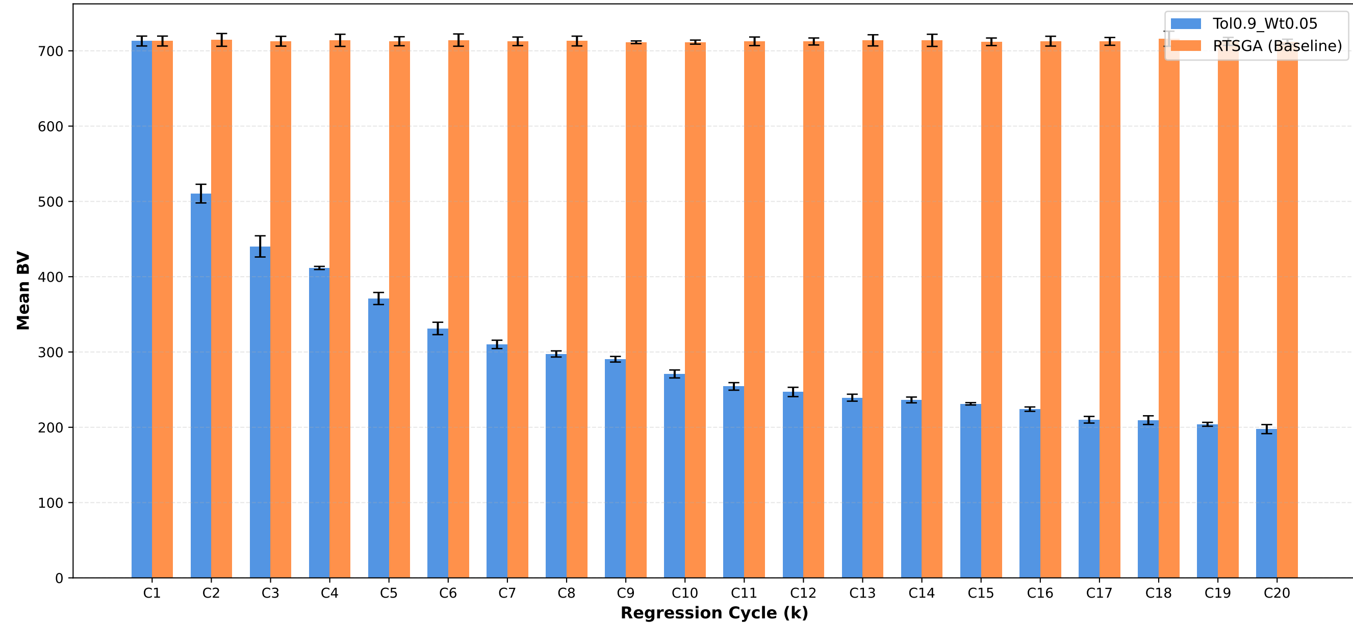
Business Value: Tol0.9_Wt0.05 vs RTSGA
