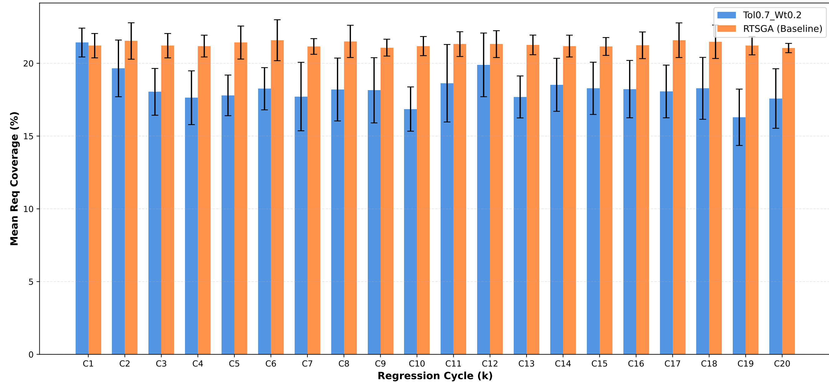
Req Coverage: Tol0.7_Wt0.2 vs RTSGA
