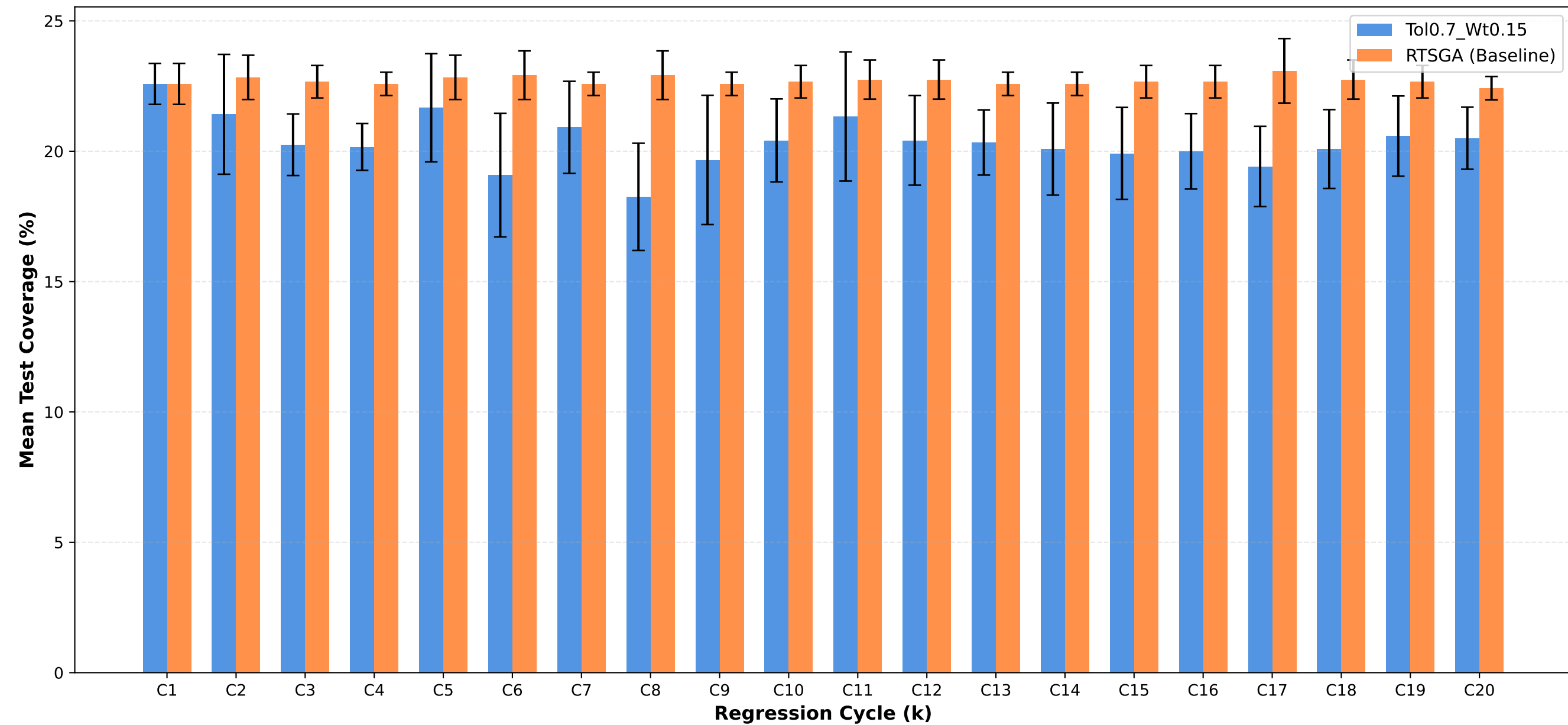
Test Coverage: Tol0.7_Wt0.15 vs RTSGA
