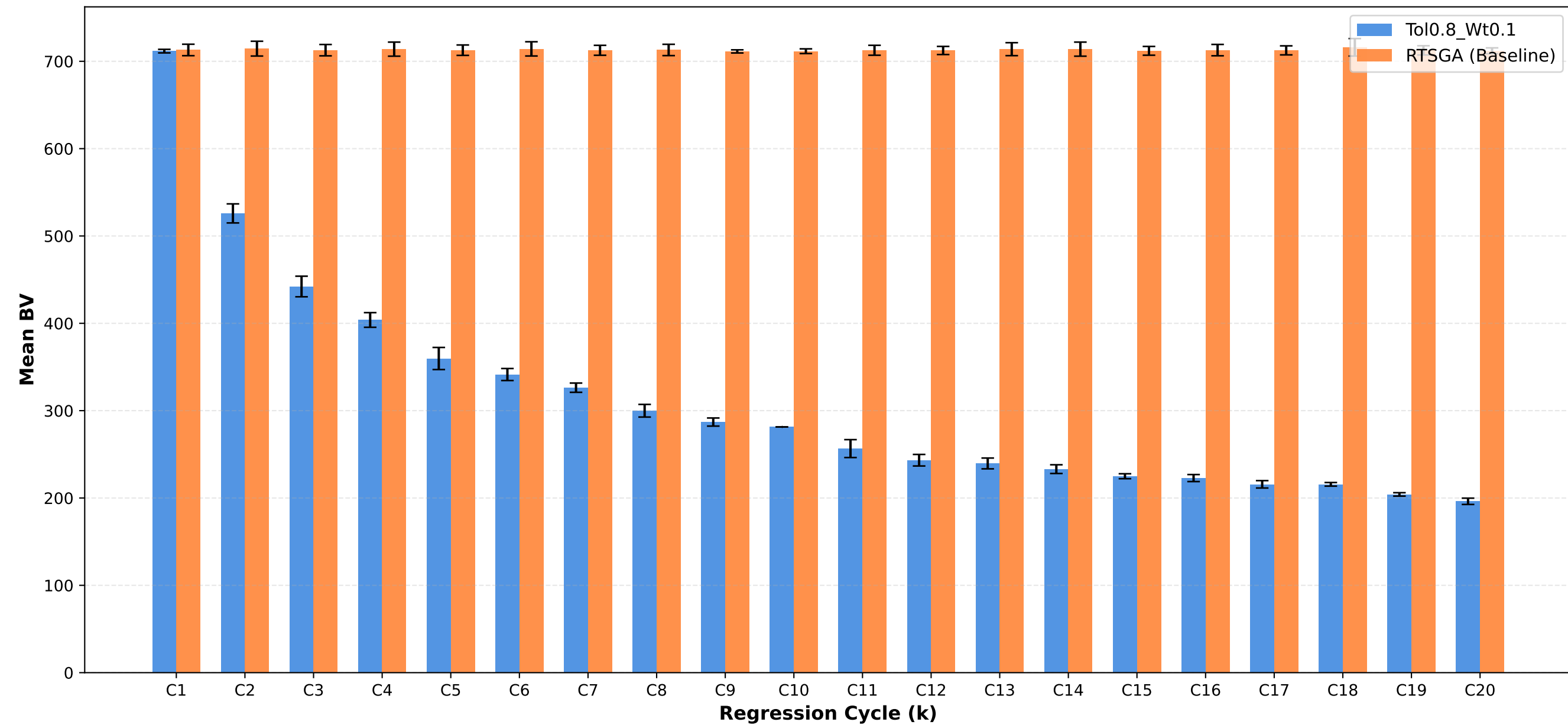
Business Value: Tol0.8_Wt0.1 vs RTSGA
