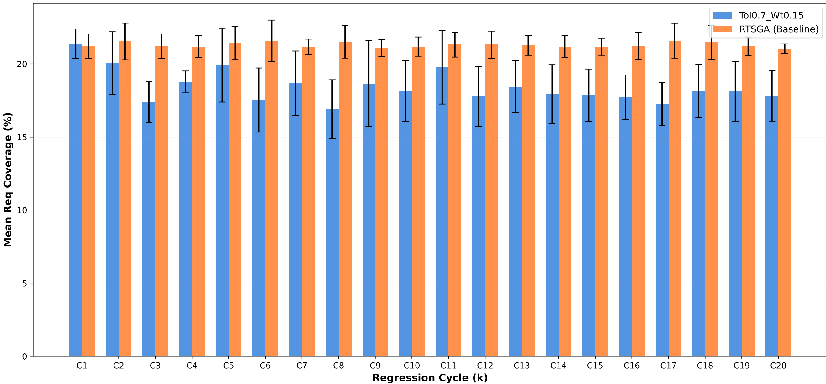
Req Coverage: Tol0.7_Wt0.15 vs RTSGA
