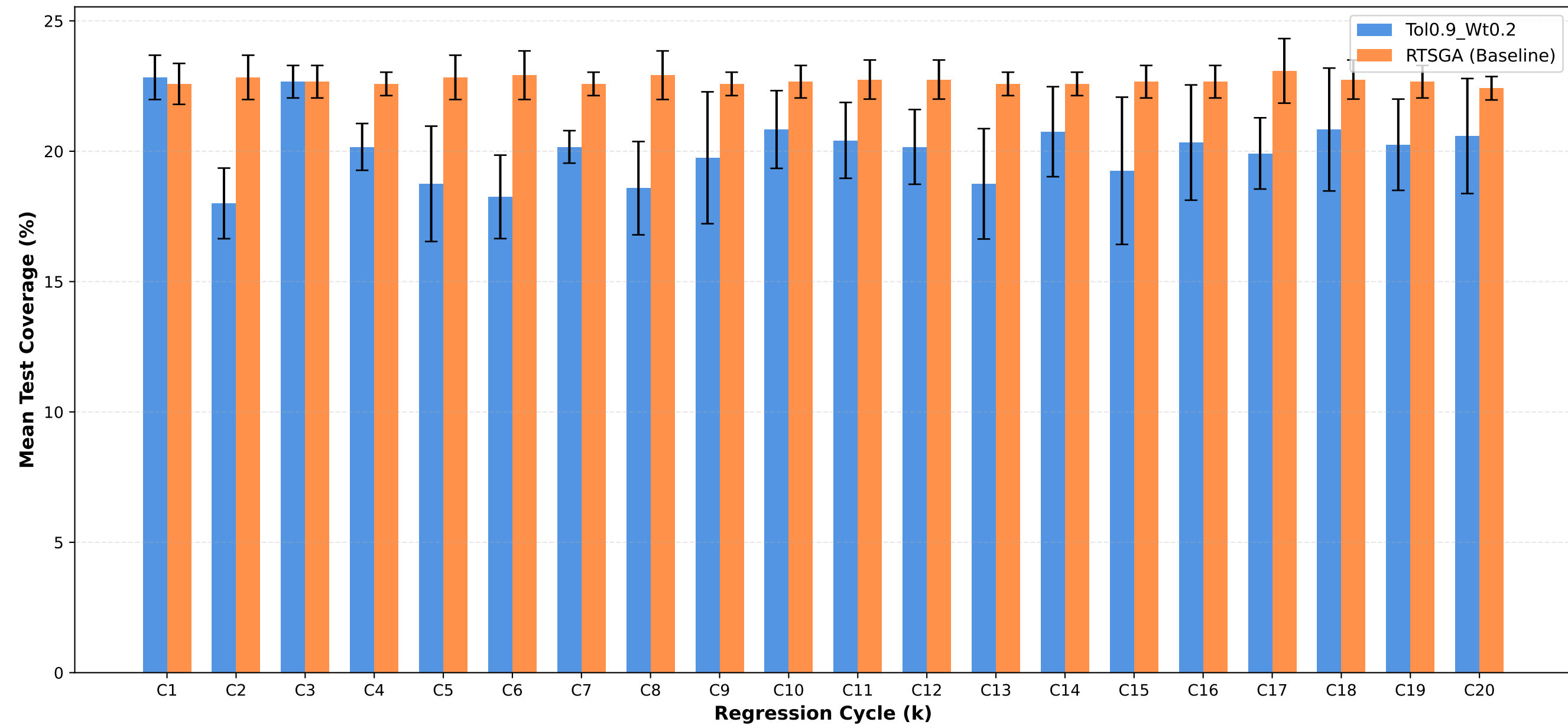
Test Coverage: Tol0.9_Wt0.2 vs RTSGA
