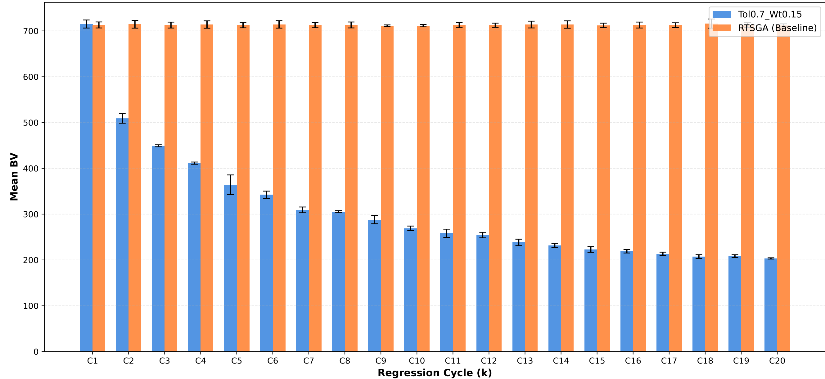
Business Value: Tol0.7_Wt0.15 vs RTSGA
