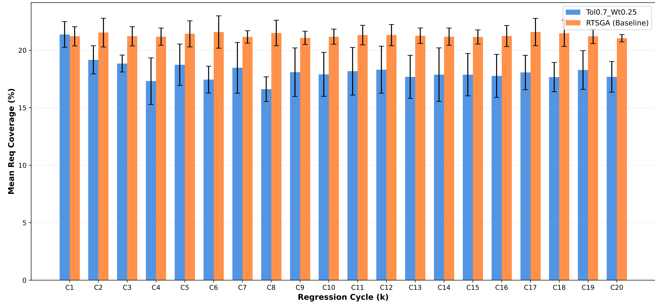
Req Coverage: Tol0.7_Wt0.25 vs RTSGA
