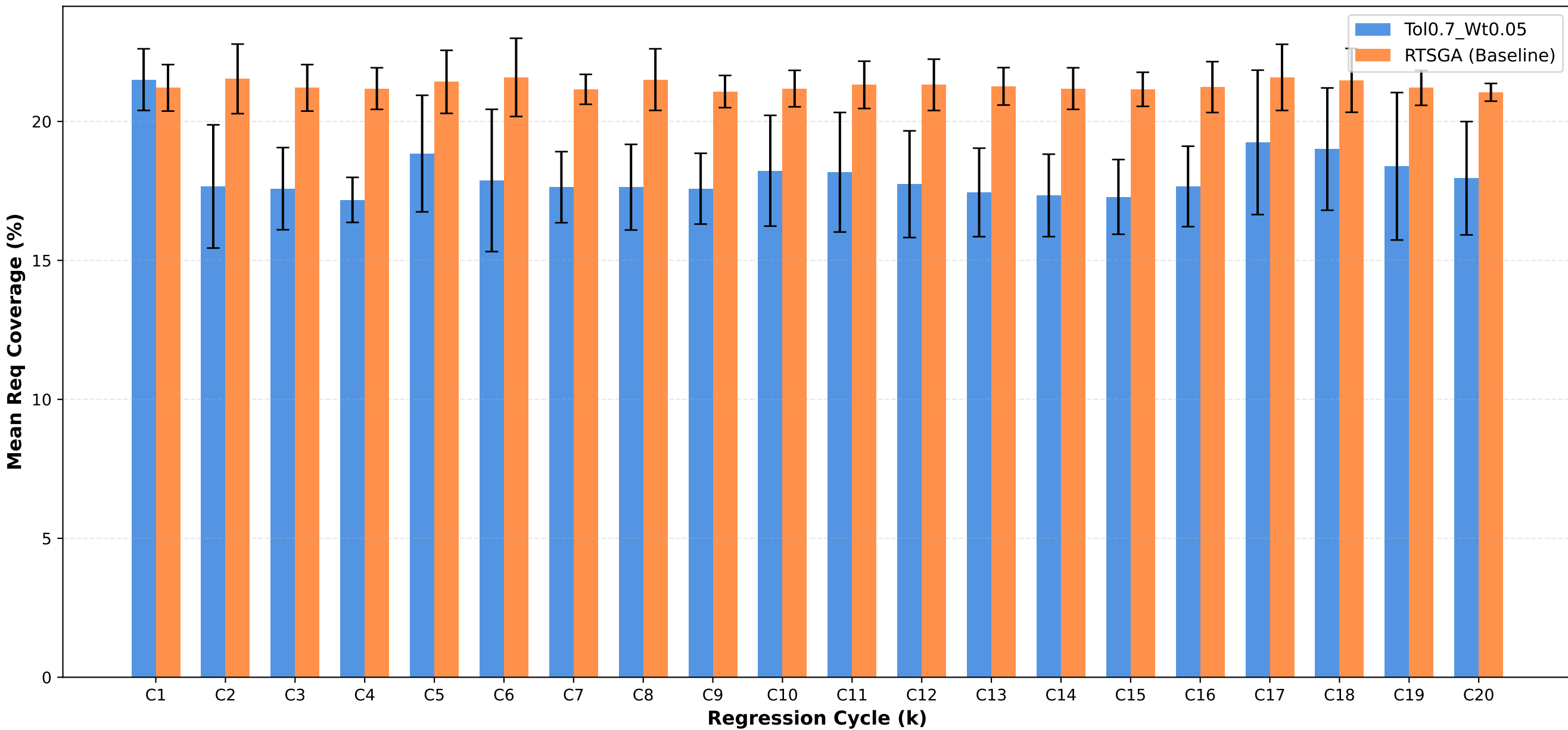
Req Coverage: Tol0.7_Wt0.05 vs RTSGA
