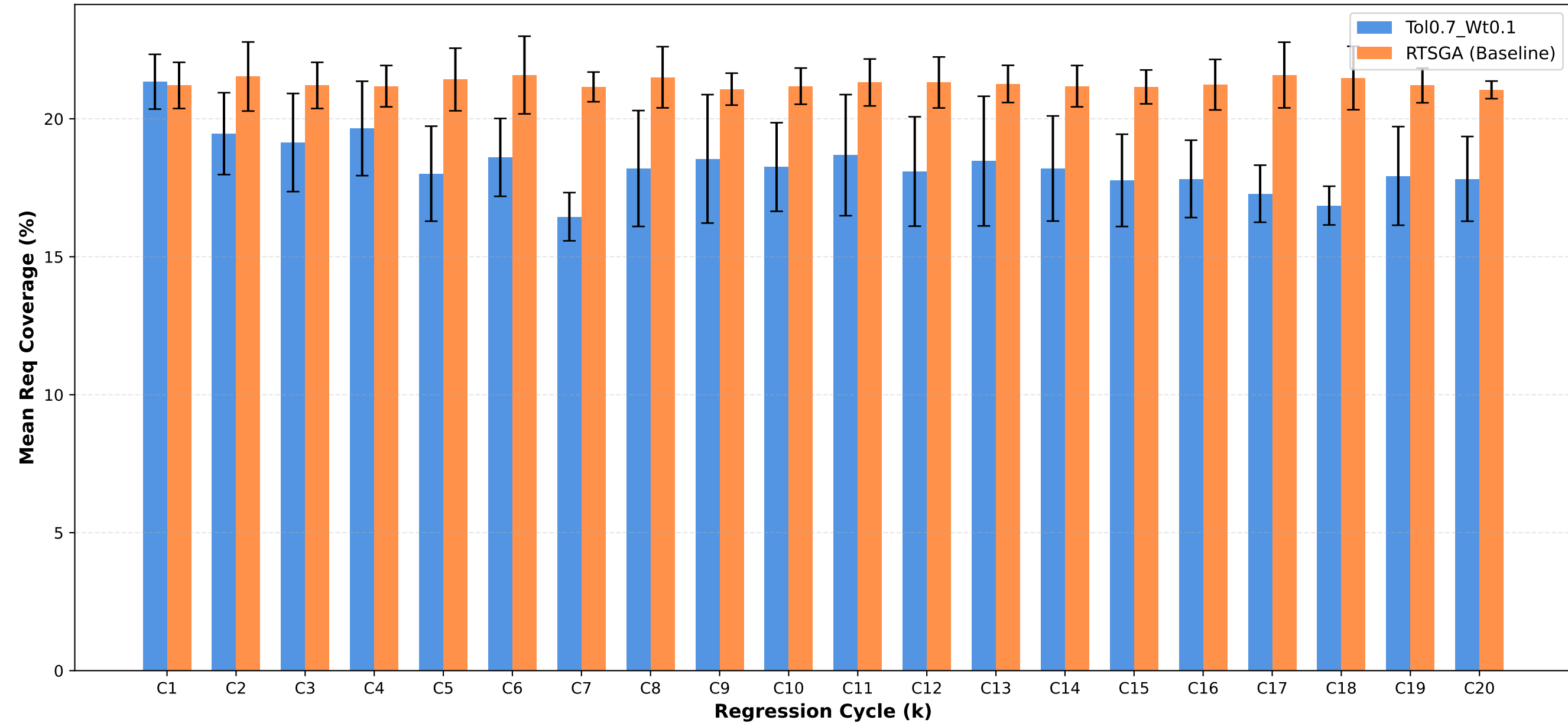
Req Coverage: Tol0.7_Wt0.1 vs RTSGA
