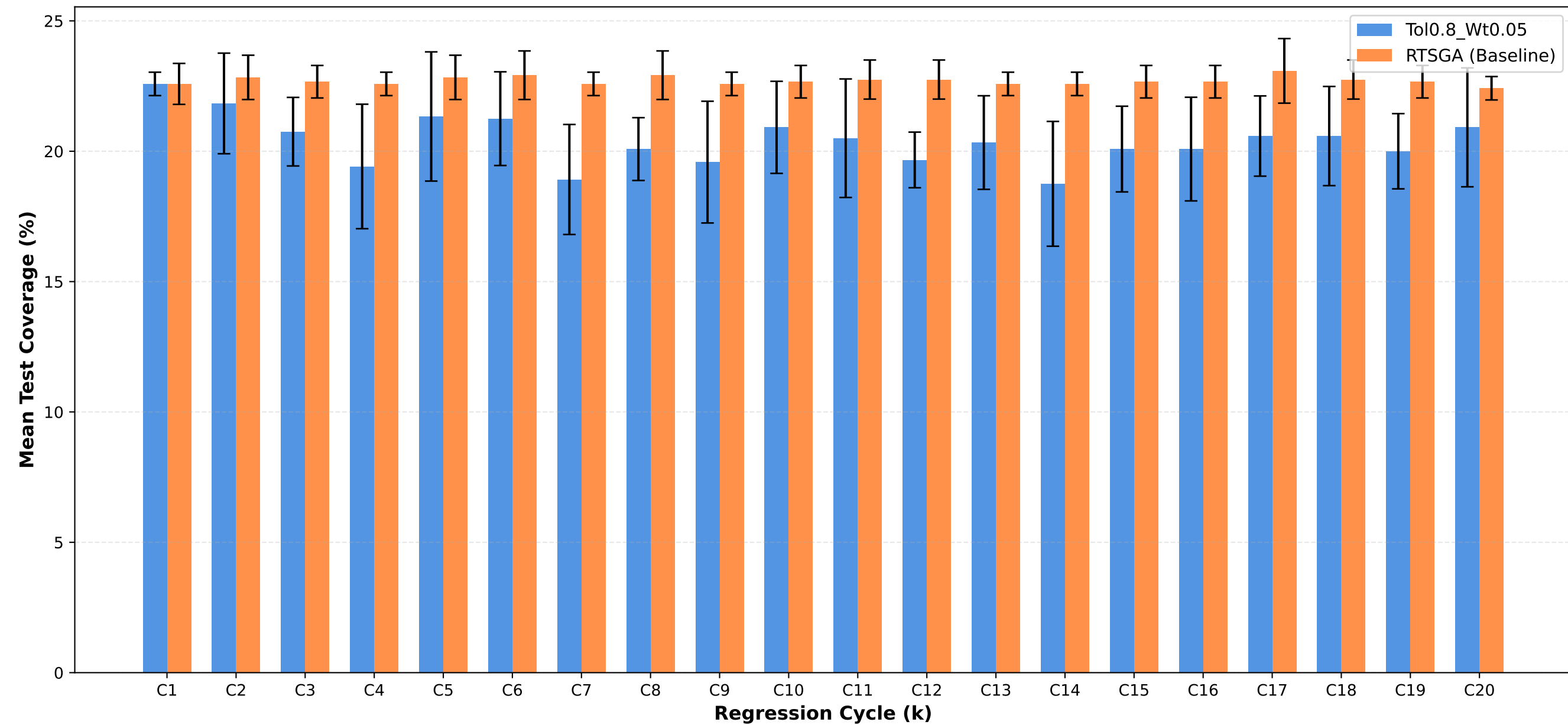
Test Coverage: Tol0.8_Wt0.05 vs RTSGA
