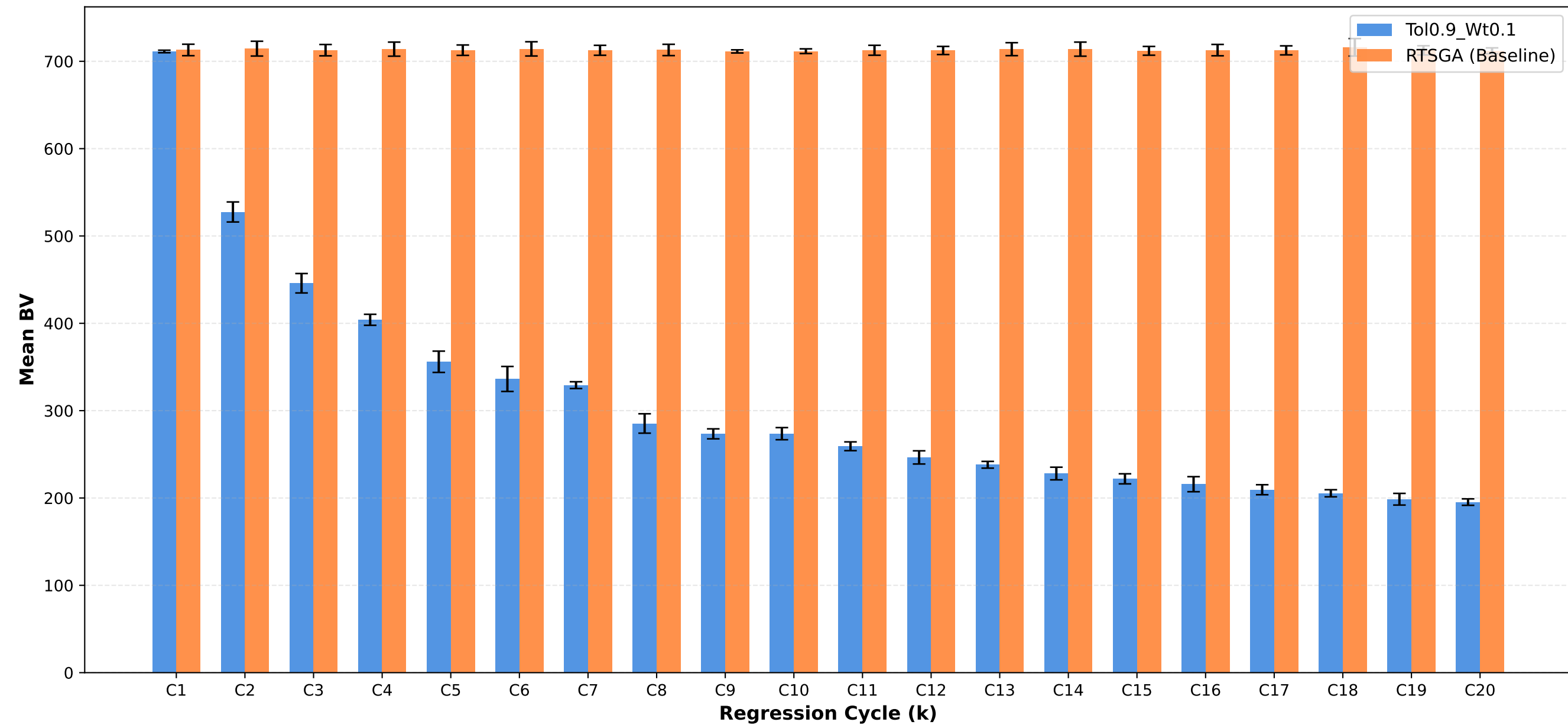
Business Value: Tol0.9_Wt0.1 vs RTSGA
