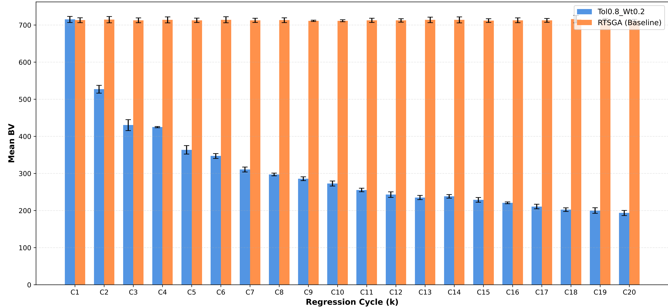
Business Value: Tol0.8_Wt0.2 vs RTSGA
