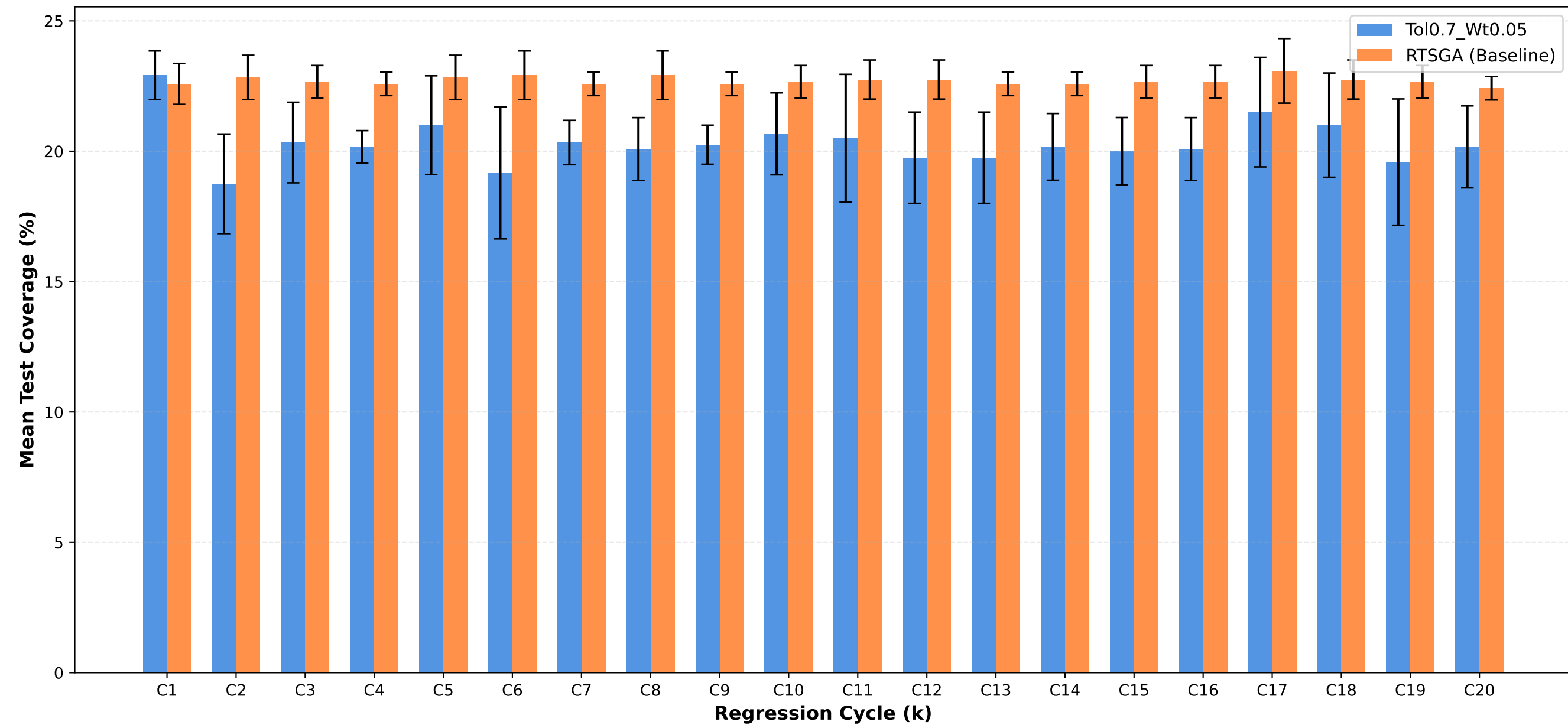
Test Coverage: Tol0.7_Wt0.05 vs RTSGA
