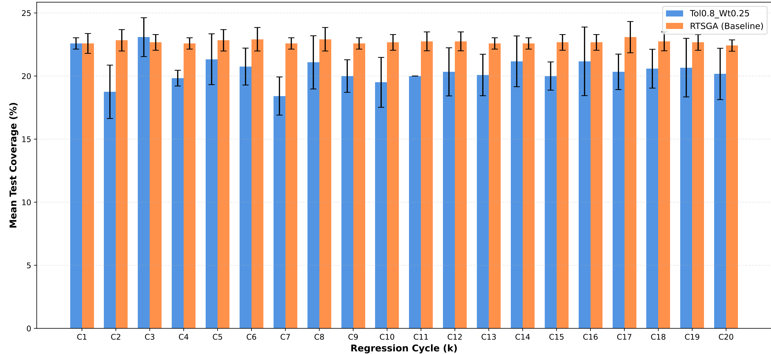
Test Coverage: Tol0.8_Wt0.25 vs RTSGA
