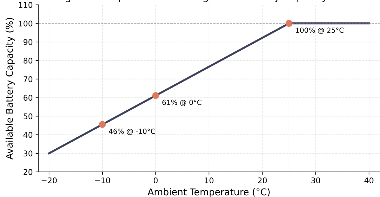
Fig 3 — Temperature Derating: Li-Po Battery Capacity Model
