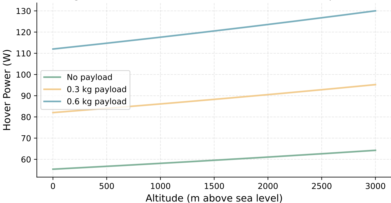
Fig 4 — Altitude Effect on Hover Power (ISA atmosphere)
