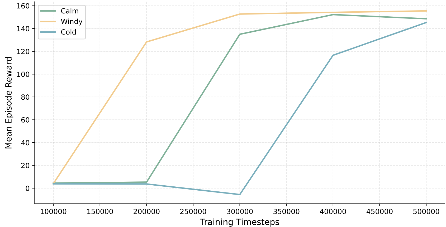
Fig 8 — PPO Training Curves by Scenario
