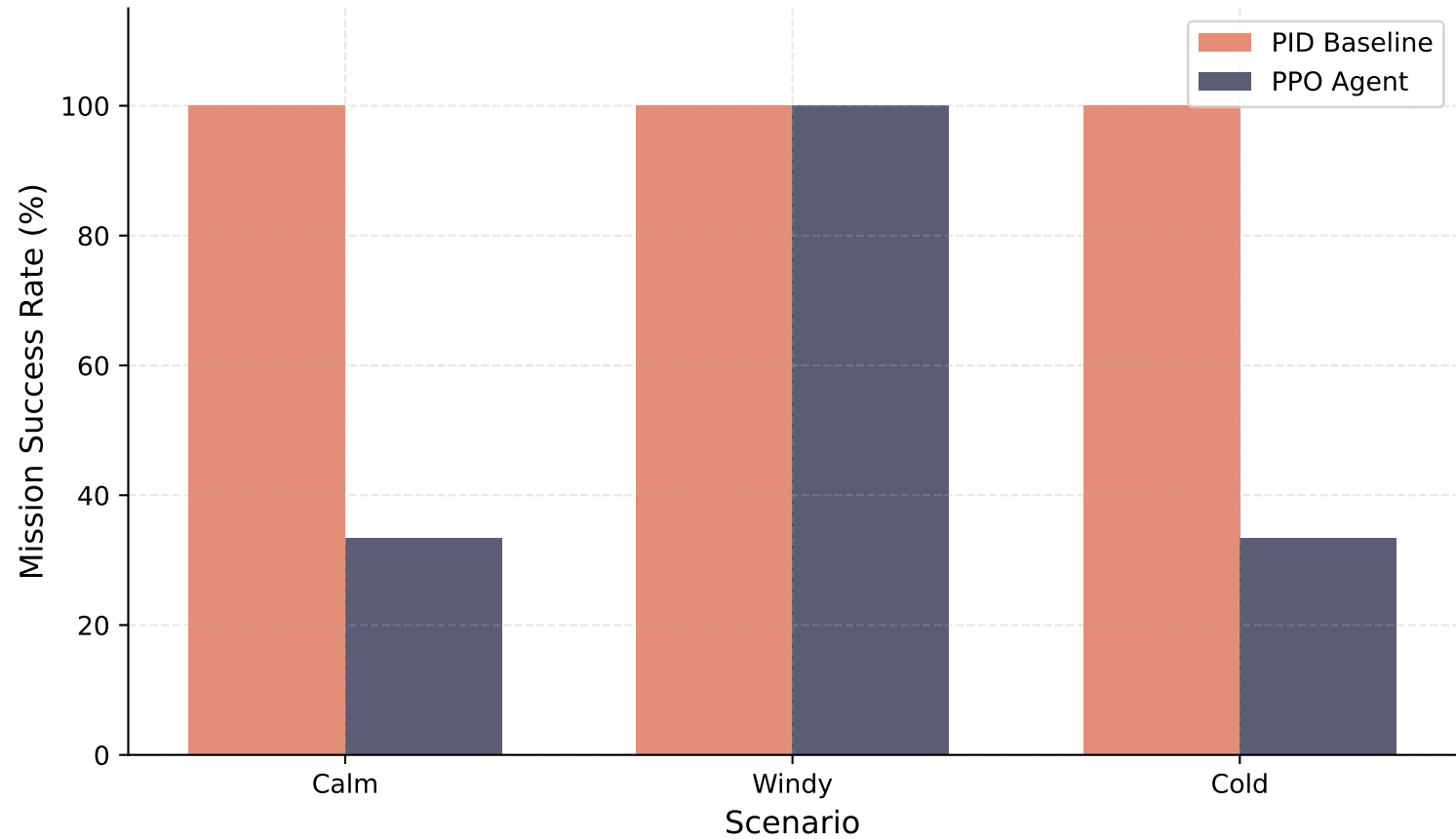
Fig 2 — Mission Success Rate: PID vs. PPO
