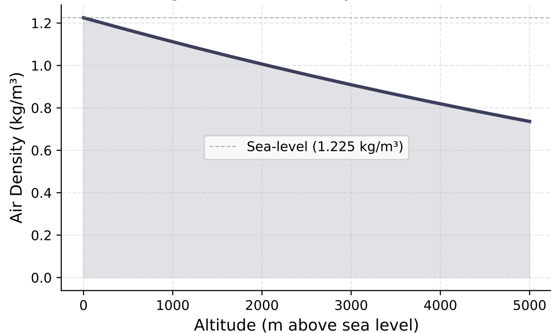
Fig 5 — ISA Air Density vs. Altitude
