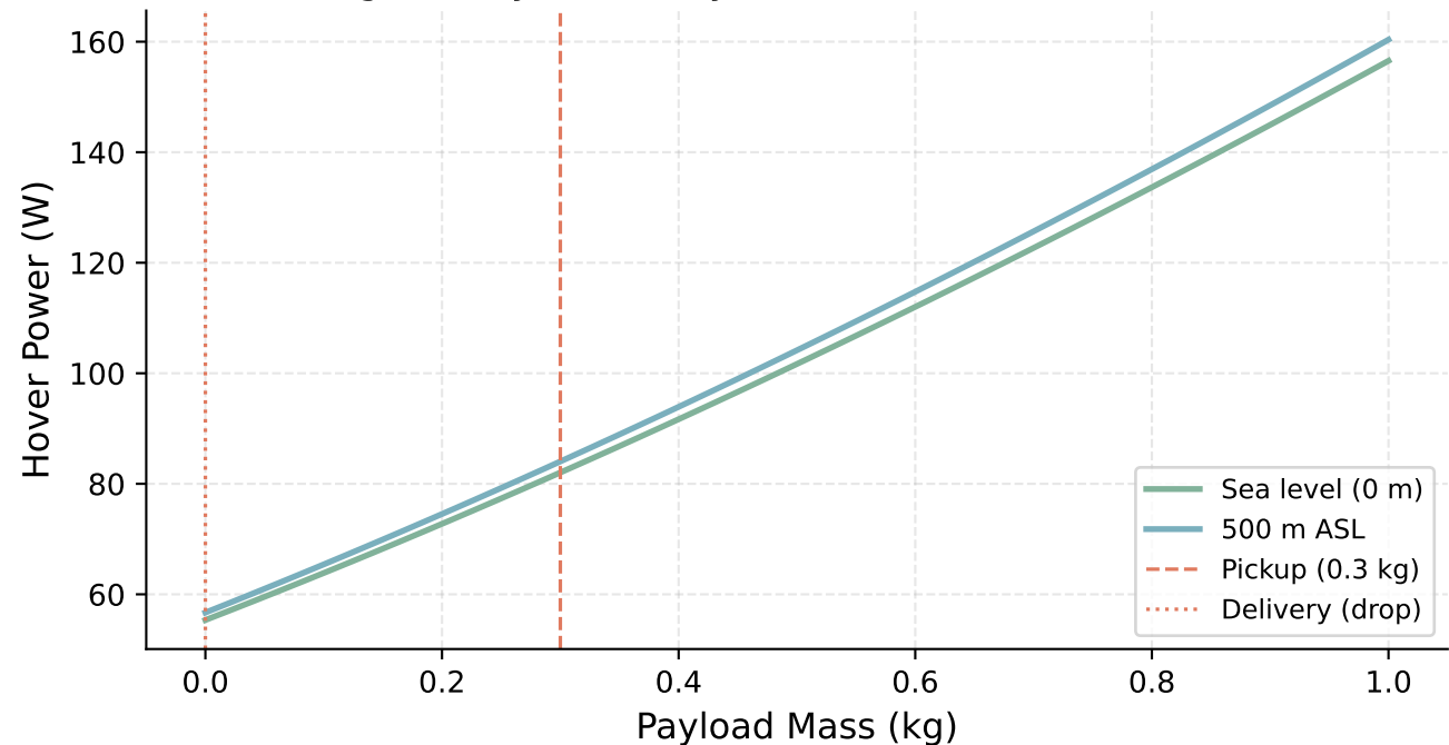
Fig 6 — Dynamic Payload: Effect on Hover Power
