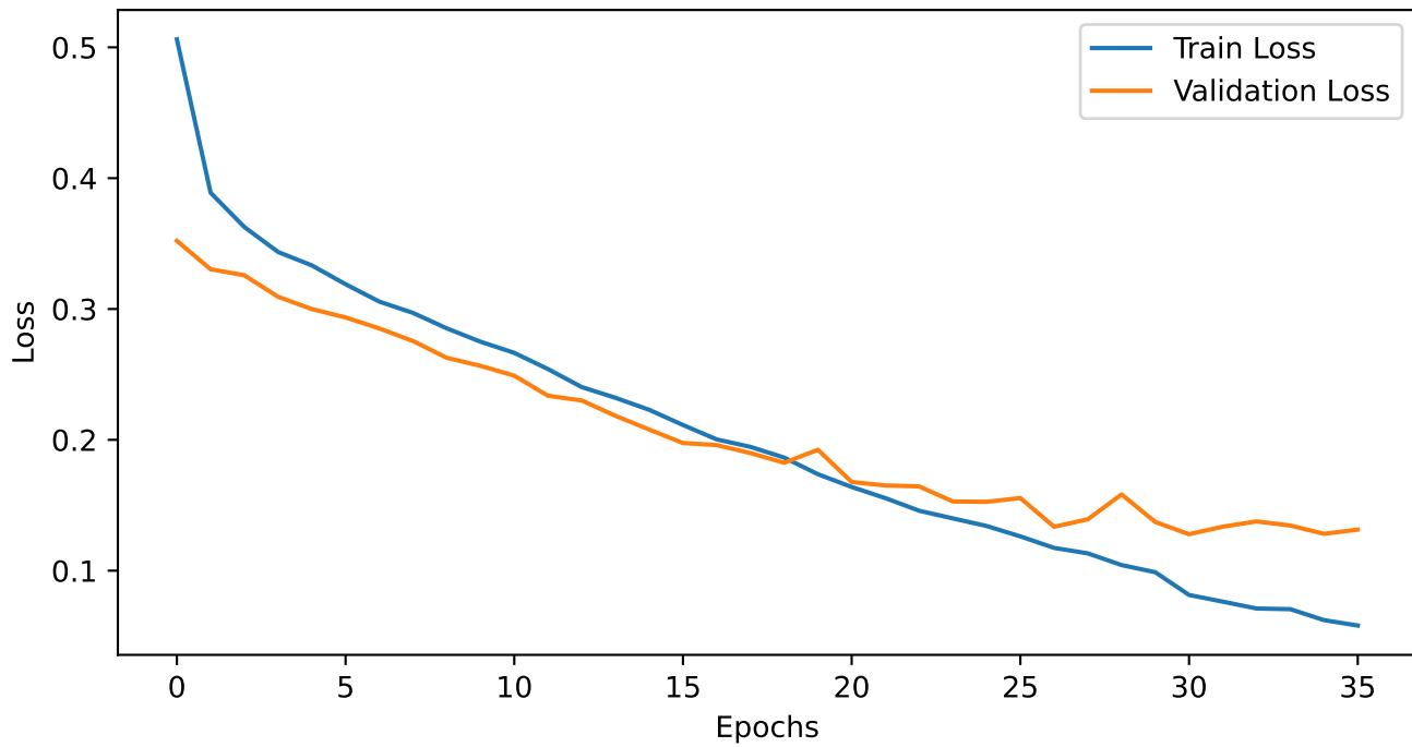
Training vs Validation Loss
