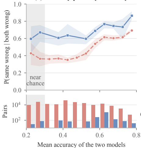
(a) Primary pairs by accuracy
