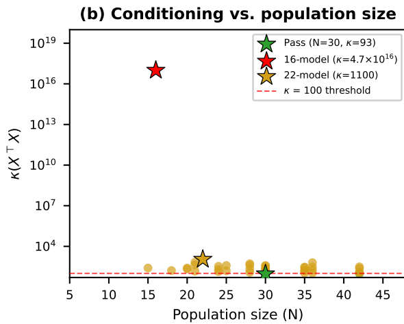
FIGURE 9: Conditioning versus population size. The condition number \kappa is shown for all full-rank designs, with the \kappa = 100 numerical-gate threshold marked. The passing design (N = 30, \kappa = 93 ) sits below the threshold; the measured 16-model population ( \kappa = 4.7 \times 10^{16} ) and the 22-model candidate ( \kappa = 1100 ) are noted as reference points.
