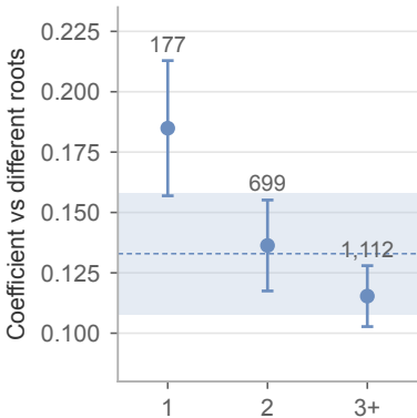
(a) Tree distance
