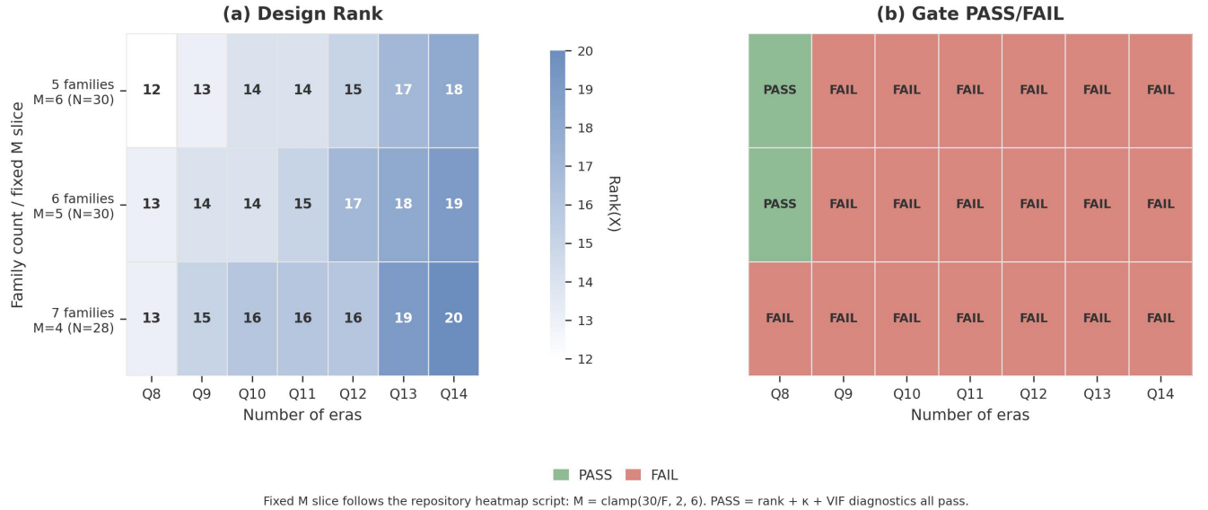
FIGURE 11: PASS/FAIL heatmap across the design space. Each cell shows whether a given (N, F, E) configuration passes all three numerical/design-matrix diagnostics: full rank, \kappa \leq 100 , and \text{VIF} \leq 10 . Crossing and connectedness are enforced by the staggered assignment constraints.
