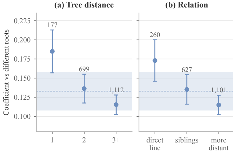
Figure 11. Lineage dose-response (primary sample; in the analysis plan, first run after review; jackknife 95% CIs; labels: pairs). Each coefficient compares one kind of related pair with different-root pairs. Tree distance: declared links through the nearest common ancestor (32 distance-zero pairs not shown). Band and dashed line: the pre-specified shared-root coefficient and interval.
