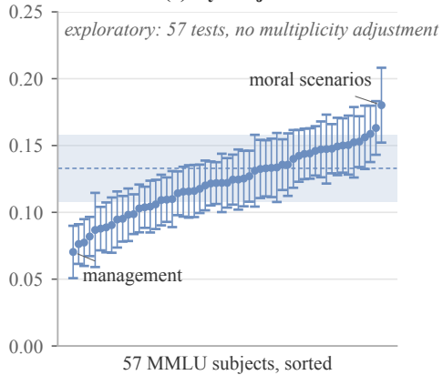
(c) By subject
