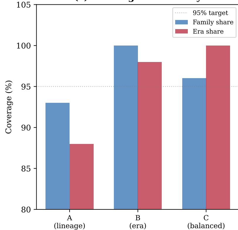
(c) Coverage Probability
